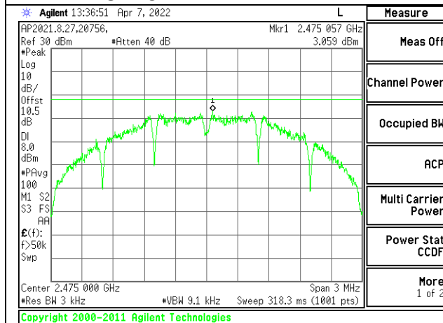
2475MHz ANTENNA 1
