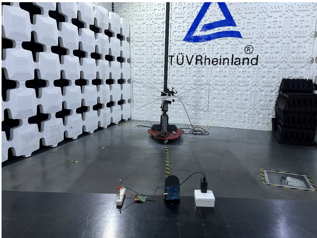
Photograph 4: Set-up for Radiated Emissions, below 1GHz
