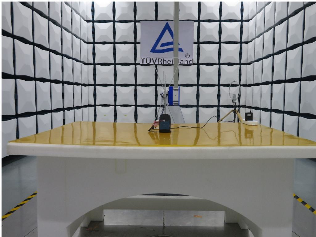
Photograph 2: Set-up for Radiated Spurious Emissions, above 30MHz
