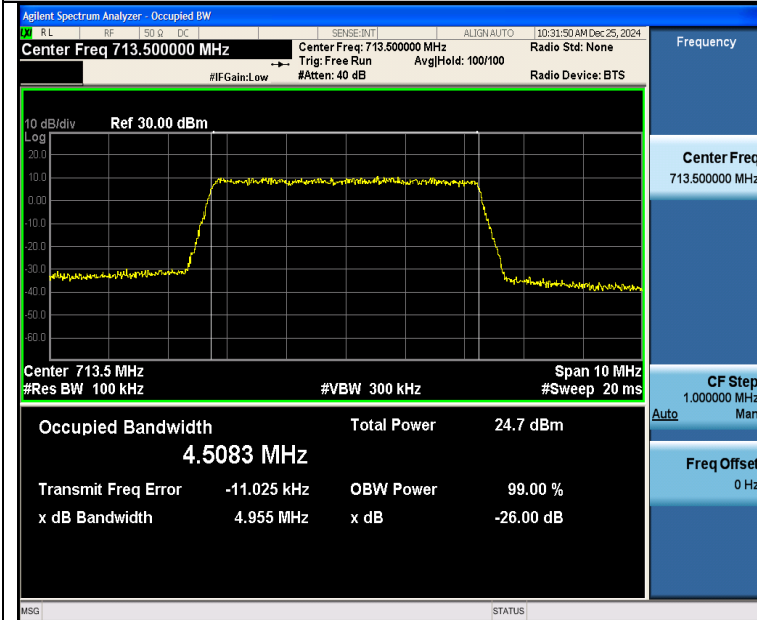
Band12-5MHz-QPSK-23155-25RB#0-PASS
