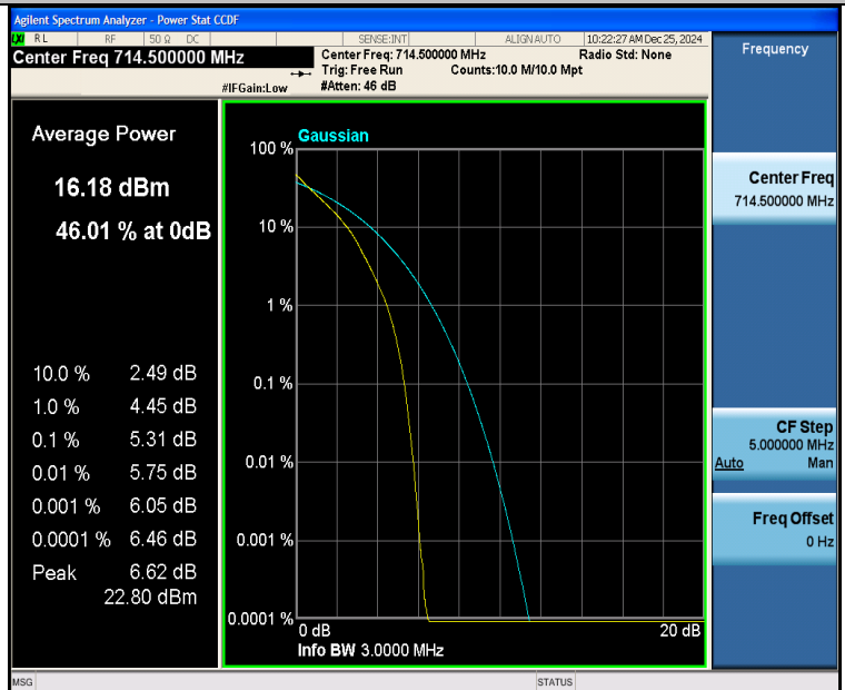
Band12-3MHz-QPSK-23165-15RB#0-PASS
