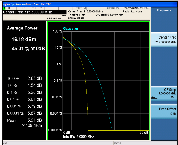
Band12-1.4MHz-QPSK-23173-6RB#0-PASS
