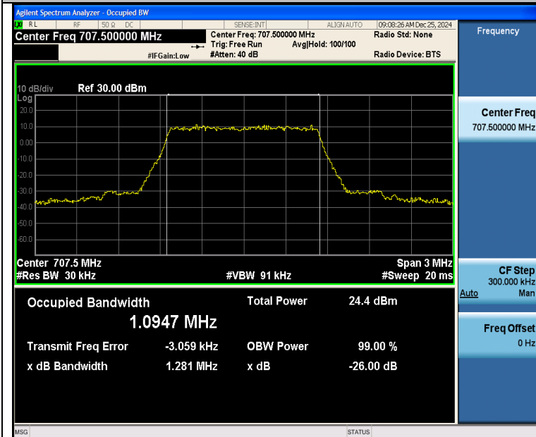
Band12-1.4MHz-QPSK-23095-6RB#0-PASS
