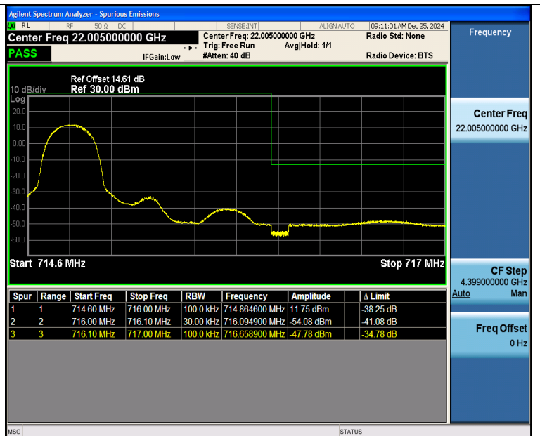
Band12 1.4MHz 16QAM 23173 1RB#0
