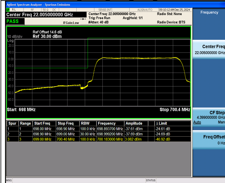
Band12 1.4MHz_QPSK_23017_6RB#0
