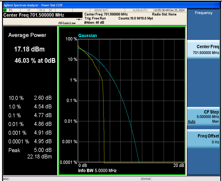
Band12-5MHz-QPSK-23035-1RB#0-PASS
