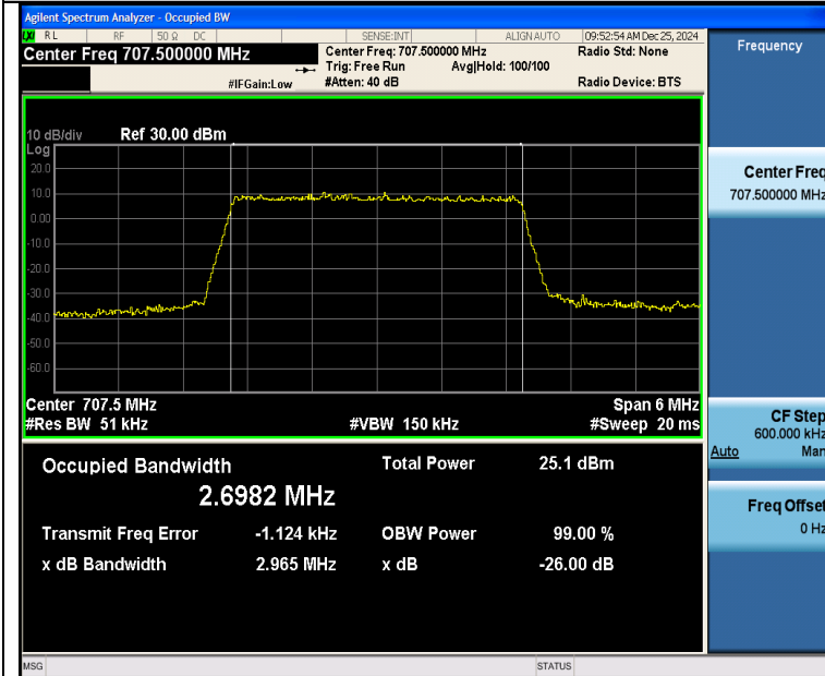
Band12-3MHz-QPSK-23095-15RB#0-PASS
