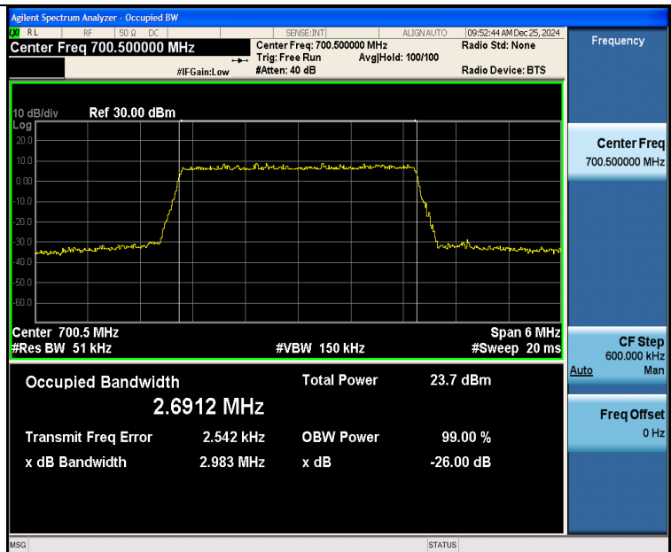
Band12-3MHz-16QAM-23025-15RB#0-PASS
