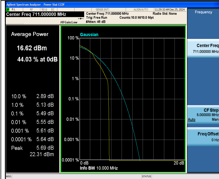
Band12-10MHz-16QAM-23130-1RB#0-PASS
