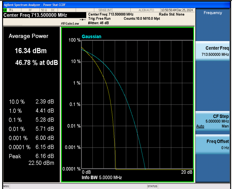
Band12-5MHz-QPSK-23155-25RB#0-PASS
