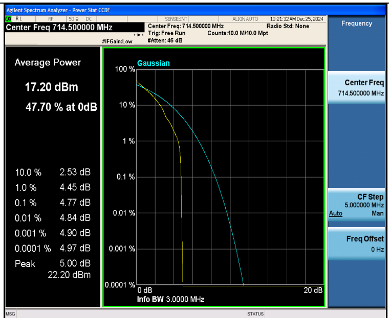
Band12-3MHz-QPSK-23165-1RB#0-PASS
