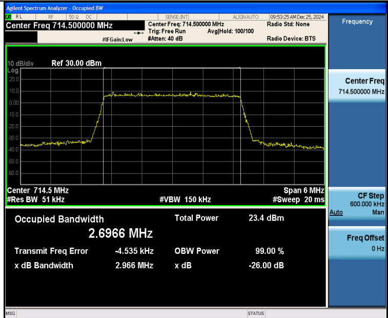
Band12-3MHz-16QAM-23165-15RB#0-PASS
