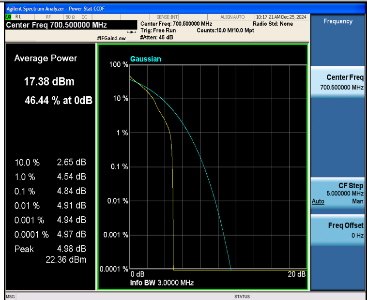
Band12-3MHz-QPSK-23025-1RB#0-PASS
