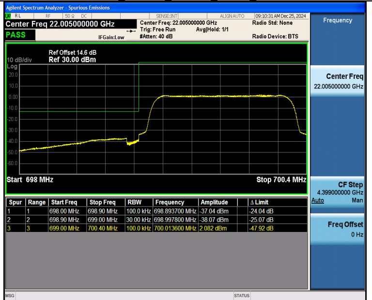
Band12 1.4MHz_16QAM_23017_6RB#0
