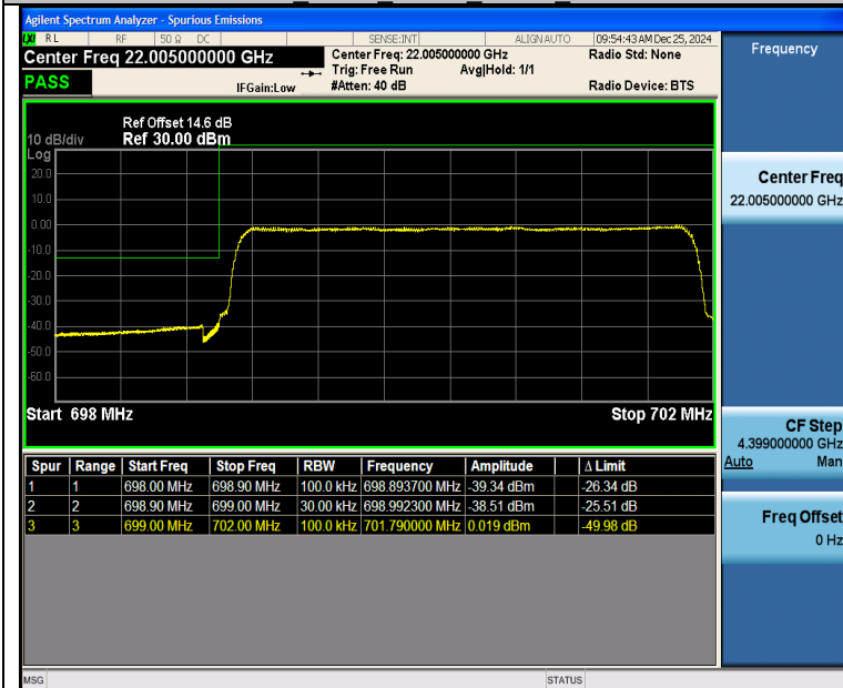
Band12_3MHz_QPSK_23025_15RB#0
