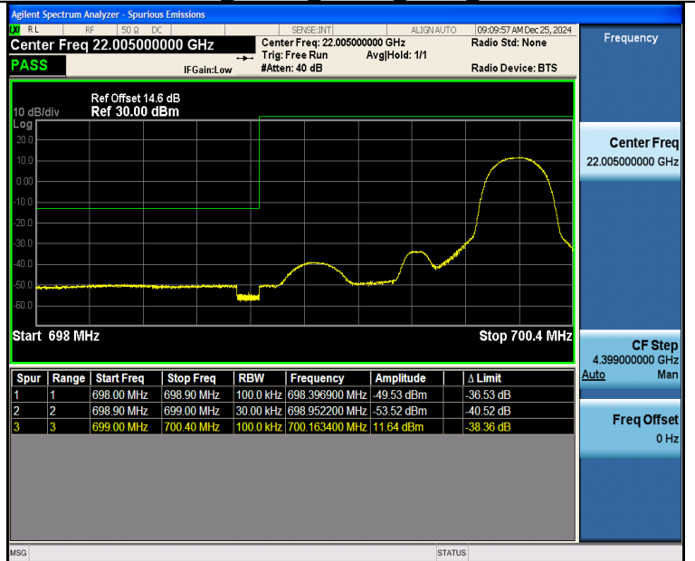
Band12 1.4MHz 16QAM 23017 1RB#5
