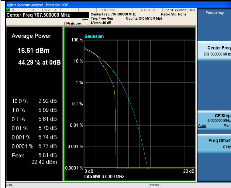
Band12-3MHz-16QAM-23095-1RB#0-PASS
