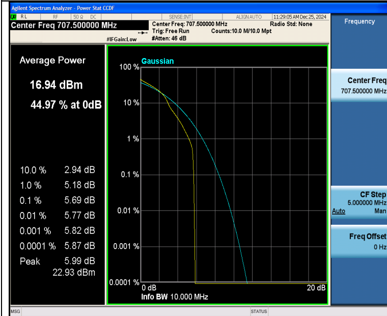
Band12-10MHz-16QAM-23095-1RB#0-PASS
