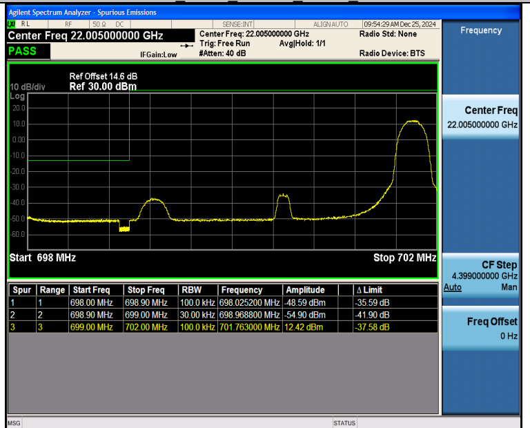
Band12 3MHz 16QAM 23025 1RB#14
