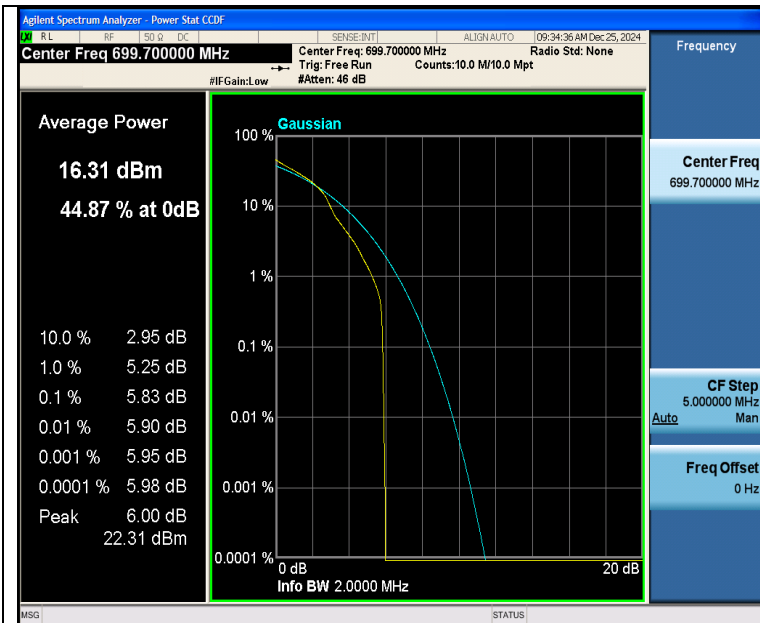
Band12-1.4MHz-16QAM-23017-1RB#0-PASS
