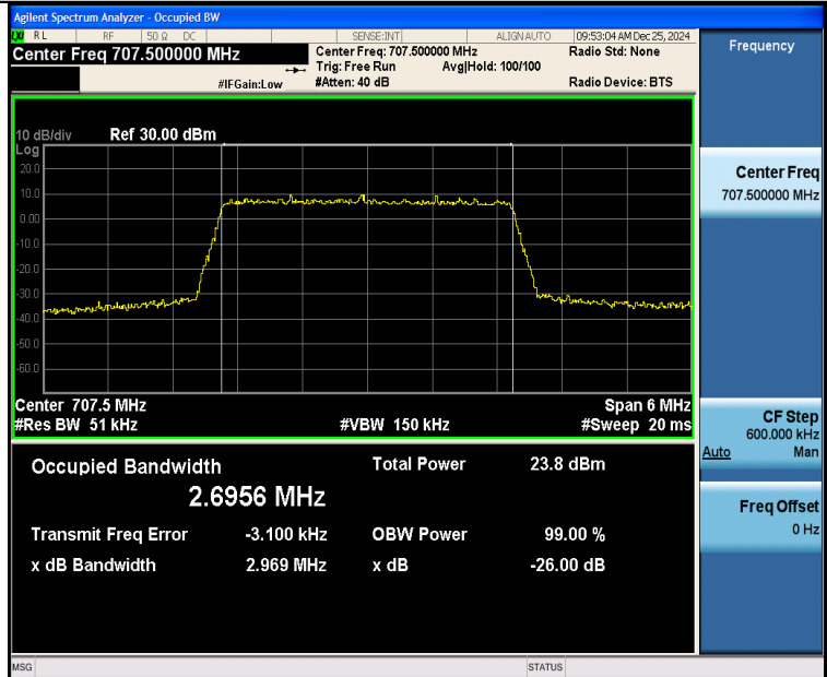
Band12-3MHz-16QAM-23095-15RB#0-PASS
