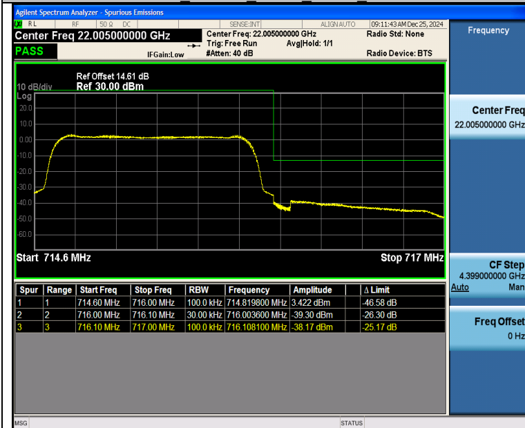
Band12 1.4MHz_QPSK_23173_6RB#0
