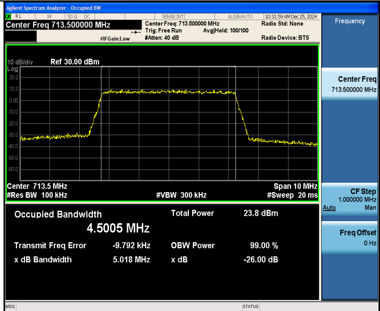
Band12-5MHz-16QAM-23155-25RB#0-PASS
