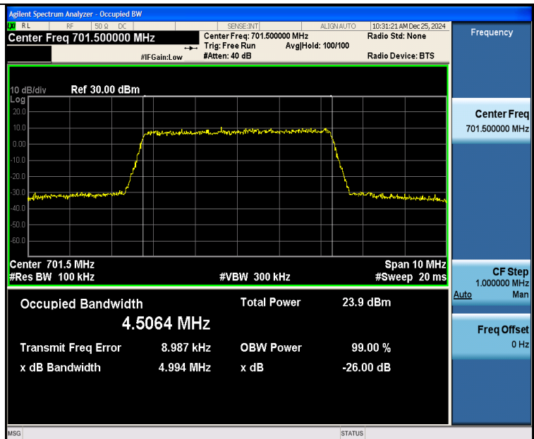
Band12-5MHz-16QAM-23035-25RB#0-PASS
