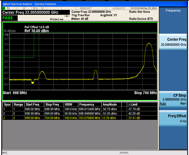
Band12 5MHz 16QAM 23035 1RB#24
