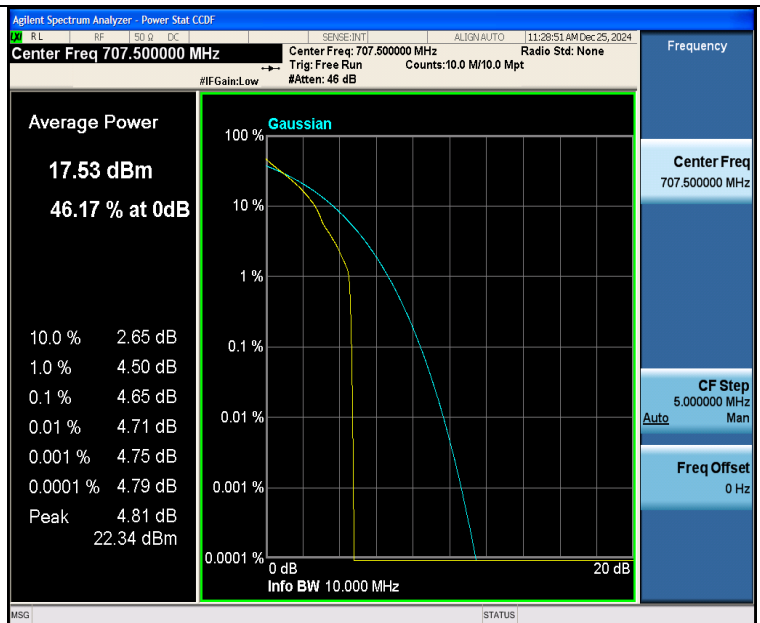
Band12-10MHz-QPSK-23095-1RB#0-PASS
