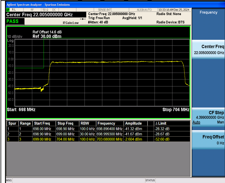
Band12_5MHz_QPSK_23035_25RB#0
