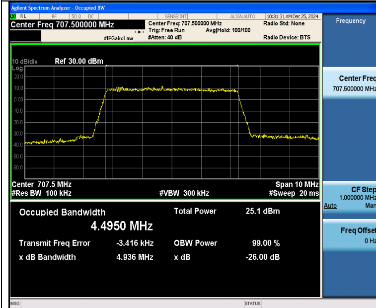
Band12-5MHz-QPSK-23095-25RB#0-PASS
