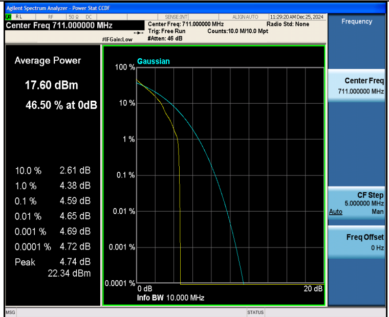
Band12-10MHz-QPSK-23130-1RB#0-PASS
