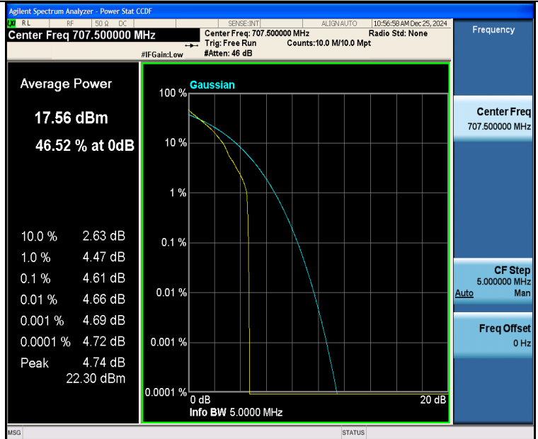
Band12-5MHz-QPSK-23095-1RB#0-PASS
