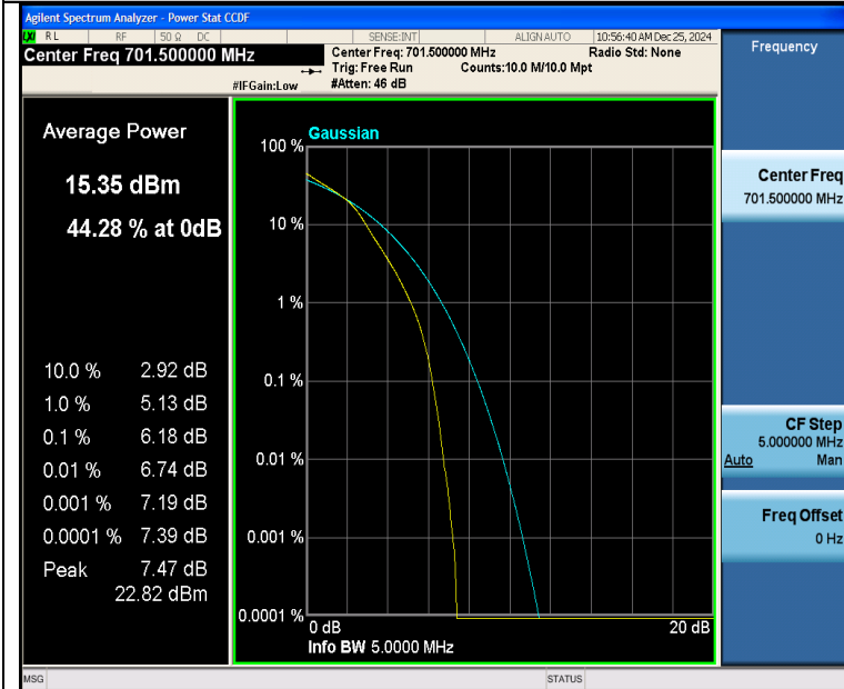
Band12-5MHz-16QAM-23035-25RB#0-PASS
