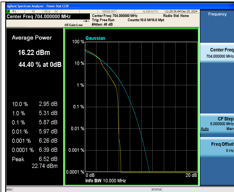
Band12-10MHz-16QAM-23060-1RB#0-PASS
