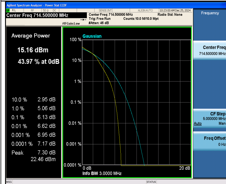
Band12-3MHz-16QAM-23165-15RB#0-PASS
