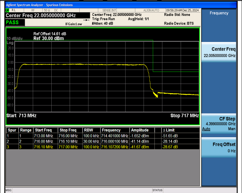
Band12_3MHz_16QAM_23165_15RB#0
