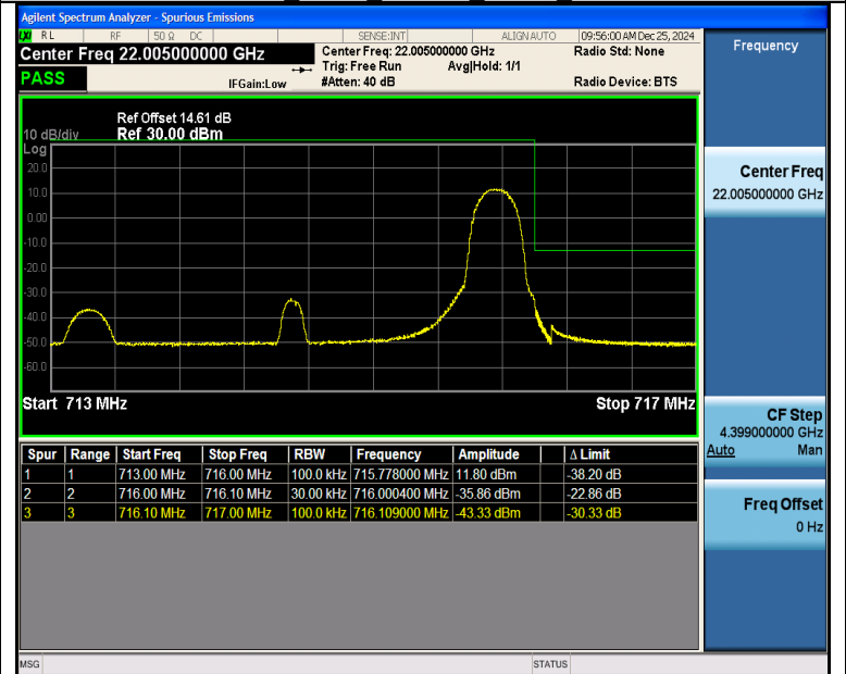
Band12 3MHz 16QAM 23165 1RB#14
