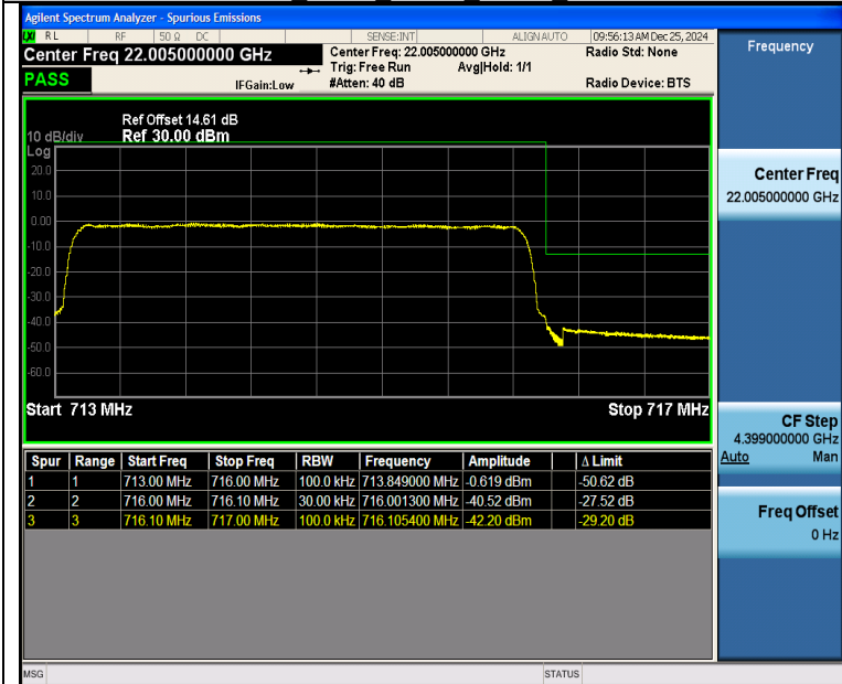
Band12_3MHz_QPSK_23165_15RB#0
