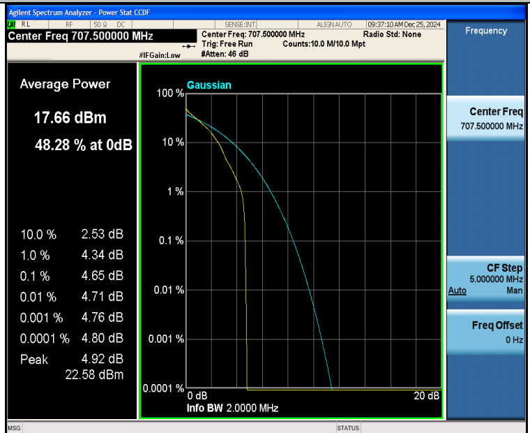
Band12-1.4MHz-QPSK-23095-1RB#0-PASS
