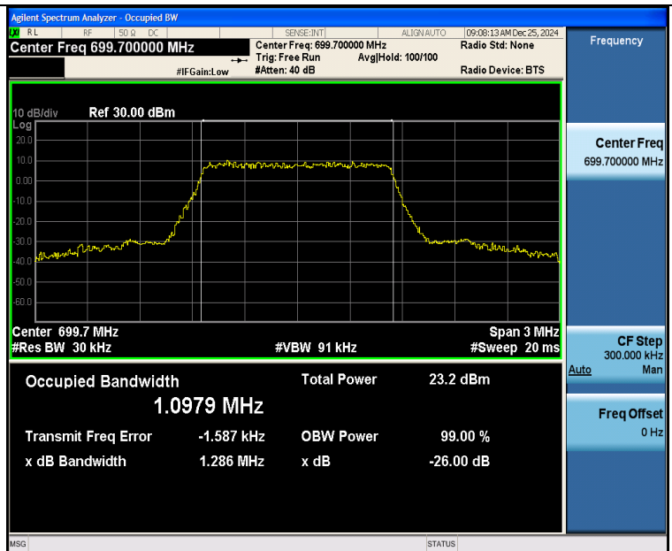
Band12-1.4MHz-16QAM-23017-6RB#0-PASS
