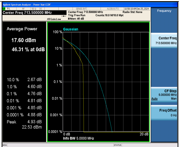
Band12-5MHz-QPSK-23155-1RB#0-PASS
