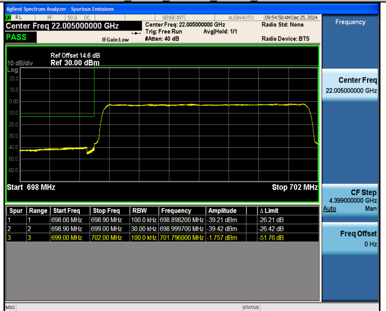
Band12_3MHz_16QAM_23025_15RB#0
