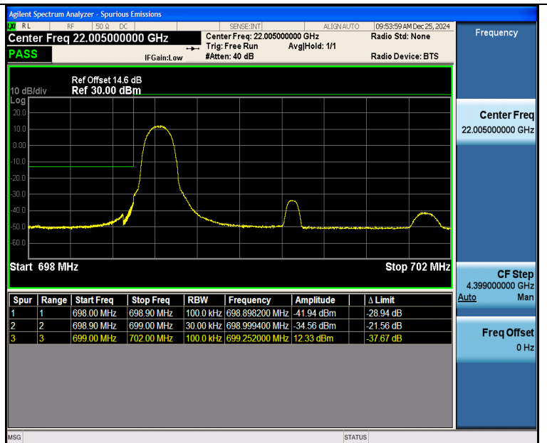
Band12 3MHz 16QAM 23025 1RB#0
