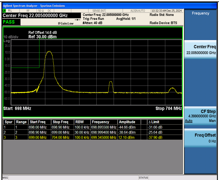
Band12 5MHz 16QAM 23035 1RB#0
