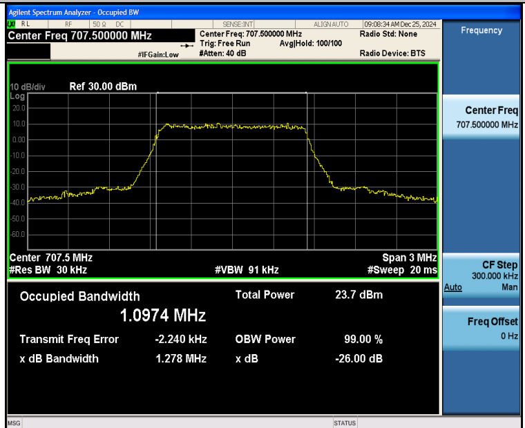
Band12-1.4MHz-16QAM-23095-6RB#0-PASS
