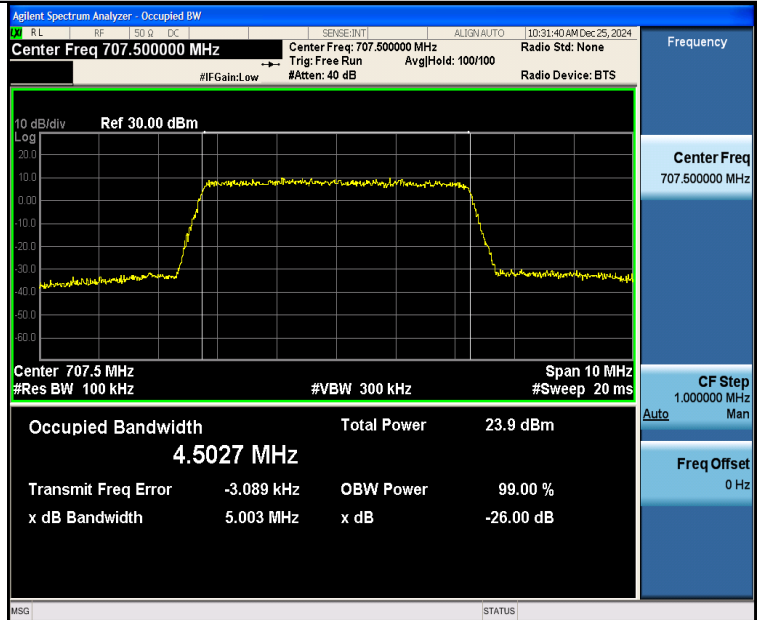
Band12-5MHz-16QAM-23095-25RB#0-PASS
