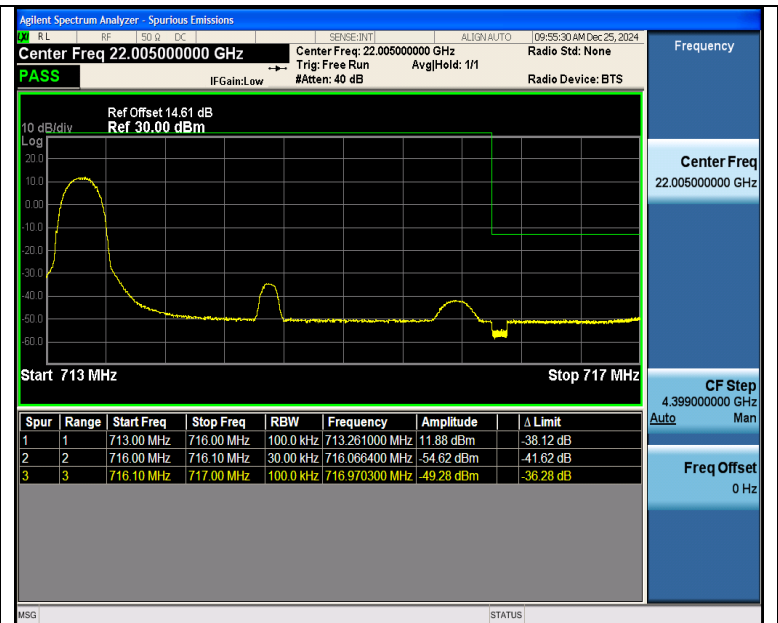
Band12 3MHz 16QAM 23165 1RB#0
