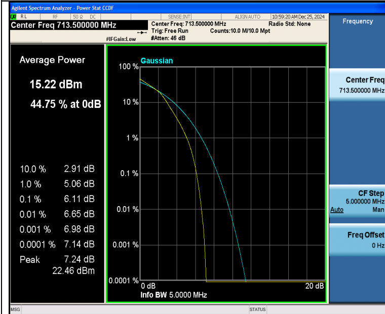
Band12-5MHz-16QAM-23155-25RB#0-PASS
