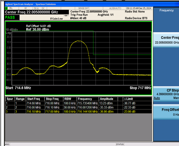
Band12 1.4MHz QPSK 23173 1RB#5
