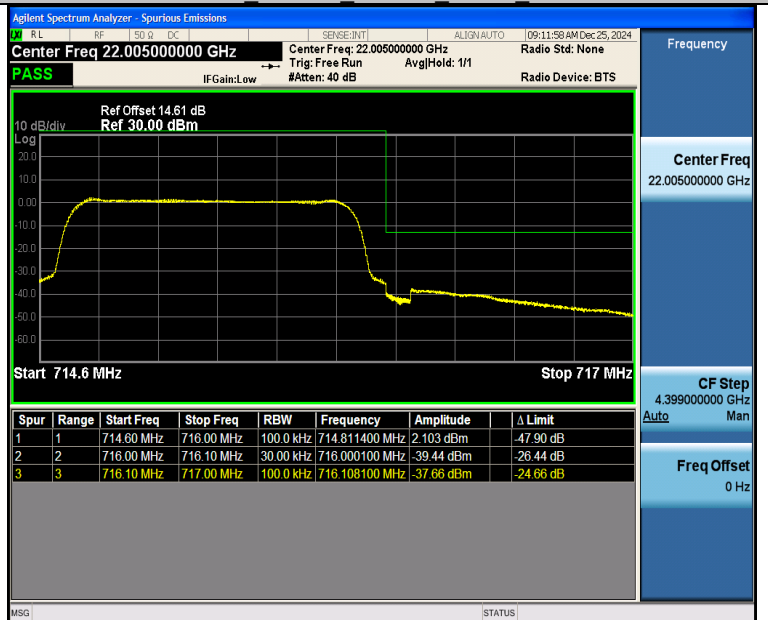
Band12 1.4MHz_16QAM_23173_6RB#0
