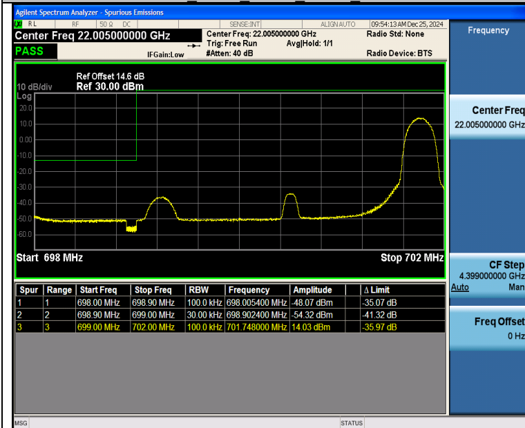
Band12 3MHz QPSK 23025 1RB#14
