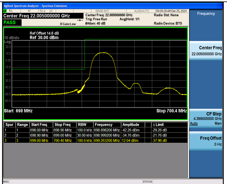
Band12 1.4MHz 16QAM 23017 1RB#0
