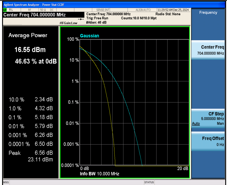
Band12-10MHz-QPSK-23060-50RB#0-PASS
