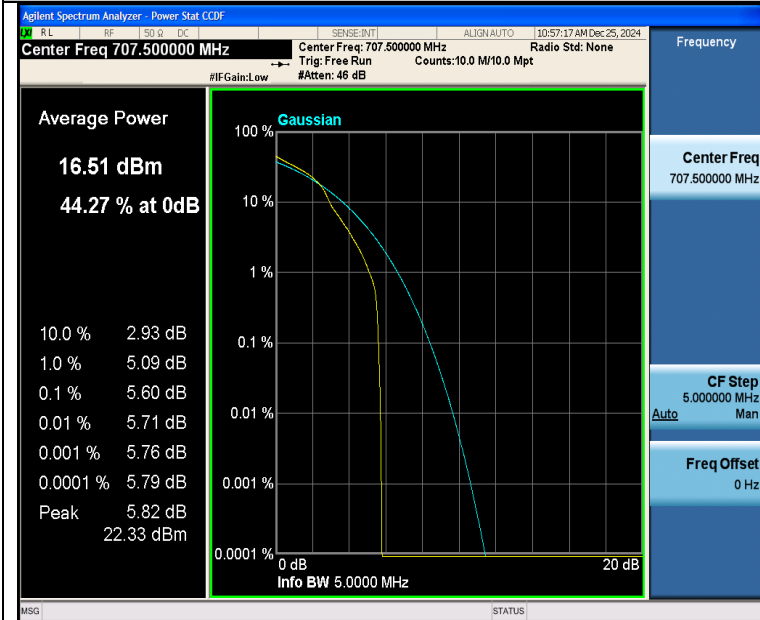
Band12-5MHz-16QAM-23095-1RB#0-PASS
