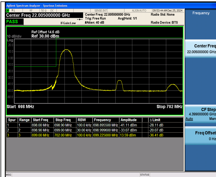
Band12 3MHz QPSK 23025 1RB#0
