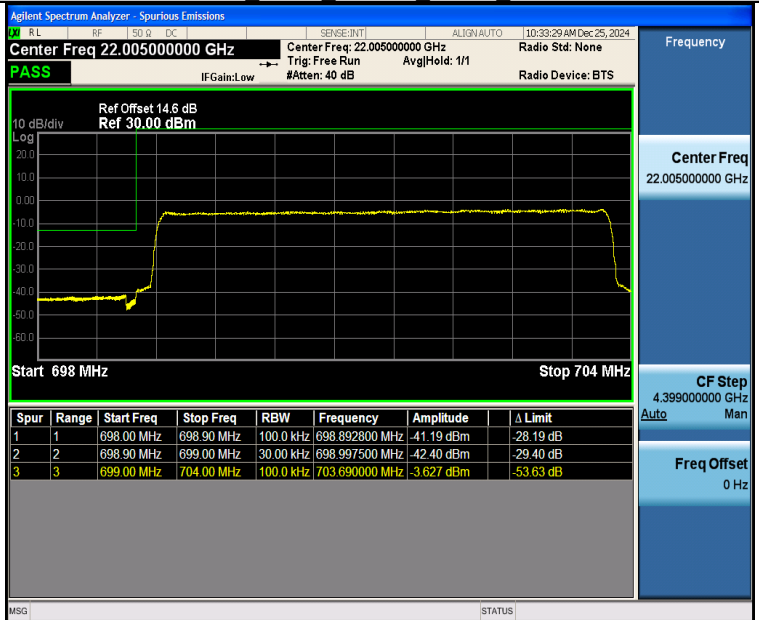
Band12_5MHz_16QAM_23035_25RB#0
