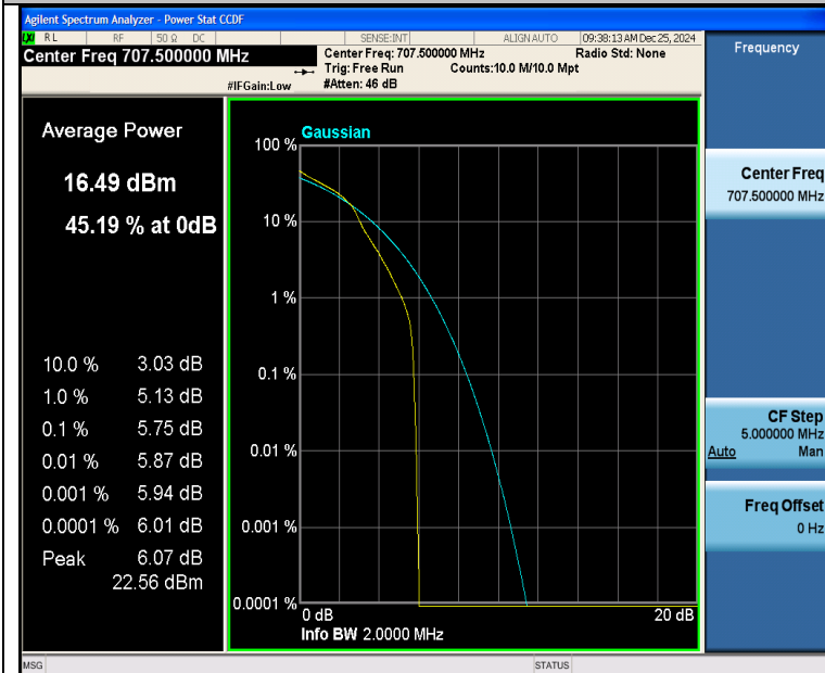
Band12-1.4MHz-16QAM-23095-1RB#0-PASS
