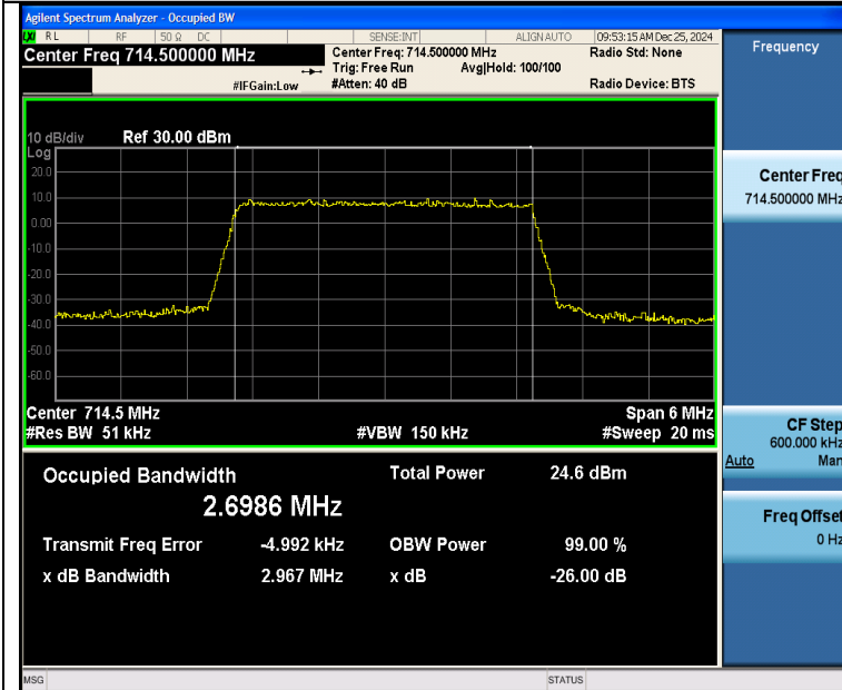
Band12-3MHz-QPSK-23165-15RB#0-PASS
