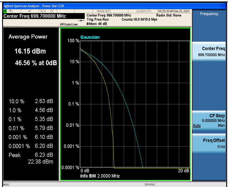
Band12-1.4MHz-QPSK-23017-6RB#0-PASS
