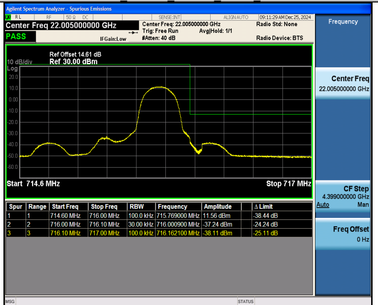
Band12 1.4MHz 16QAM 23173 1RB#5
