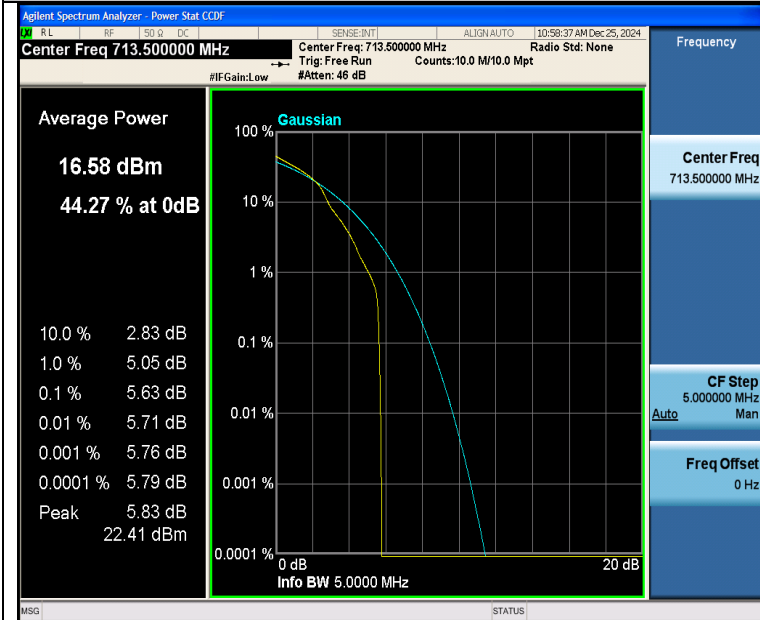
Band12-5MHz-16QAM-23155-1RB#0-PASS
