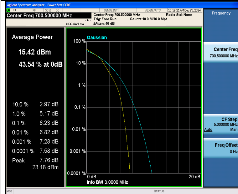
Band12-3MHz-16QAM-23025-15RB#0-PASS
