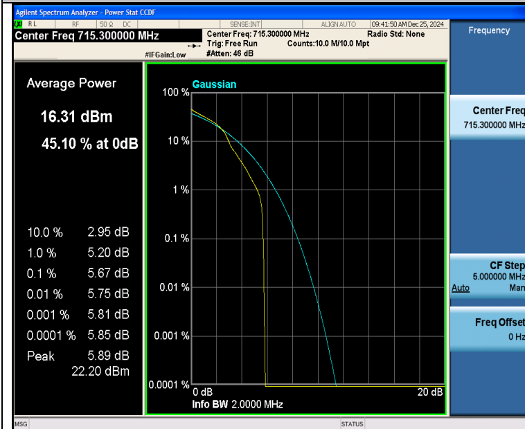
Band12-1.4MHz-16QAM-23173-1RB#0-PASS
