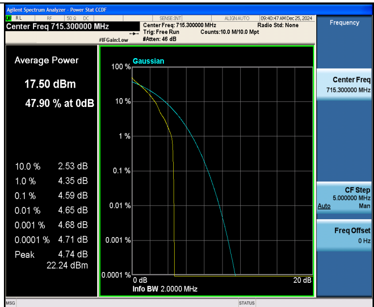
Band12-1.4MHz-QPSK-23173-1RB#0-PASS
