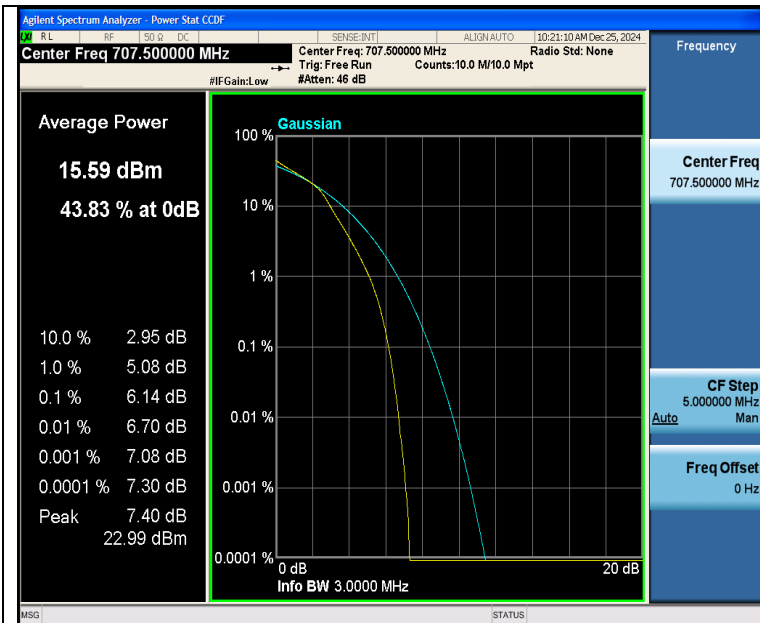
Band12-3MHz-16QAM-23095-15RB#0-PASS
