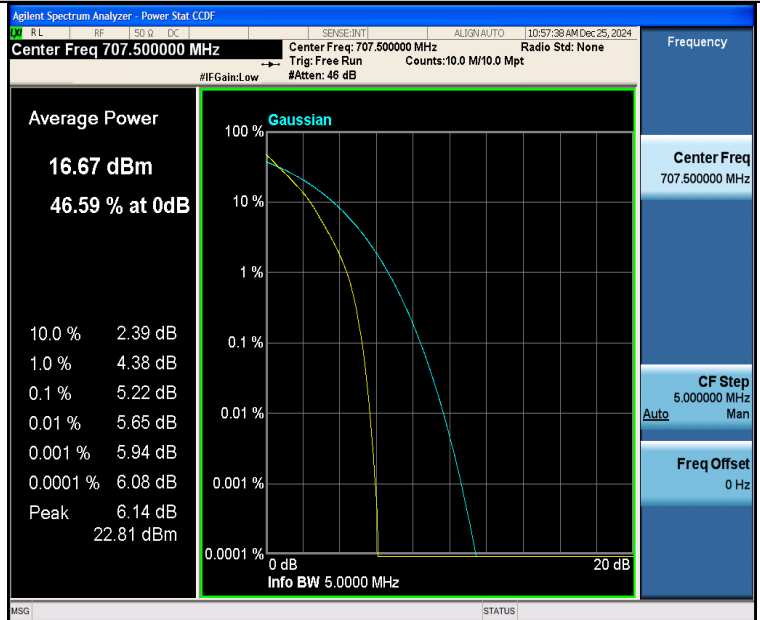
Band12-5MHz-QPSK-23095-25RB#0-PASS
