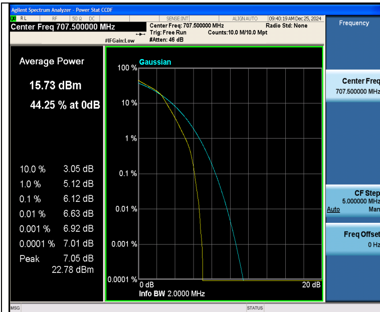
Band12-1.4MHz-16QAM-23095-6RB#0-PASS
