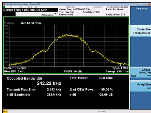
(Plot B1: GPRS 1900MHz Channel = 512 Occupied bandwidth)
