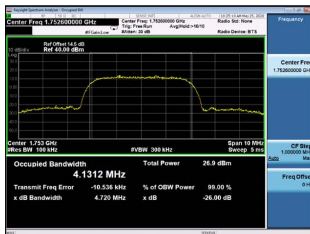
(Plot G3: WCDMA 1700 MHz Channel = 1513 bandwidth)
