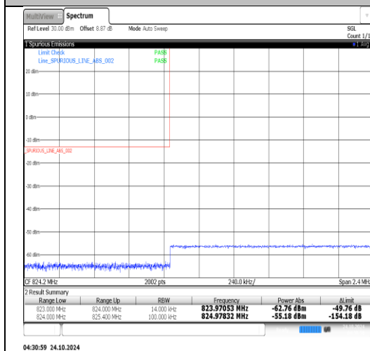
Band26(824-849)-1.4MHz-16QAM-26797-1RB#5-PASS
