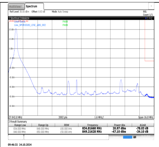
Band26(824-849)-15MHz-QPSK-26965-1RB#74-PASS
