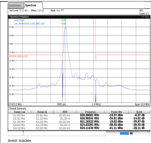
Band26(814-824)-3MHz-16QAM-26775- 1RB#14-PASS
