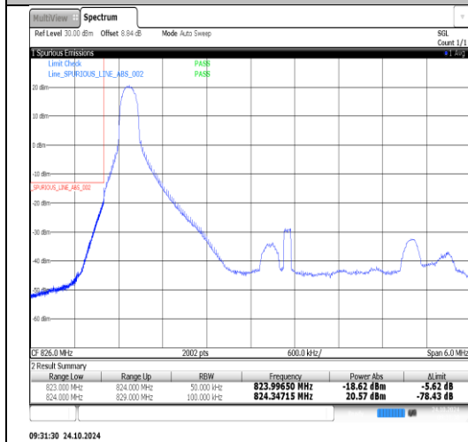
Band26(824-849)-5MHz-QPSK-26815-1RB#24-PASS
