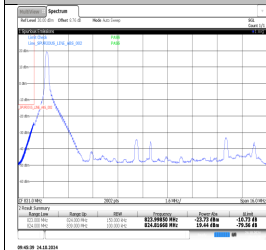
Band26(824-849)-15MHz-16QAM-26865-1RB#74-PASS
