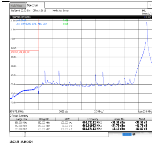
Band71-20MHz-16QAM-133372-100RB#0-PASS
