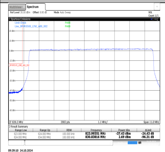
Band26(824-849)-10MHz-16QAM-26990- 1RB#0-PASS
