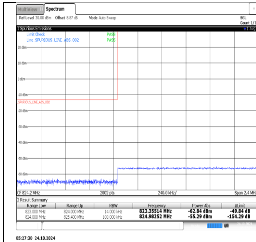
Band26(824-849)-1.4MHz-QPSK-27033-6RB#0-PASS
