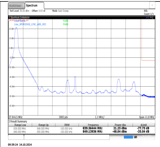
Band26(824-849)-10MHz-QPSK-26990-1RB#49- PASS
