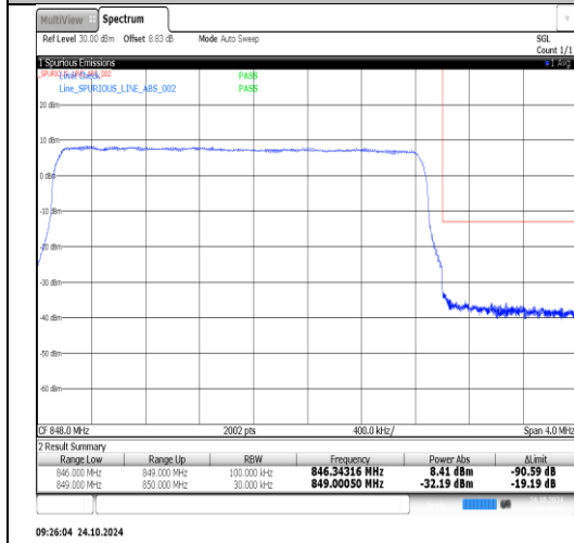
Band26(824-849)-5MHz-QPSK-26815-1RB#0-PASS
