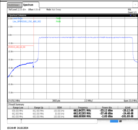
Band71-20MHz-16QAM-133372-1RB#0-PASS
