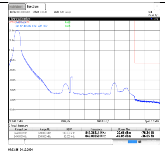
Band26(824-849)-5MHz-16QAM-27015-1RB#24-PASS
