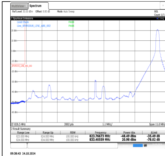
Band26(824-849)-10MHz-QPSK-26990-50RB#0- PASS
