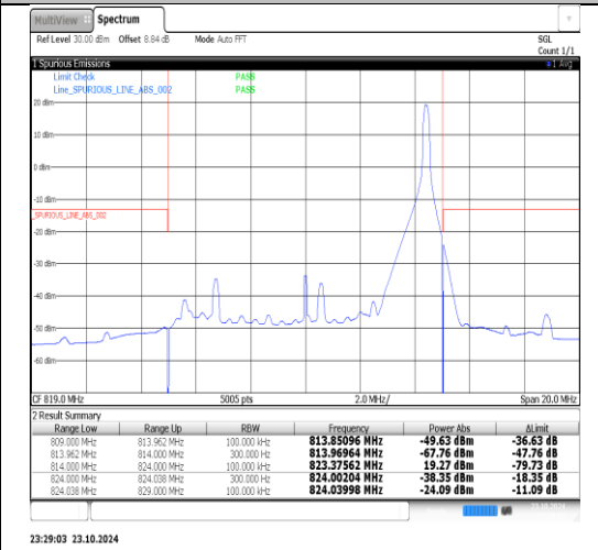
Band26(824-849)-1.4MHz-QPSK-26797-6RB#0-PASS
