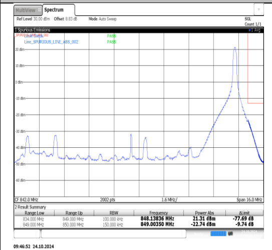
Band26(824-849)-15MHz-16QAM-26865-75RB#0-PASS
