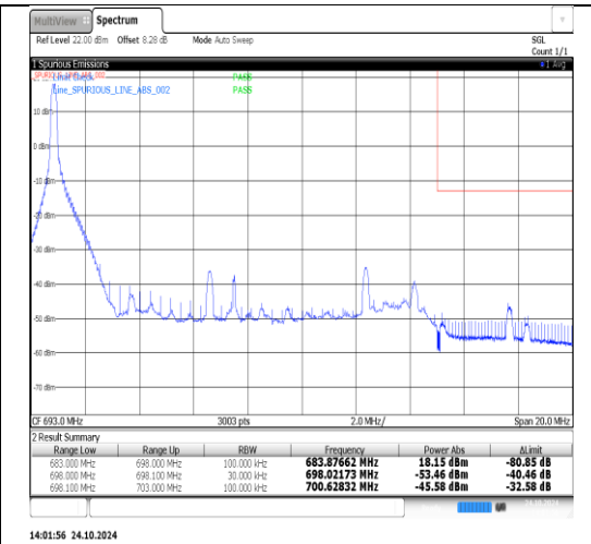
Band71-15MHz-16QAM-133397-1RB#74-PASS
