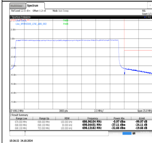
Band71-20MHz-16QAM-133222-1RB#0-PASS
