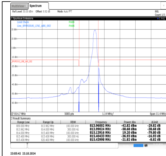
Band26(814-824)-1.4MHz-QPSK-26783-6RB#0-PASS
