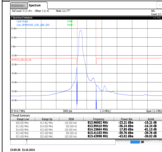
Band26(814-824)-1.4MHz-16QAM-26697-1RB#5-PASS
