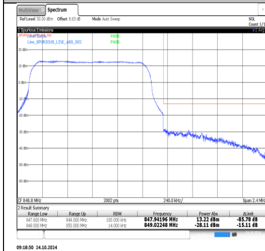
Band26(824-849)-1.4MHz-16QAM-26797-1RB#0-PASS
