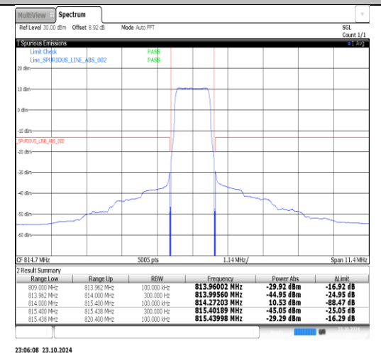
Band26(814-824)-1.4MHz-QPSK-26783-1RB#0-PASS
