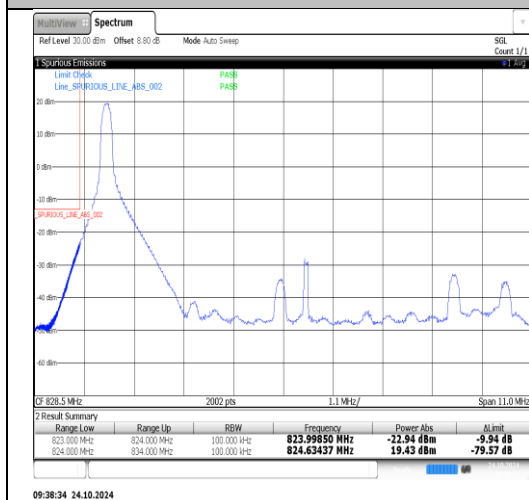
Band26(824-849)-10MHz-16QAM-26840- 1RB#49-PASS
