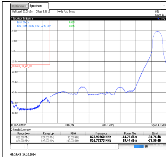
Band26(824-849)-3MHz-16QAM-27025-15RB#0-PASS
