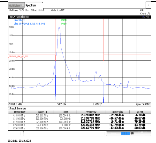
Band26(814-824)-5MHz-QPSK-26765-1RB#24- PASS
