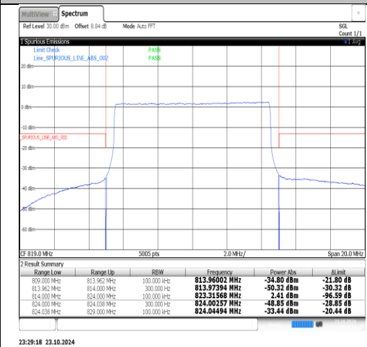
Band26(814-824)-10MHz-16QAM-26740- 1RB#0-PASS
