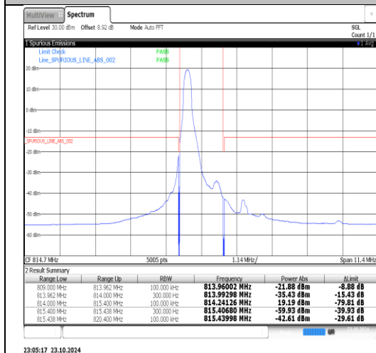
Band26(814-824)-1.4MHz-QPSK-26697-1RB#5-PASS
