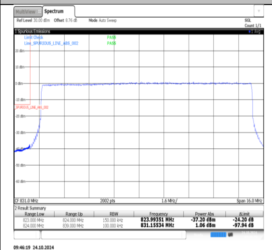
Band26(824-849)-15MHz-16QAM-26965-1RB#0-PASS
