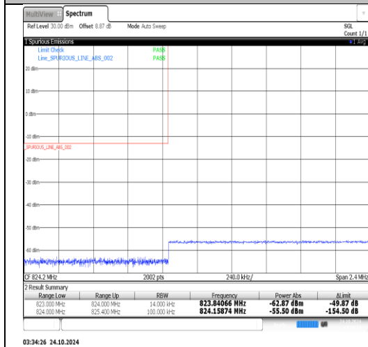
Band26(824-849)-1.4MHz-QPSK-26797-1RB#5-PASS
