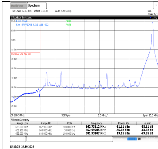
Band71-20MHz-QPSK-133372-100RB#0-PASS
