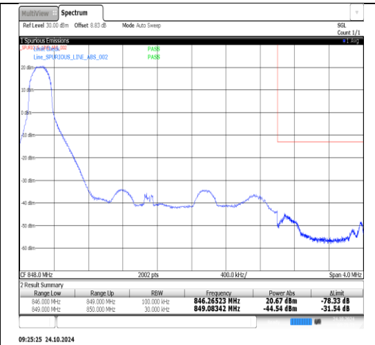
Band26(824-849)-3MHz-16QAM-27025-1RB#14-PASS
