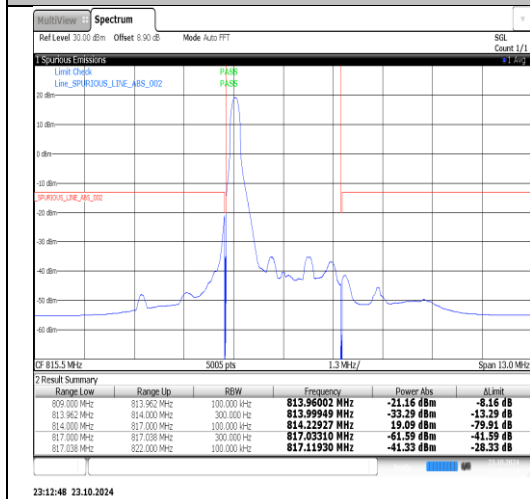
Band26(814-824)-3MHz-QPSK-26705-1RB#14-PASS
