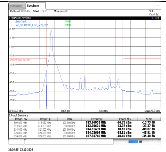
Band26(814-824)-10MHz-16QAM-26740-1RB#49-PASS
