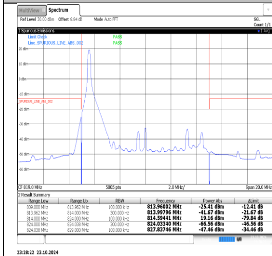
Band26(814-824)-10MHz-QPSK-26740-1RB#49- PASS
