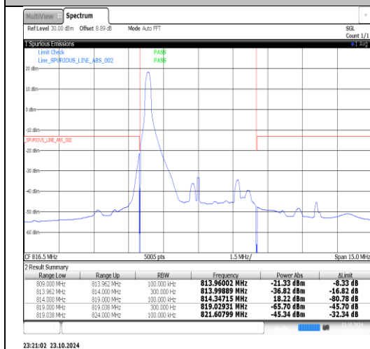
Band26(814-824)-5MHz-16QAM-26715- 1RB#24-PASS
