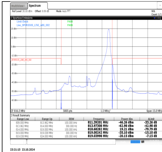
Band26(814-824)-5MHz-QPSK-26765-25RB#0- PASS
