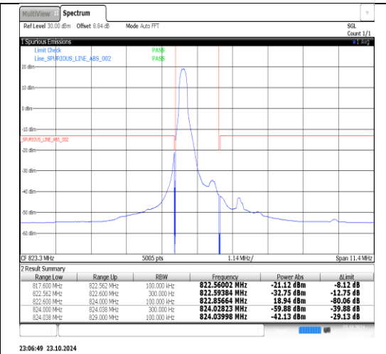
Band26(814-824)-1.4MHz-16QAM-26783-1RB#5-PASS
