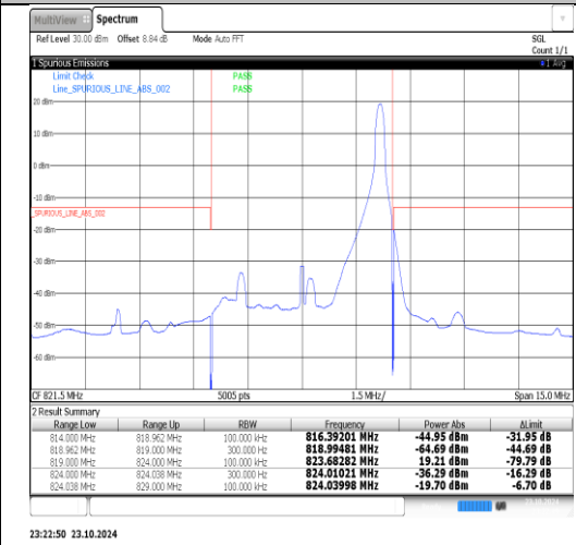
Band26(814-824)-10MHz-QPSK-26740-50RB#0- PASS
