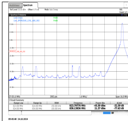
Band26(824-849)-15MHz-QPSK-26965-75RB#0-PASS
