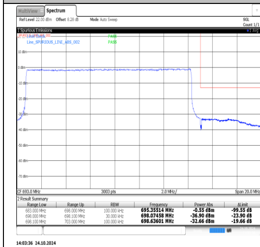
Band71-20MHz-QPSK-133222-1RB#0-PASS
