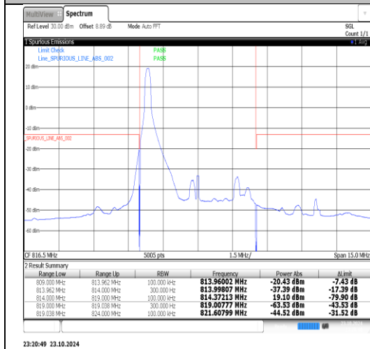
Band26(814-824)-5MHz-QPSK-26715-1RB#24- PASS
