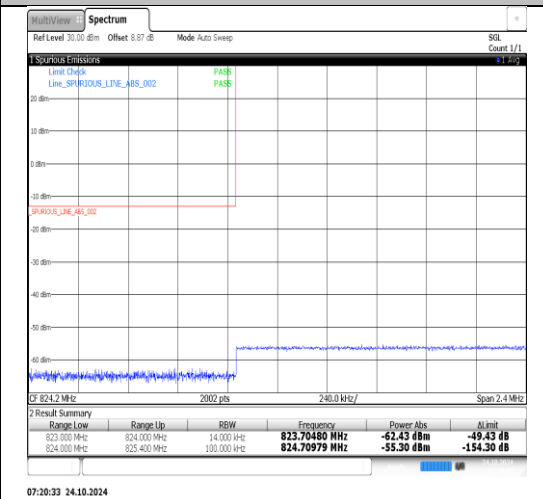
Band26(824-849)-1.4MHz-QPSK-27033-1RB#0-PASS
