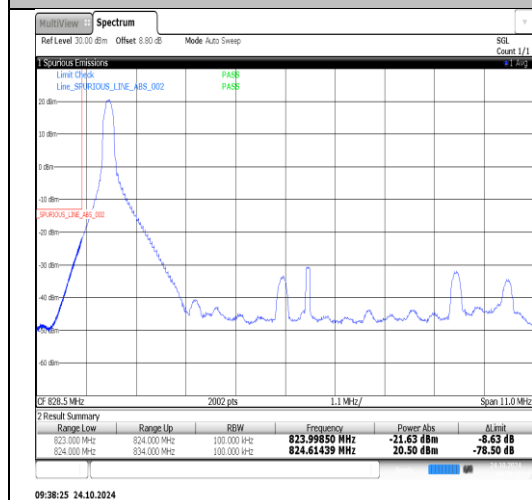
Band26(824-849)-10MHz-QPSK-26840-1RB#49-PASS
