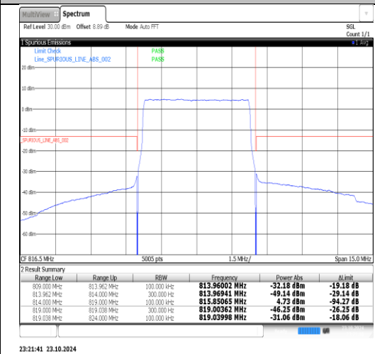
Band26(814-824)-5MHz-QPSK-26765-1RB#0- PASS
