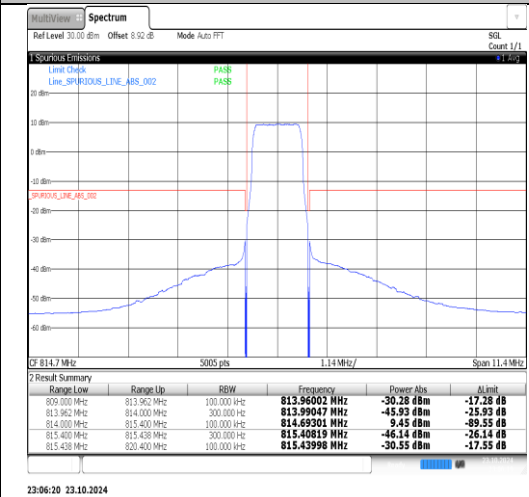
Band26(814-824)-1.4MHz-16QAM-26783-1RB#0-PASS
