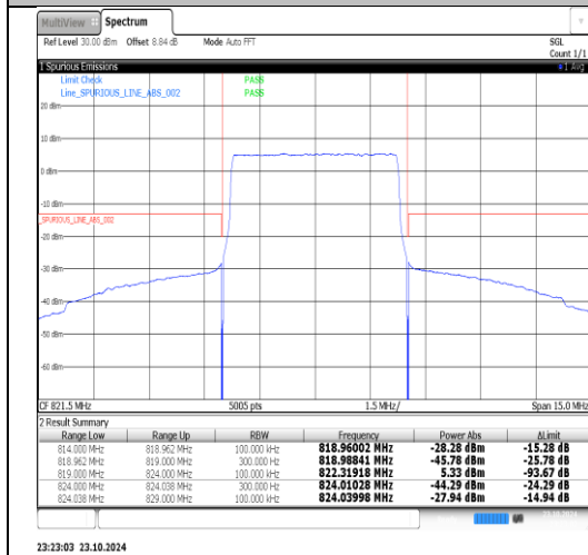
Band26(814-824)-5MHz-16QAM-26715-1RB#0- PASS
