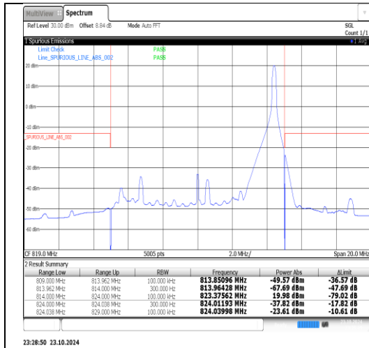
Band26(814-824)-10MHz-16QAM-26740-50RB#0-PASS
