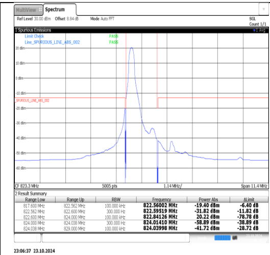
Band26(814-824)-1.4MHz-QPSK-26783-1RB#5-PASS
