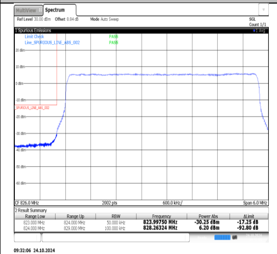
Band26(824-849)-5MHz-QPSK-27015-1RB#0-PASS
