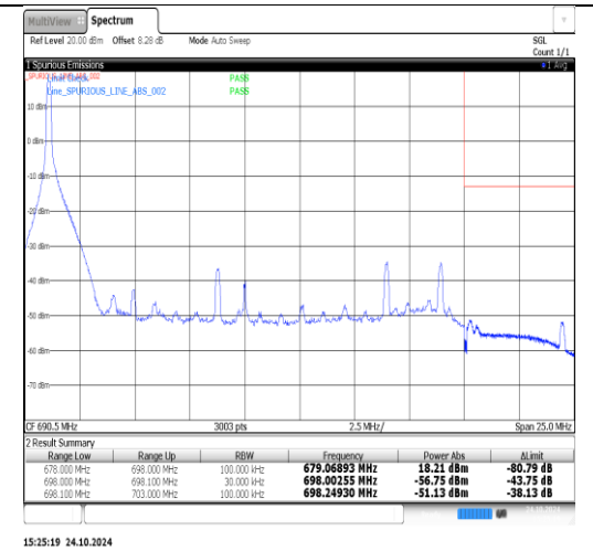
Band71-20MHz-16QAM-133372-1RB#99-PASS
