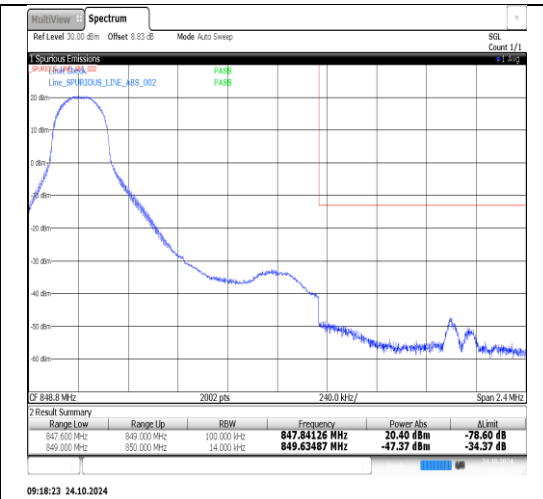
Band26(824-849)-1.4MHz-16QAM-27033-1RB#5-PASS
