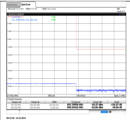
Band26(824-849)-1.4MHz-QPSK-27033-1RB#5-PASS
