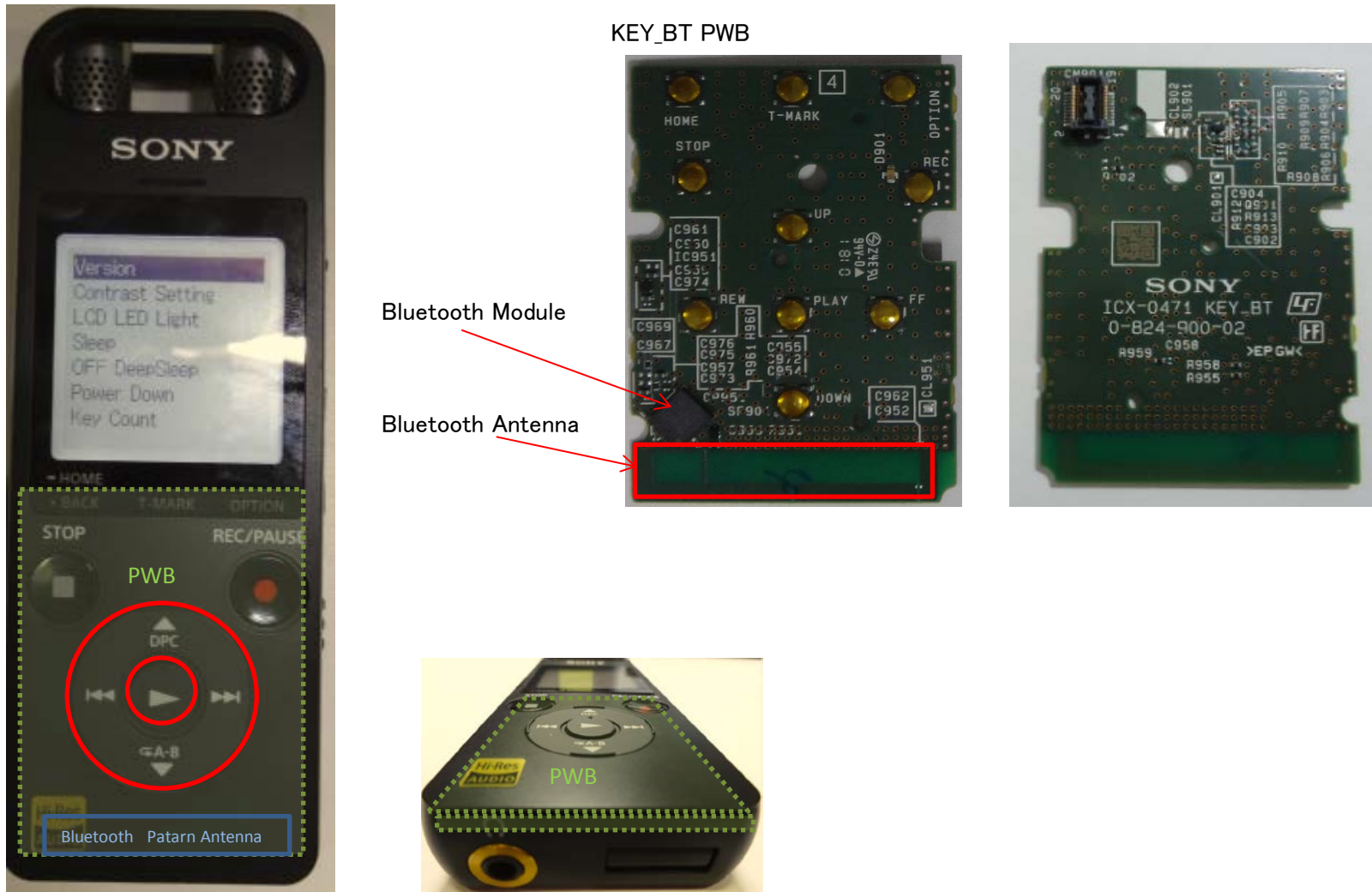
Bluetooth Antenna&device position
