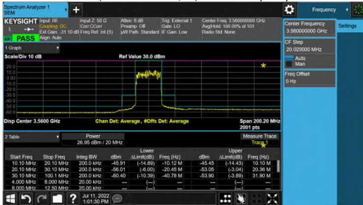
Test Model 3.1, Modulation 64QAM, Channel Frequency 3560 MHz
