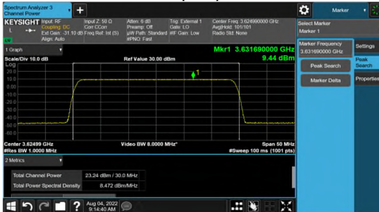
30MHz BW, TM1.1 Channel Frequency 3625MHz
