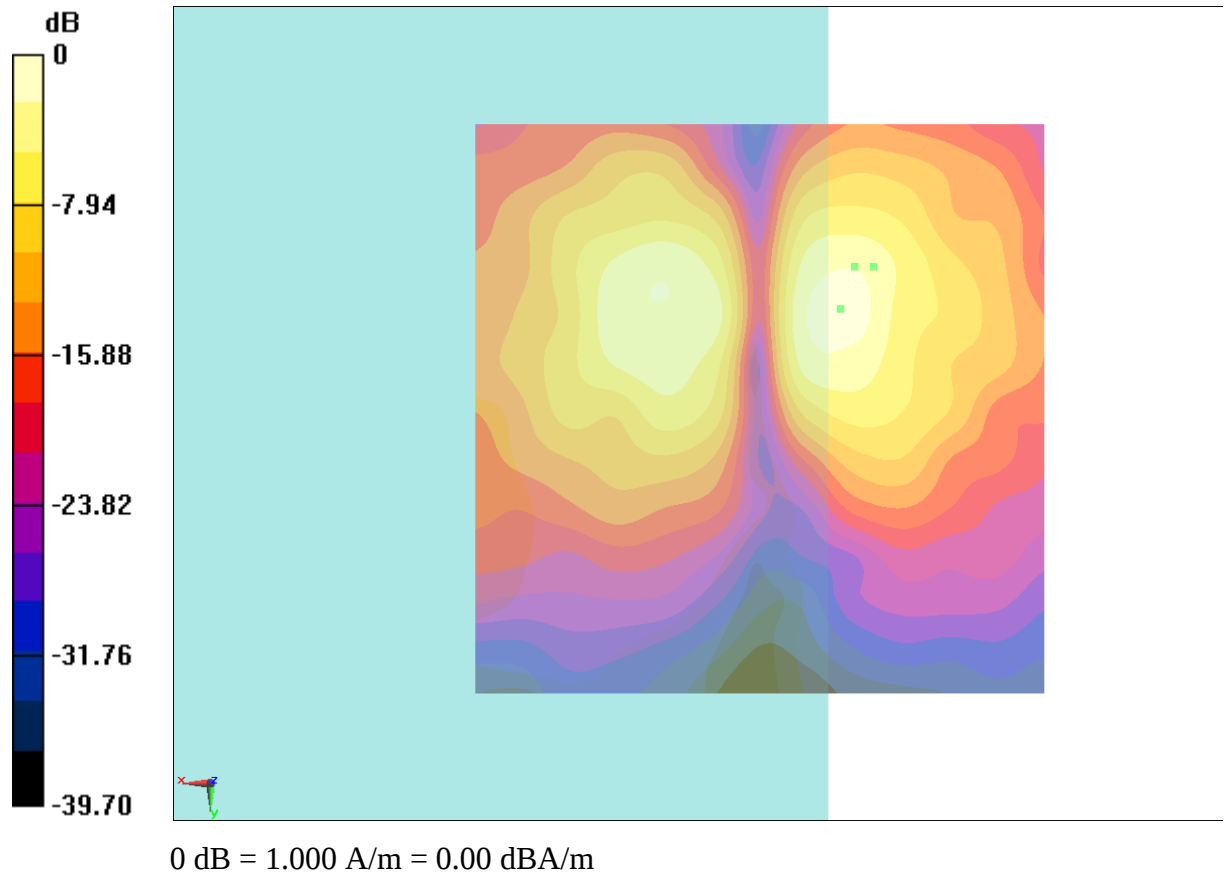
Fig B.12 T-Coil CDMA 1880_Channel 25
