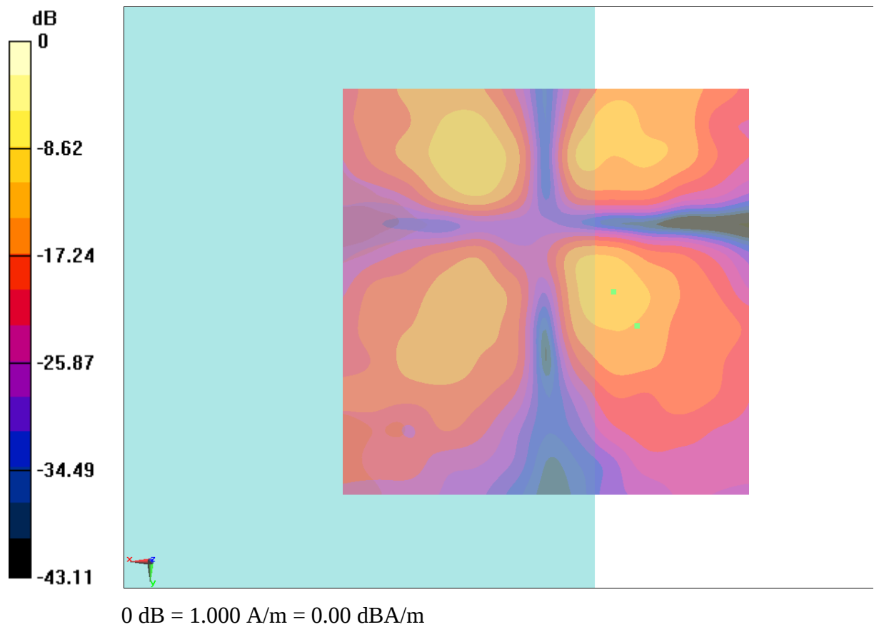
Fig B.9 T-Coil CDMA 1880_Channel 600
