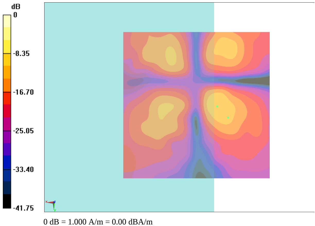
Fig B.11 T-Coil CDMA 1880_Channel 25
