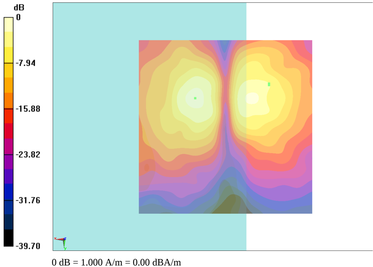
Fig B.10 T-Coil CDMA 1880_Channel 600
