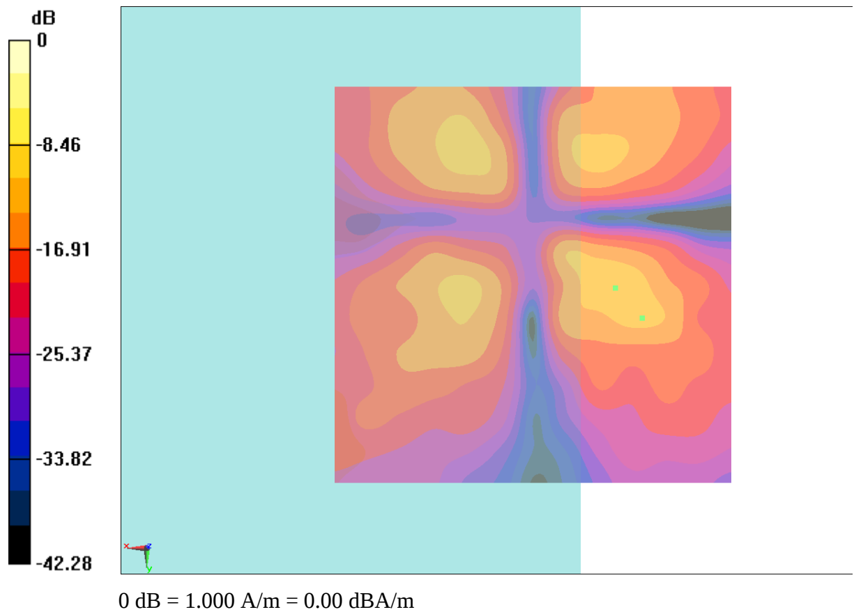
Fig B.7 T-Coil CDMA 1880_Channel 1175
