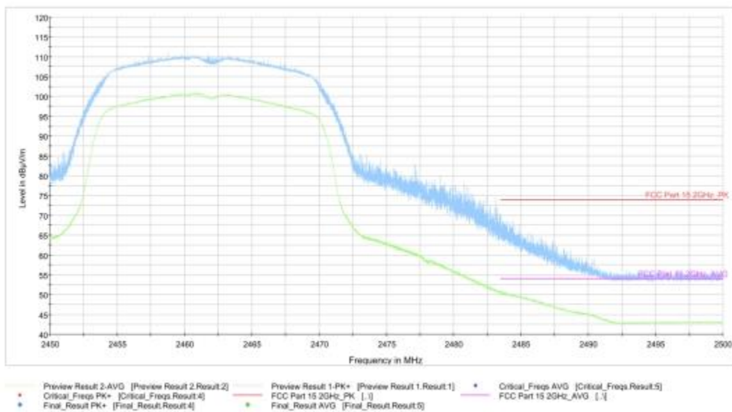
Fig.A.6.2.4 Transmitter Spurious Emission - Radiated (Power): 802.11g, ch11, 2.45 GHz - 2.50GHz
