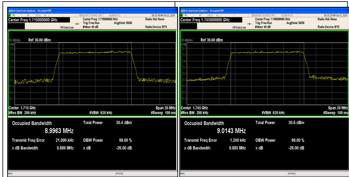
Band66-10MHz-64QAM-132022-50RB#0-PASS
