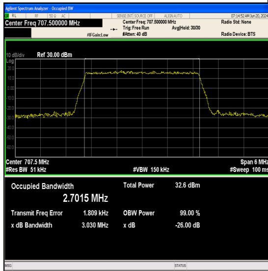
Band12-3MHz-QPSK-23095-15RB#0-PASS
