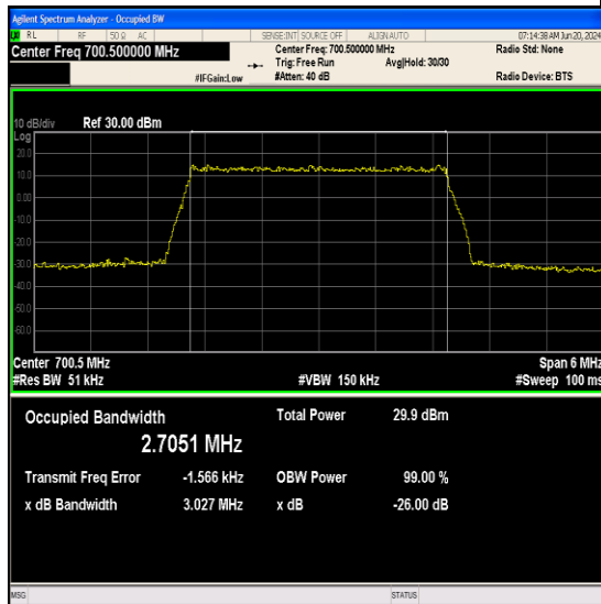
Band12-3MHz-64QAM-23025-15RB#0-PASS
