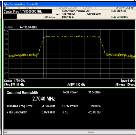
Band66-3MHz-16QAM-132657-15RB#0-PASS
