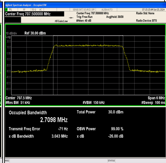
Band12-3MHz-64QAM-23095-15RB#0-PASS
