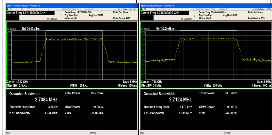
Band66-3MHz-64QAM-131987-15RB#0-PASS
