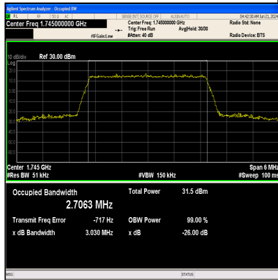
Band66-3MHz-16QAM-132322-15RB#0-PASS
