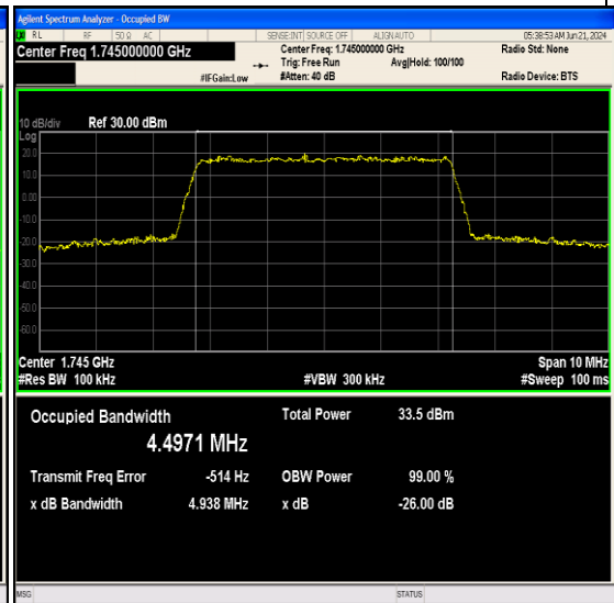
Band66-5MHz-QPSK-132322-25RB#0-PASS
