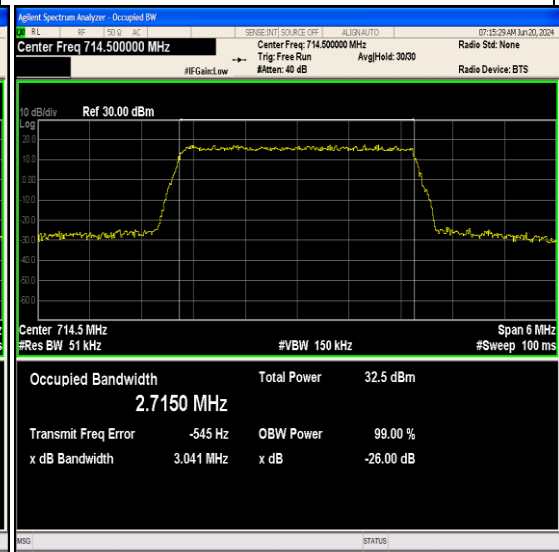
Band12-3MHz-QPSK-23165-15RB#0-PASS
