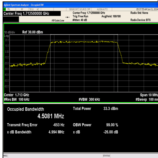
Band66-5MHz-QPSK-131997-25RB#0-PASS
