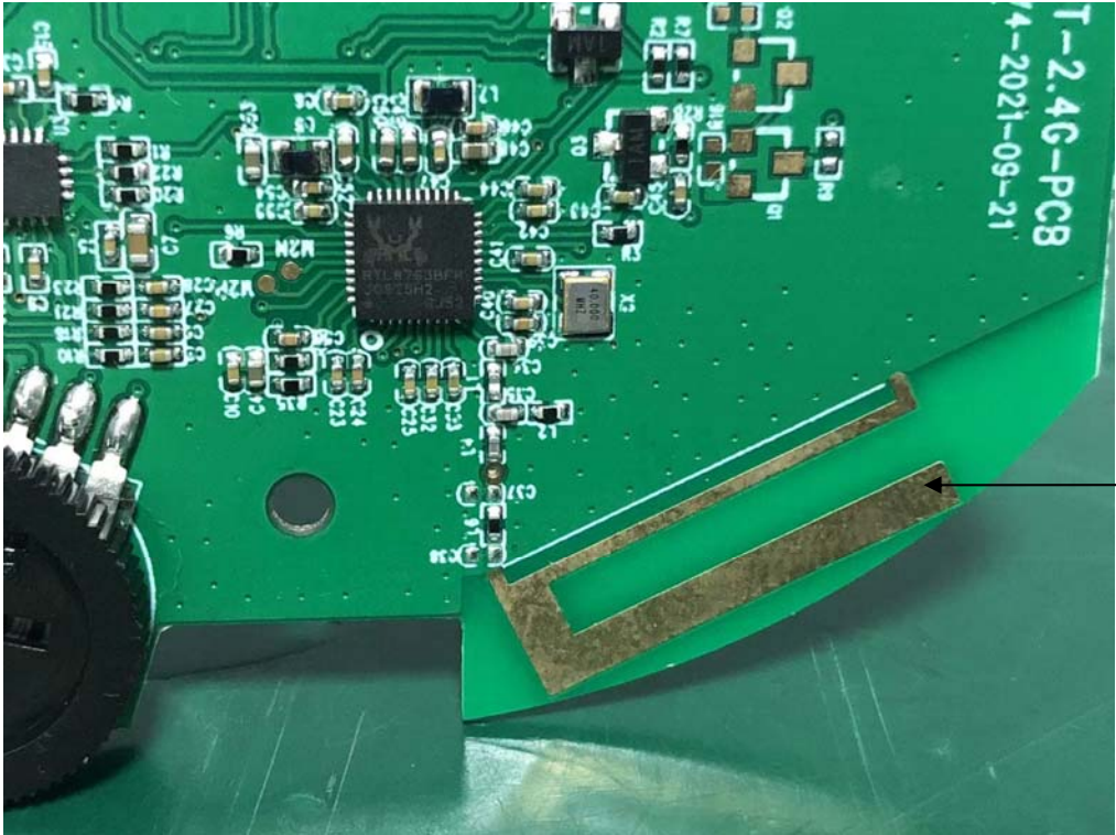
2.4G SRD Antenna
