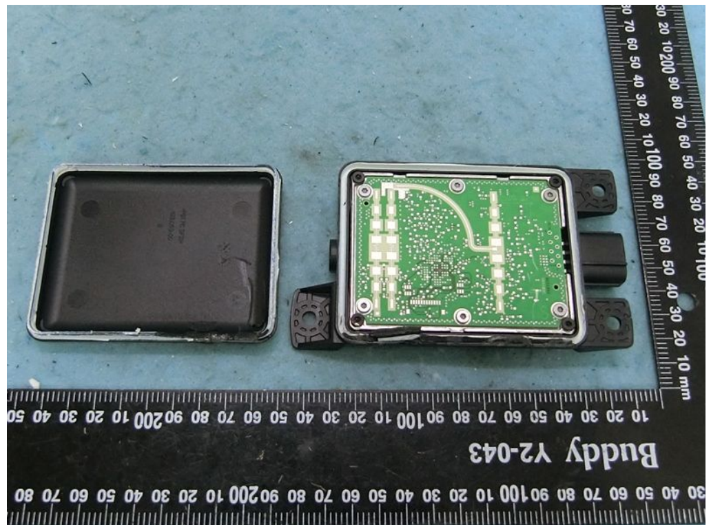
Slave Control Unit (EUT)
