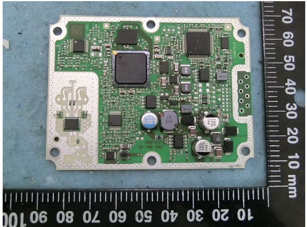
Master Control Unit (EUT)
