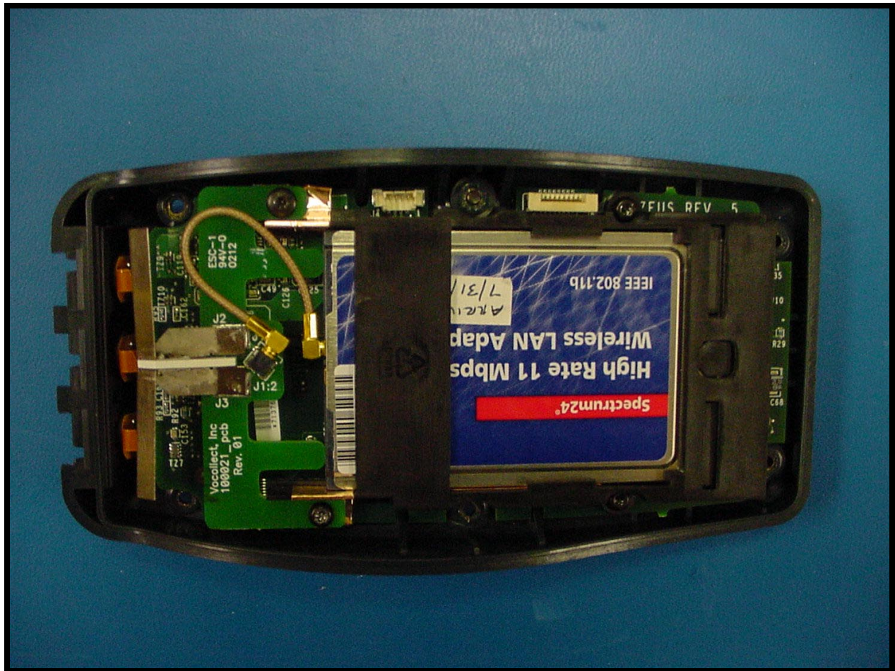
PHOTOGRAPH 10: INTERNAL VIEW WITH WLAN CARD
