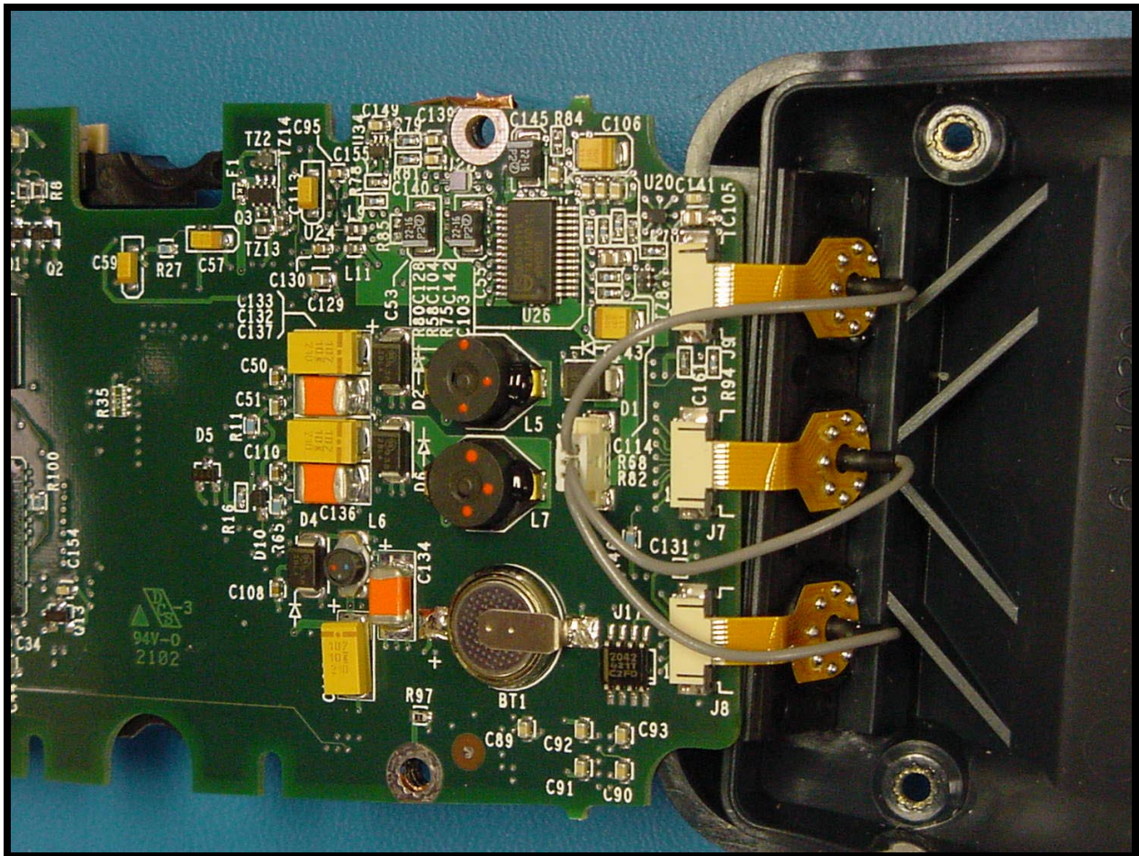
PHOTOGRAPH 21: PCB CONNECTIONS
