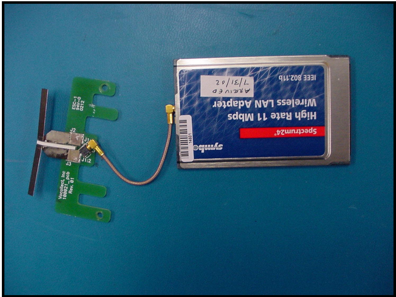
PHOTOGRAPH 16: WLAN CARD FRONT WITH ANTENNA
