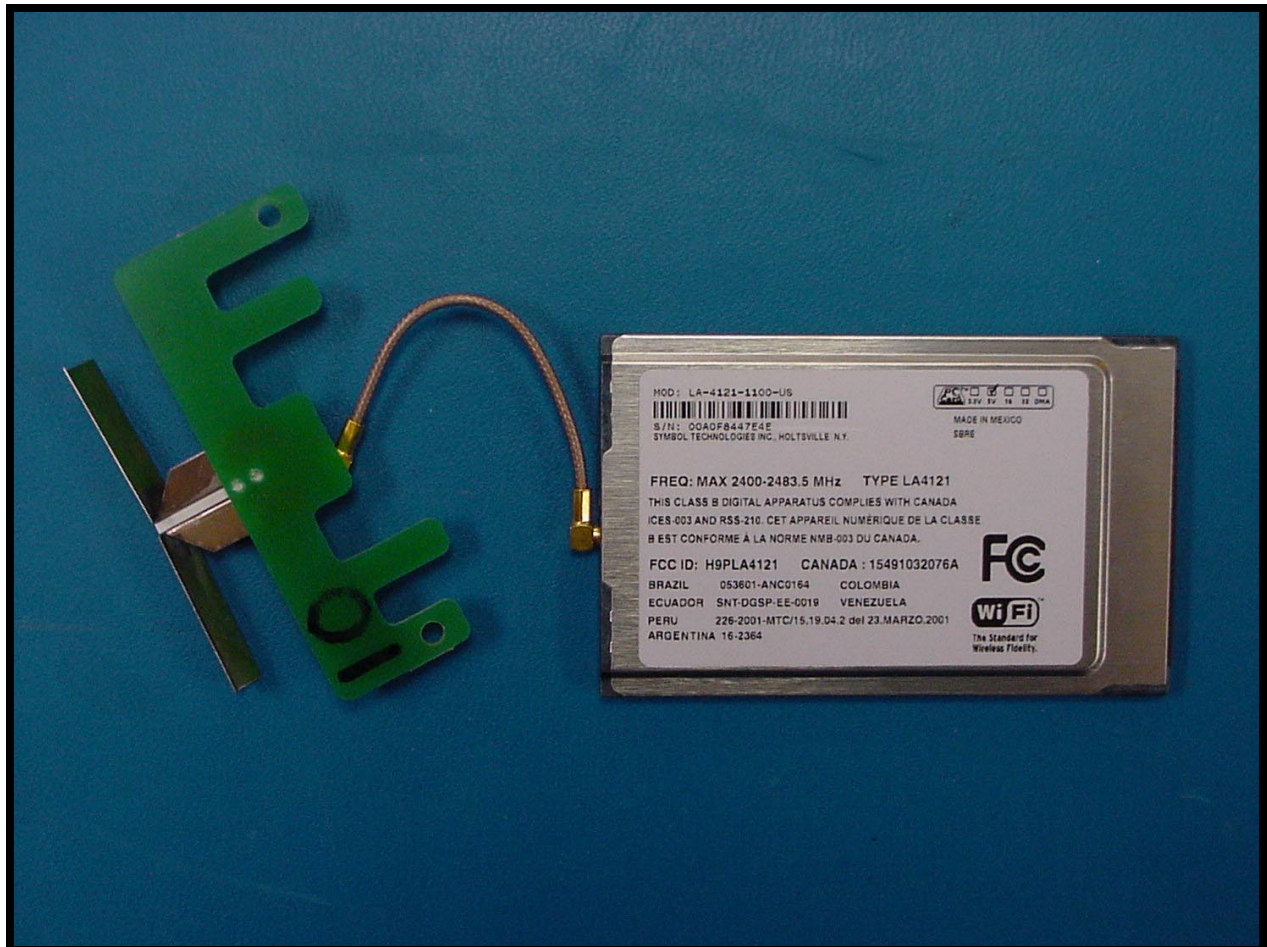
PHOTOGRAPH 17: WLAN CARD REAR WITH ANTENNA
