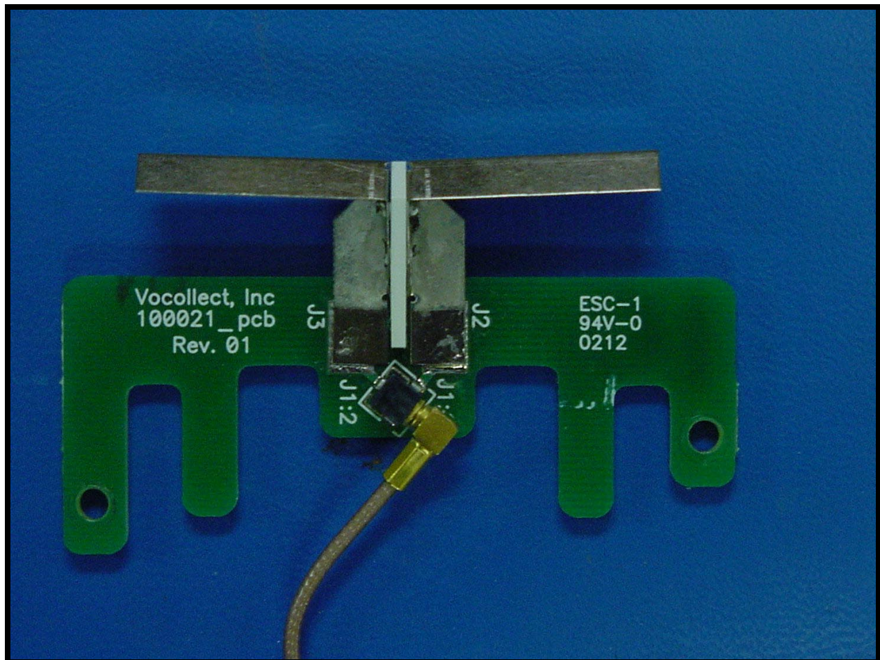
PHOTOGRAPH 18: ANTENNA FRONT
