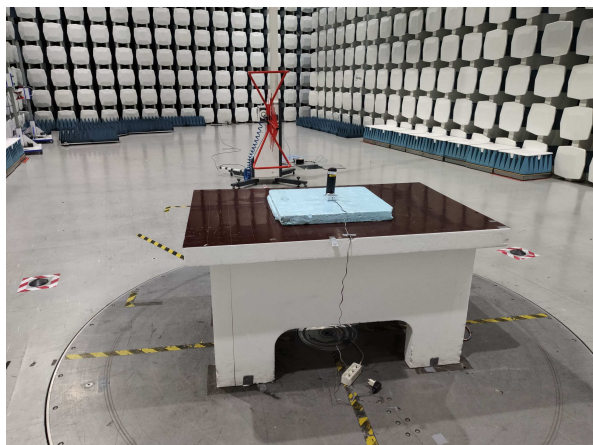
Radiated Emissions 30 – 1000 MHz, Charging
