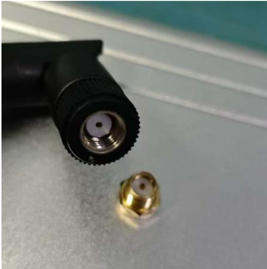
RP-SMA antenna port
