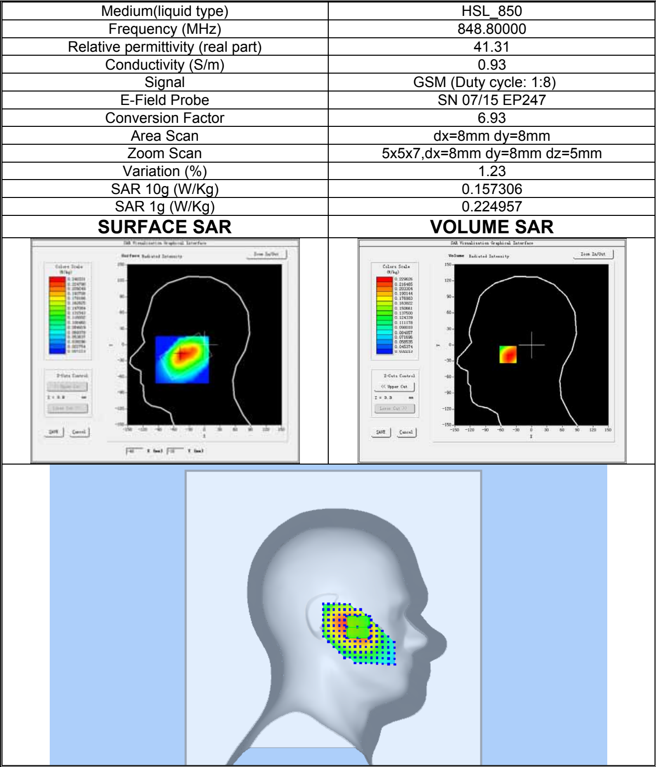
Plot 3: GSM850MHz, High channel (Left Head , Cheek) Product Description: MOBILE PHONE Test Date:2018-09-25
