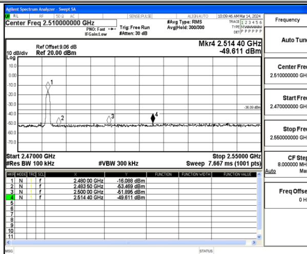
2DH5-Ant1-2480-PASS
