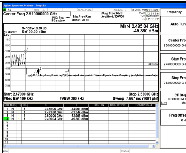
DH5-Ant1-Hop_2480-PASS
