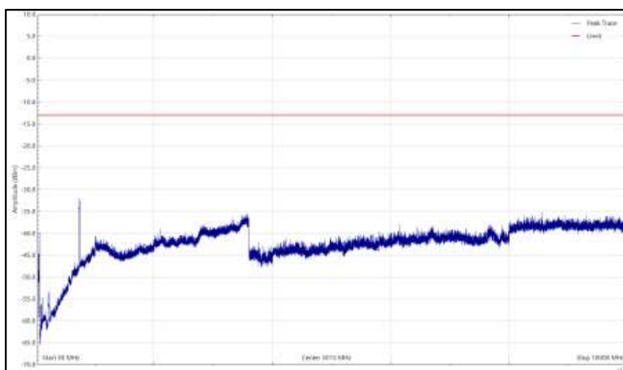
Bot - NR&NB-IoT - B12A, 734, 30 MHz to 10 GHz, Vertical (Peak)
