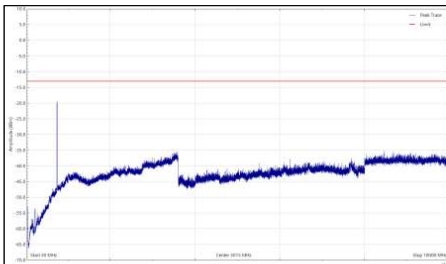
Mid - NR&NB-IoT - B12A, 737, 30 MHz to 10 GHz, Horizontal (Peak)
