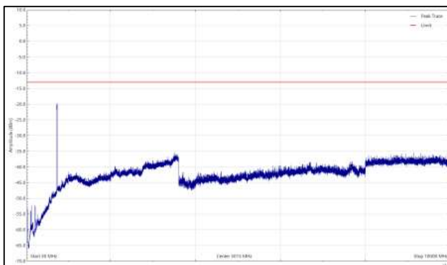
Bot - NR&NB-IoT - B12A, 734, 30 MHz to 10 GHz, Horizontal (Peak)
