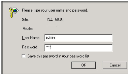
Figure 6-3: Login window
