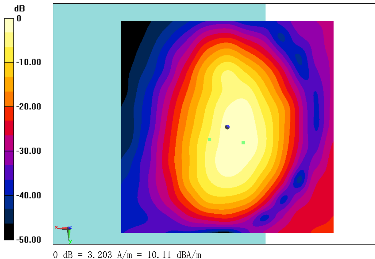
Fig B.28 T-Coil LTE B25
