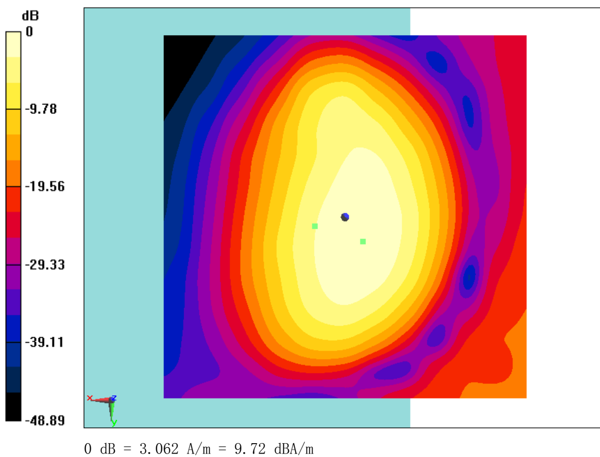
Fig B.10 T-Coil WCDMA 1700
