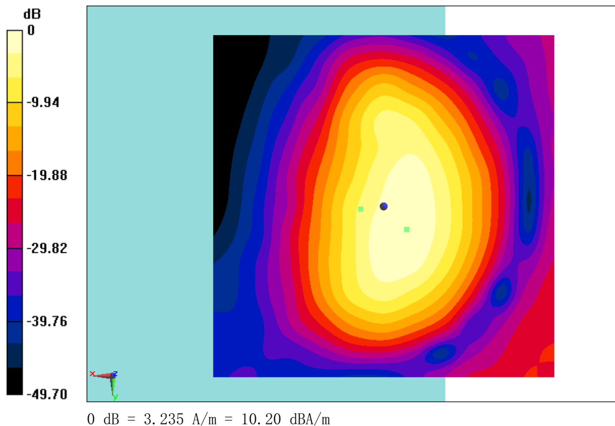
Fig B.18 T-Coil LTE B2
