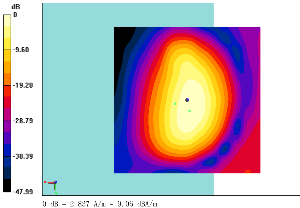
Fig B.36 T-Coil LTE B71
