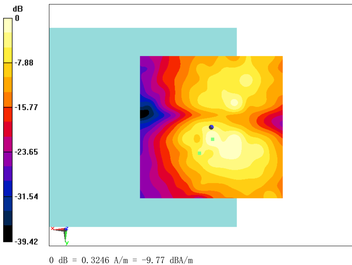
Fig B.39 T-Coil GSM 1900
