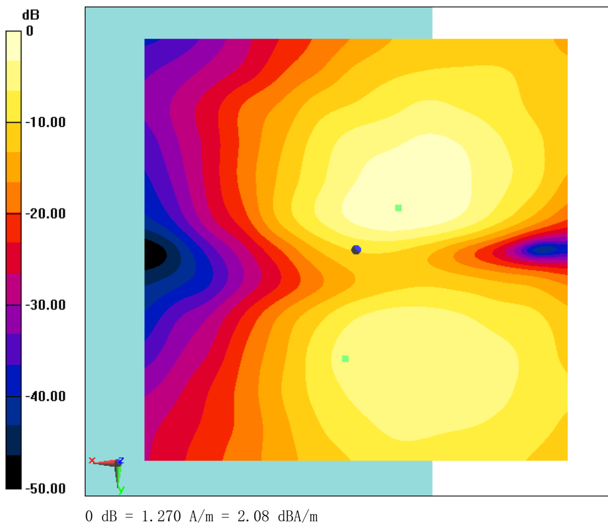
Fig B.33 T-Coil LTE B41
