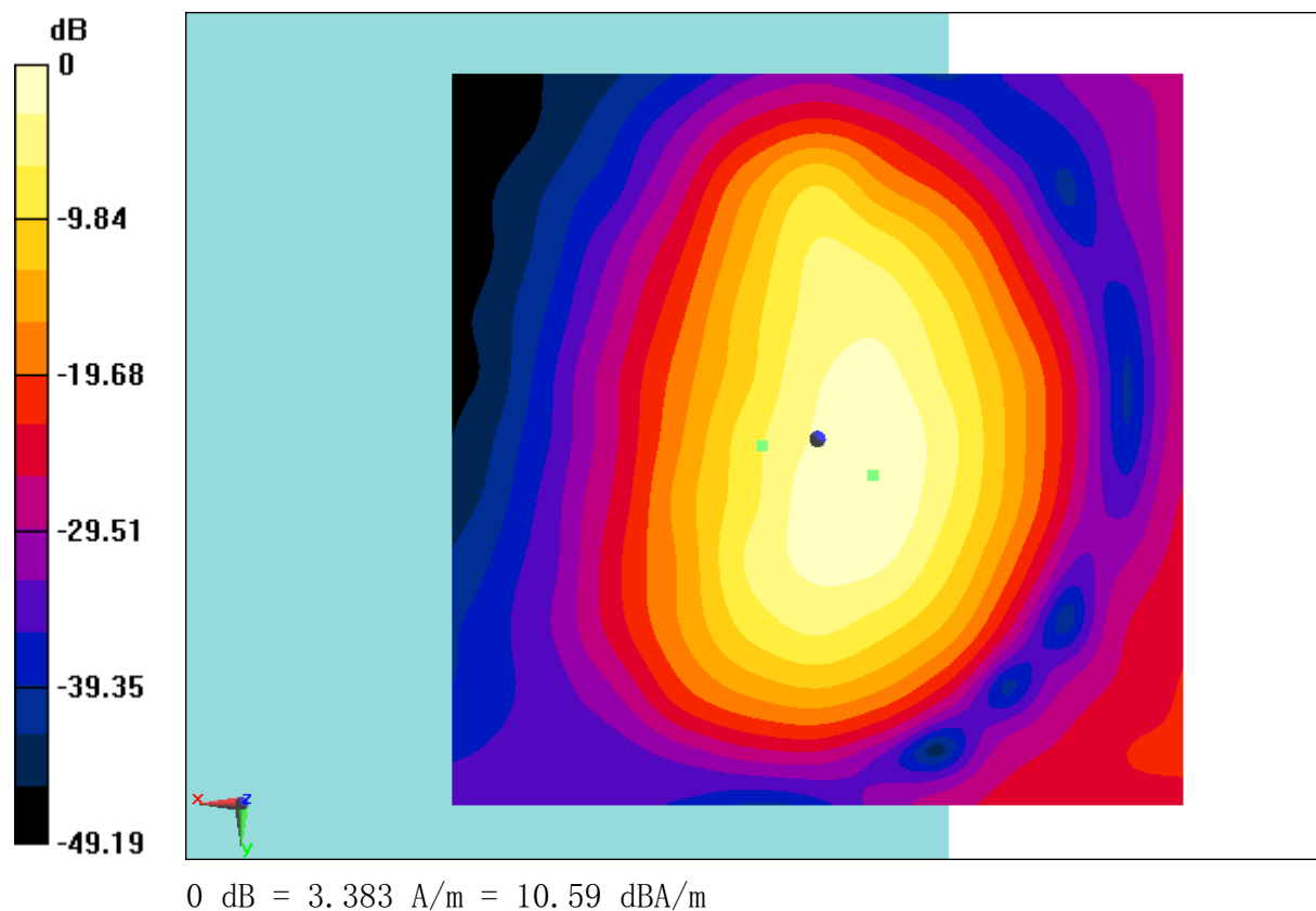
Fig B.24 T-Coil LTE B12
