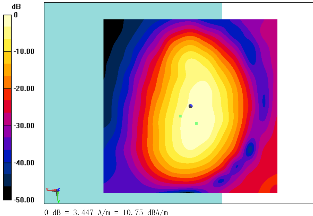
Fig B.26 T-Coil LTE B13
