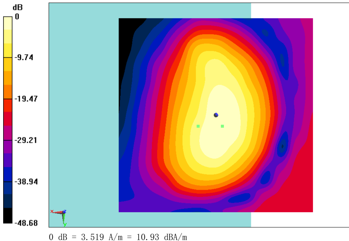
Fig B.22 T-Coil LTE B5
