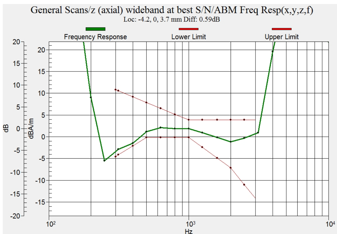
Figure C.4 Frequency Response of WCDMA 1900
