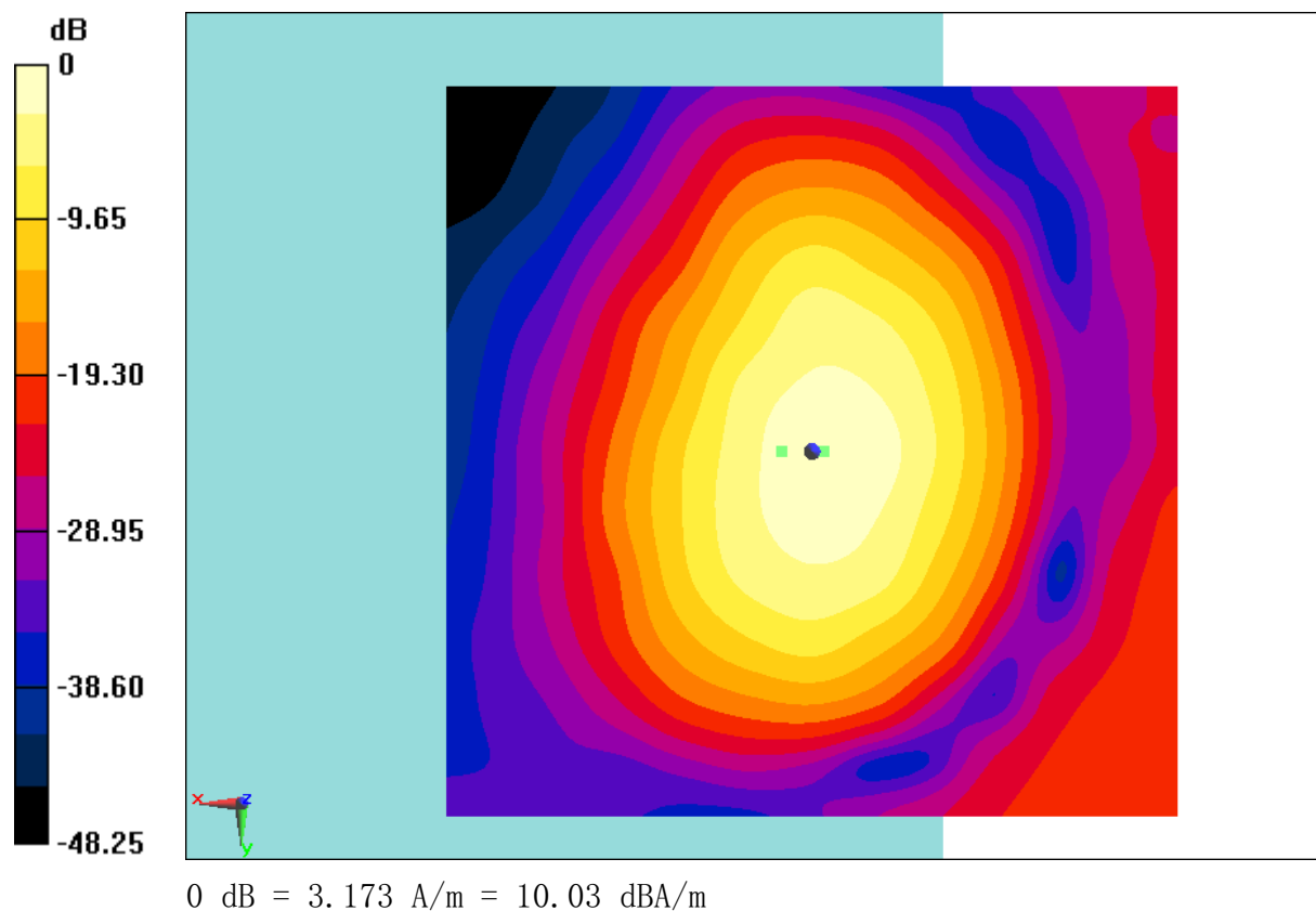
Fig B.32 T-Coil LTE B41
