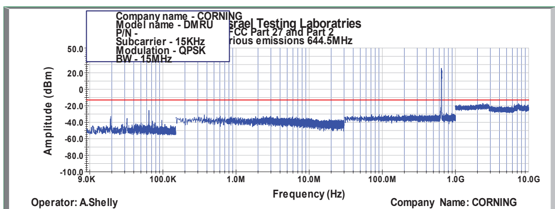
Figure 542: Spurious Emissions at Antenna Terminal QPSK, 644.5MHz, B.W. 15MHz, Sub Carrier 15kHz
