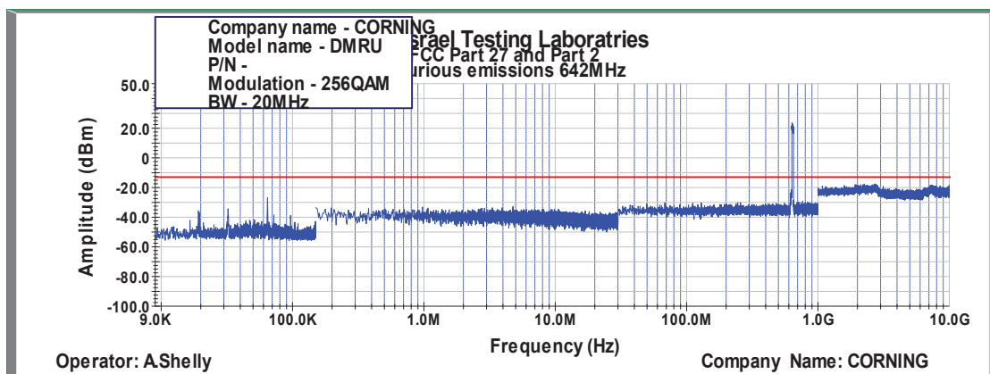
Figure 524: Spurious Emissions at Antenna Terminal 256QAM, 642.0MHz, B.W. 20MHz, Sub Carrier 15kHz
