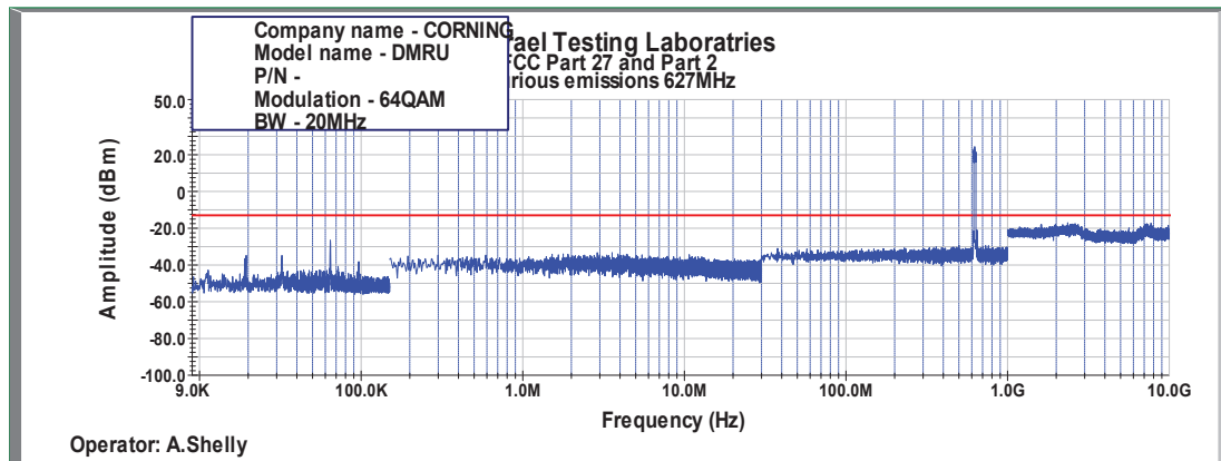
Figure 498: Spurious Emissions at Antenna Terminal 64QAM, 627.0MHz, B.W. 20MHz, Sub Carrier 15kHz
