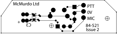
SOLDER SIDE
