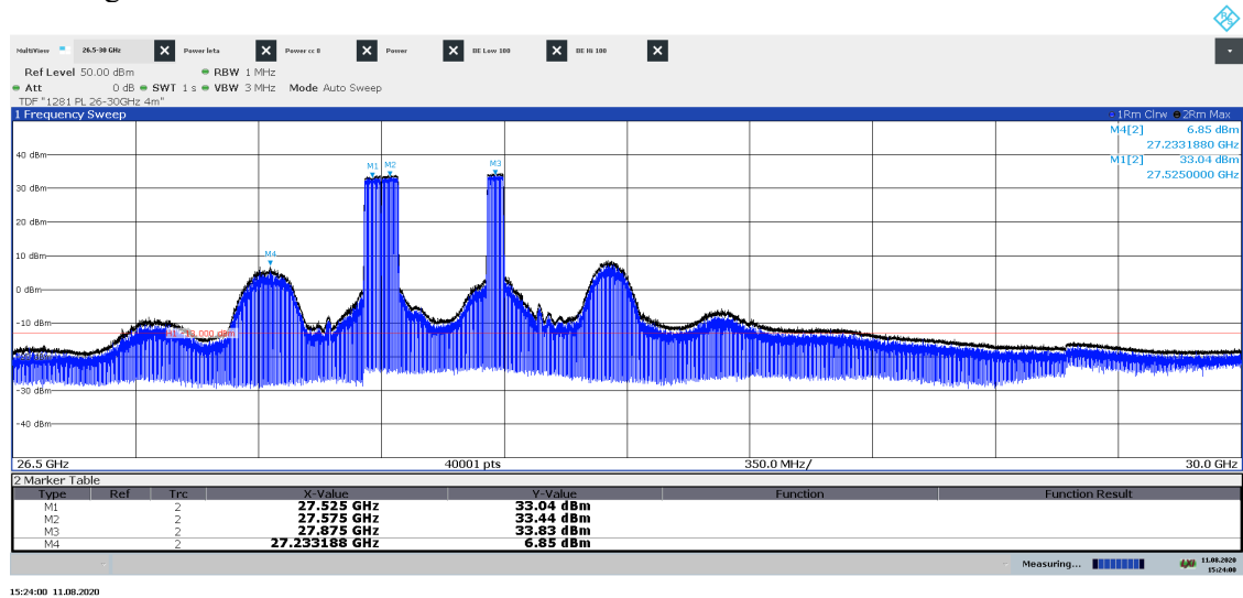
Diagram 2.9b: Pre scan 26.5 – 30.0 GHz, Symbolic name: Bim3 50 , EIRP Vertical polarization See diagram 2.9e for TRP result
