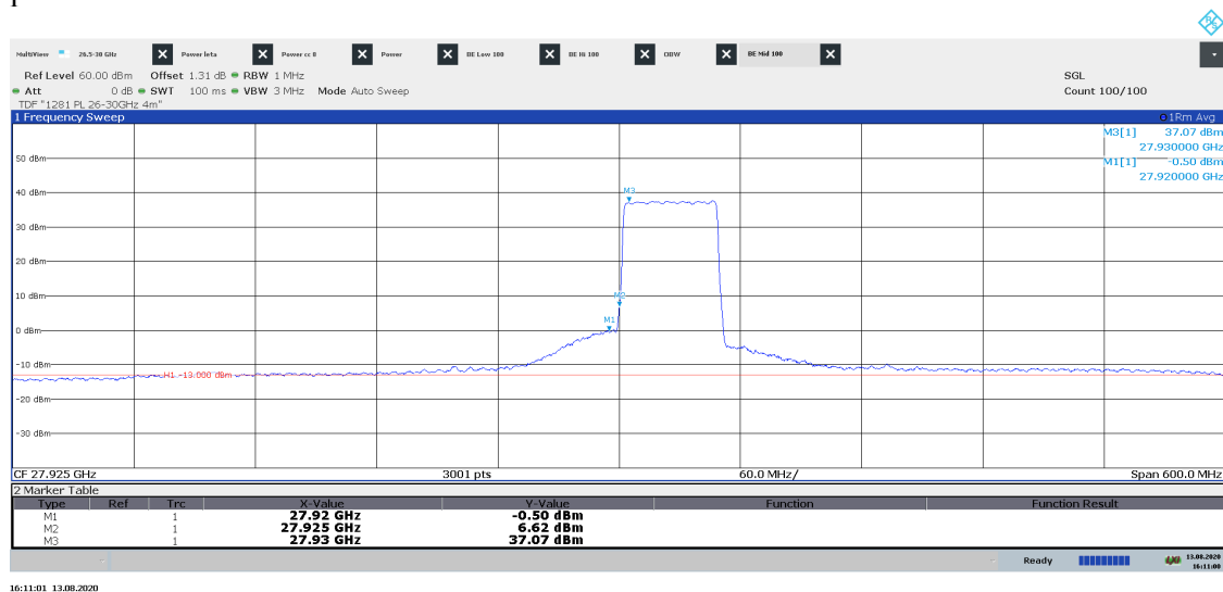
Diagram 2.11b: Pre scan 27.625 – 28.225 GHz, Symbolic name: BH 50 , EIRP Vertical polarization
