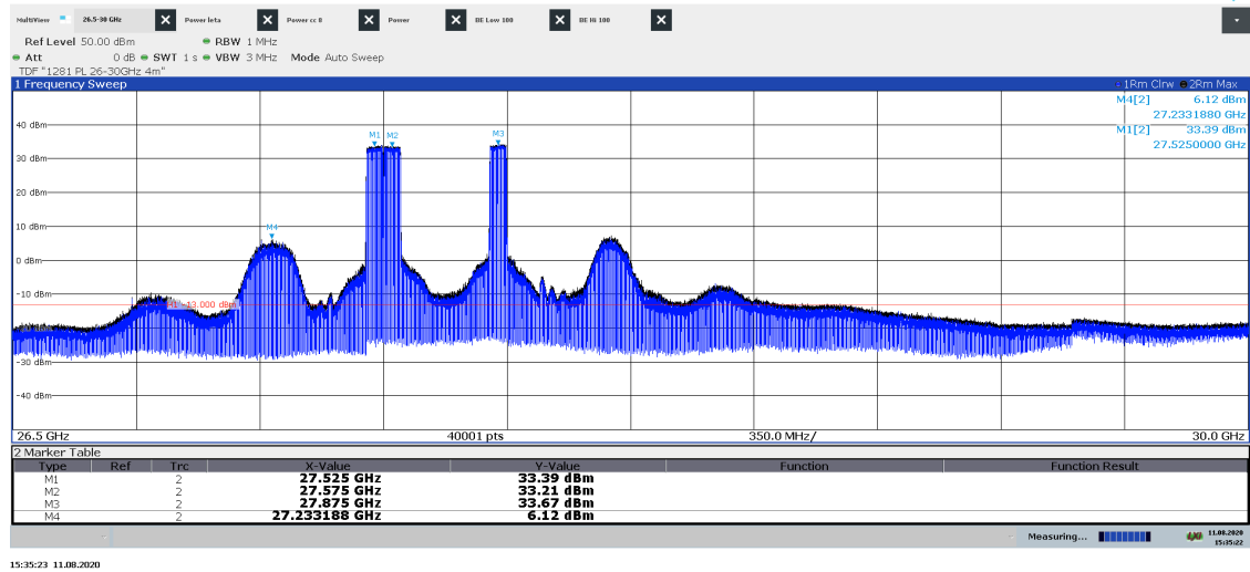
Diagram 2.9a: Pre scan 26.5 – 30.0 GHz, Symbolic name: Bim3 50 , EIRP Horizontal polarization See diagram 2.9e for TRP result
