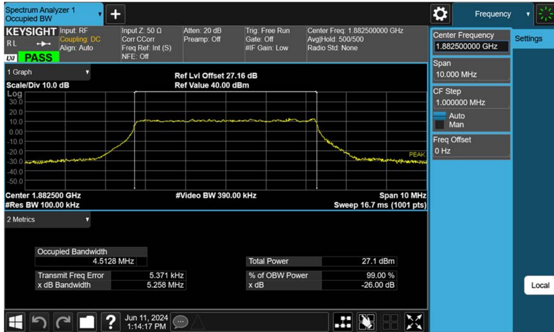
Sub6 n25(2)_5 M_OBW_Mid_256QAM_FullRB
