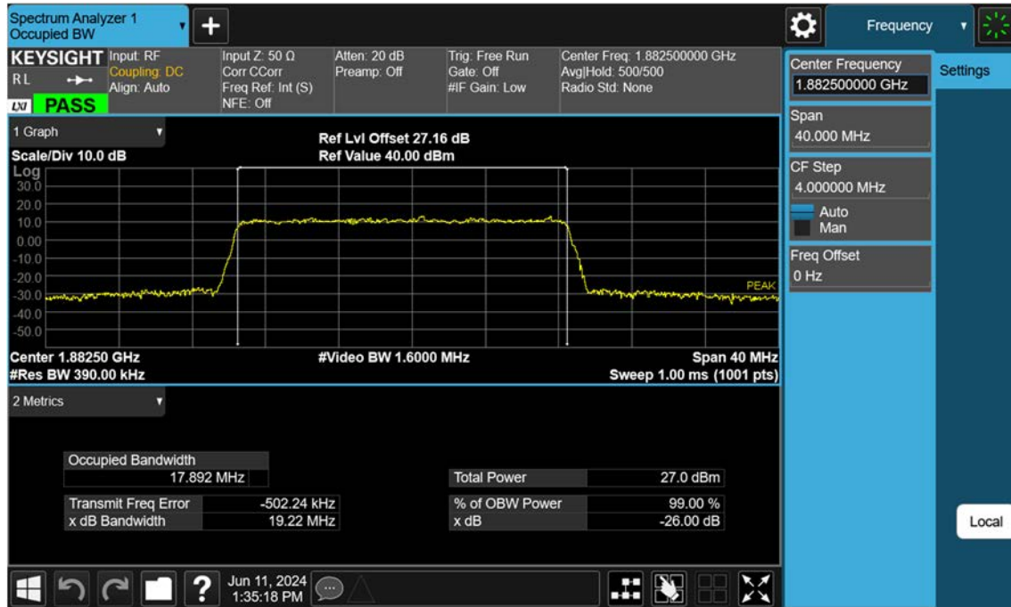
Sub6 n25(2)_20 M_OBW_Mid_256QAM_FullIRB
