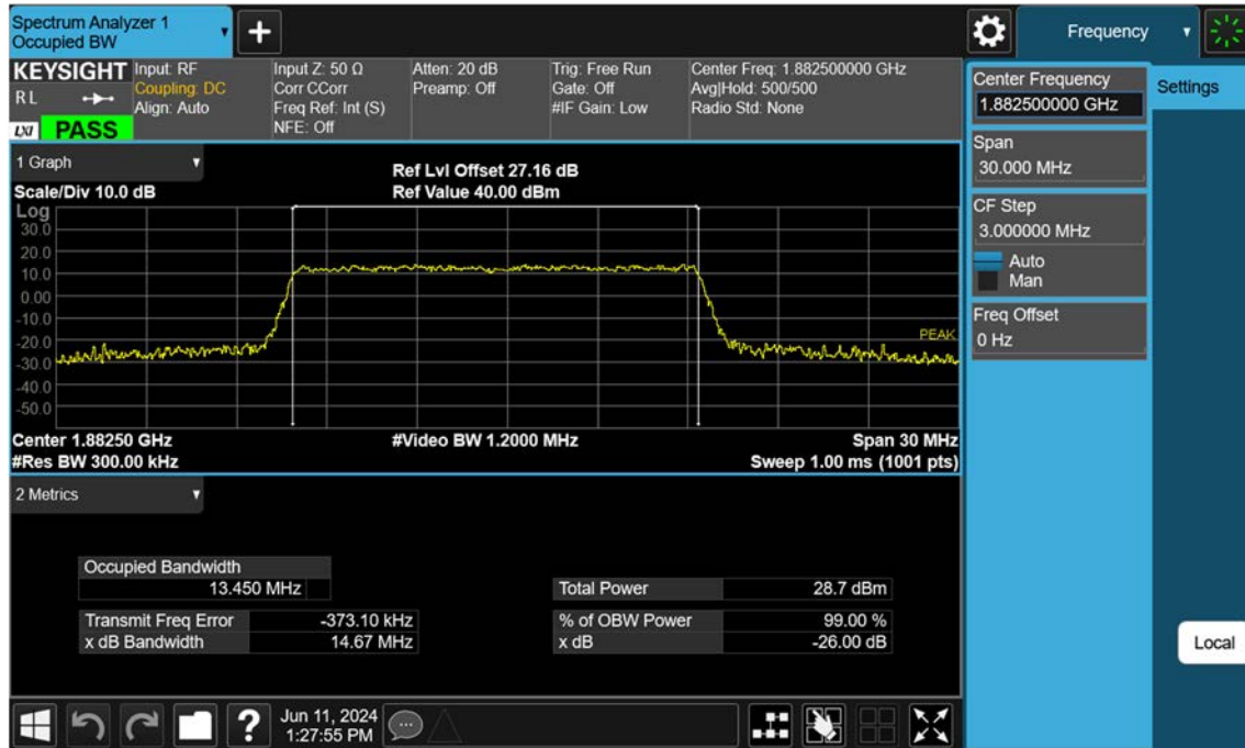
Sub6 n25(2)_15 M_OBW_Mid_64QAM_FullRB
