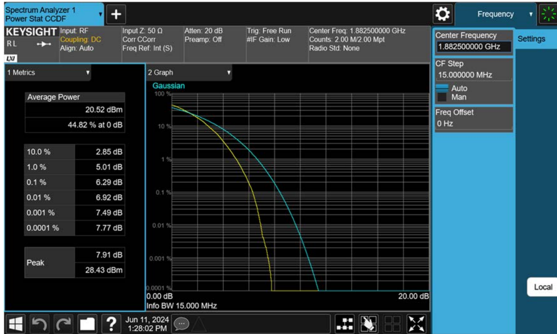
Sub6 n25(2)_15 M_PAR_Mid_64QAM_FullRB
