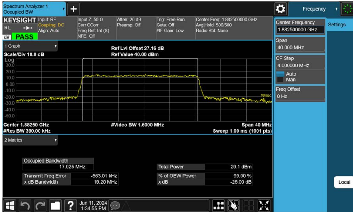
Sub6 n25(2)_20 M_OBW_Mid_64QAM_FullRB
