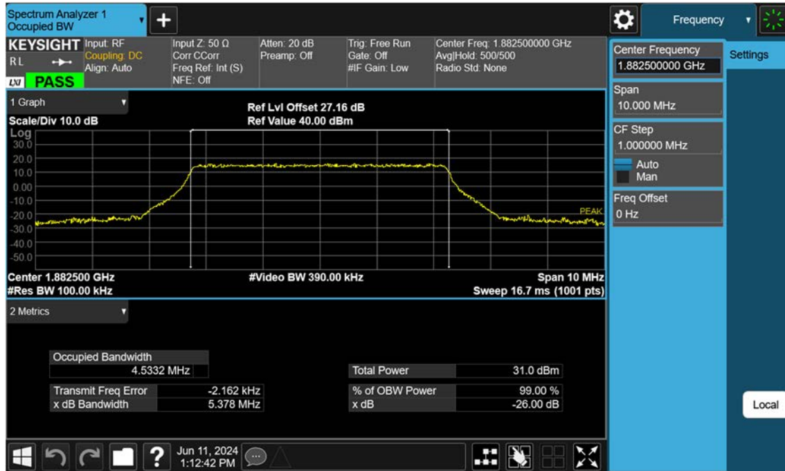
Sub6 n25(2)_5 M_OBW_Mid_QPSK_FullRB
