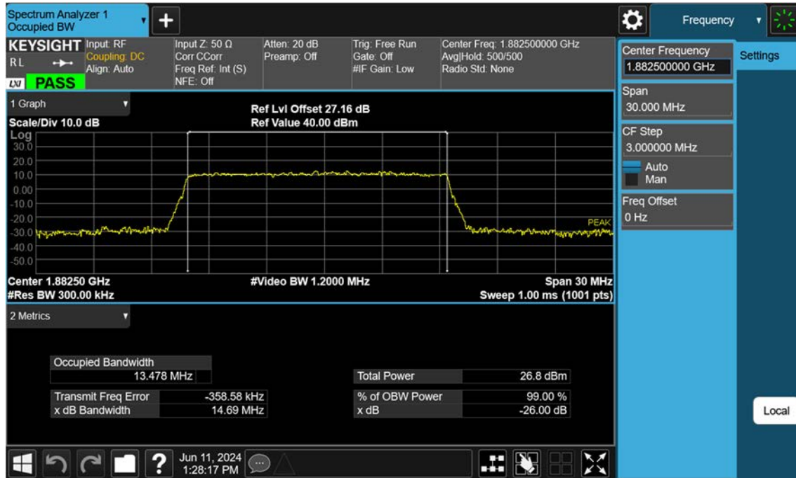
Sub6 n25(2)_15 M_OBW_Mid_256QAM_FullIRB
