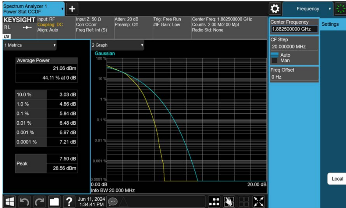
Sub6 n25(2)_20 M_PAR_Mid_16QAM_FullRB
