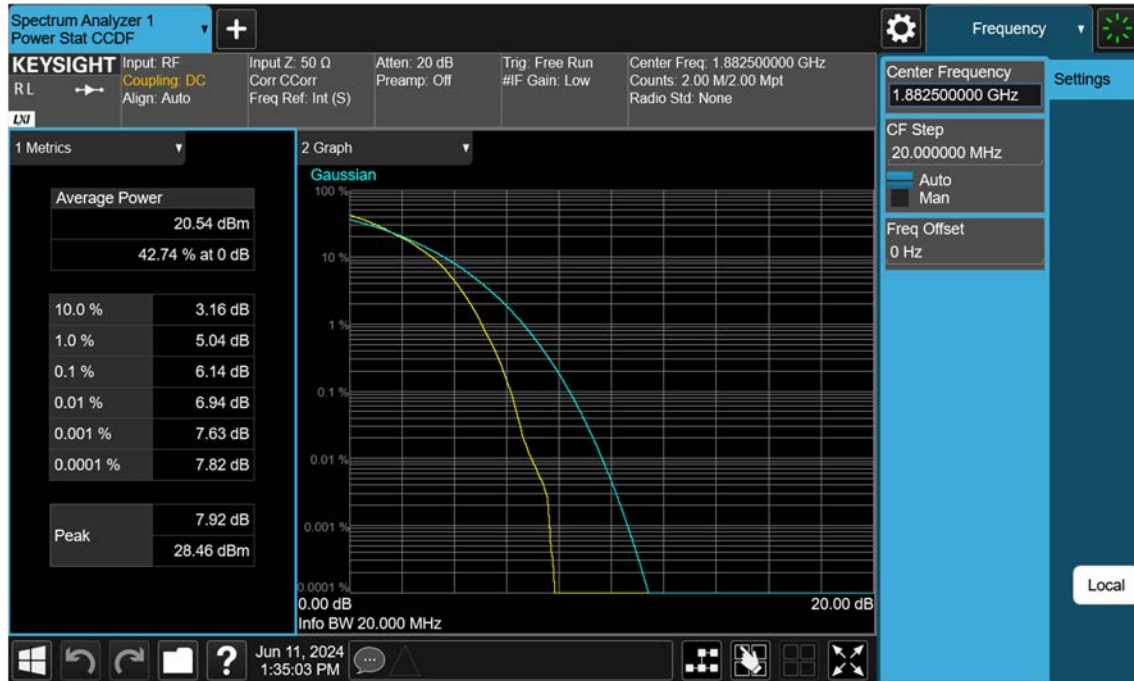
Sub6 n25(2)_20 M_PAR_Mid_64QAM_FullRB
