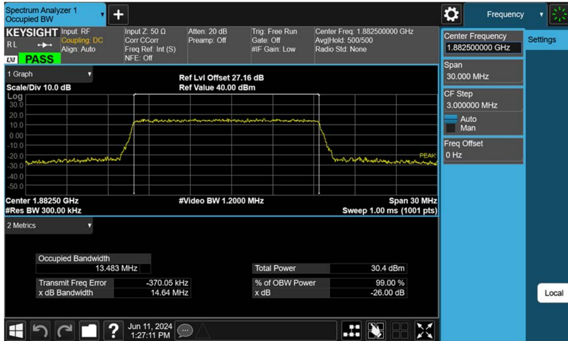
Sub6 n25(2)_15 M_OBW_Mid_QPSK_FullRB
