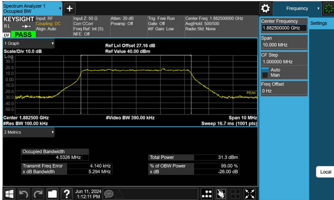
Sub6 n25(2)_5 M_OBW_Mid_BPSK_FullRB
