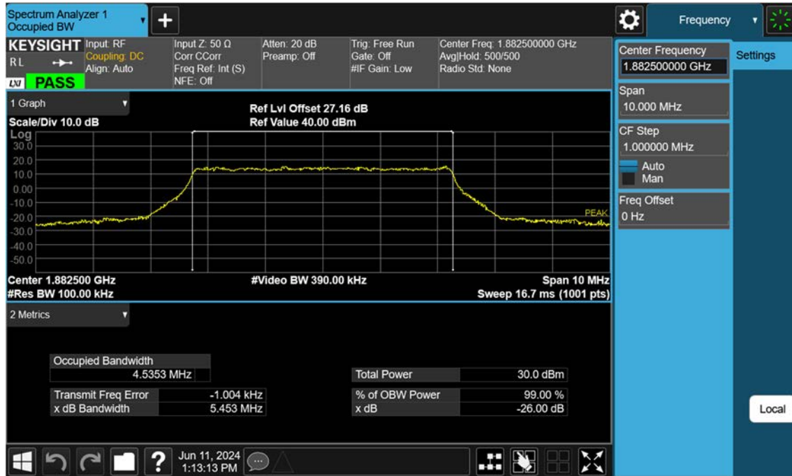
Sub6 n25(2)_5 M_OBW_Mid_16QAM_FullRB
