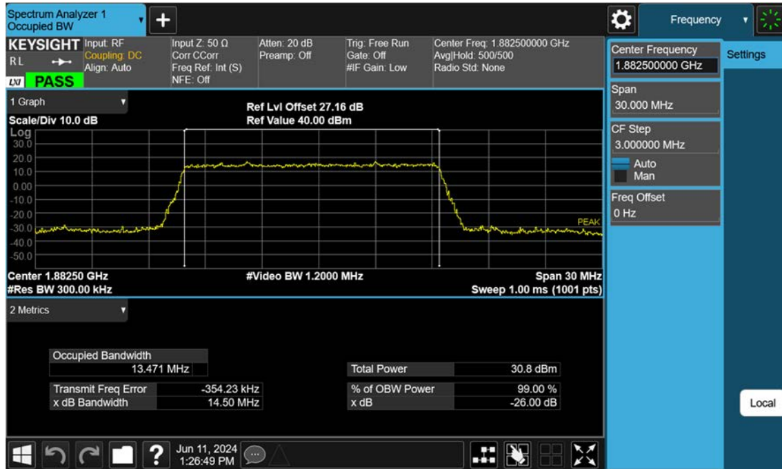
Sub6 n25(2)_15 M_OBW_Mid_BPSK_FullRB
