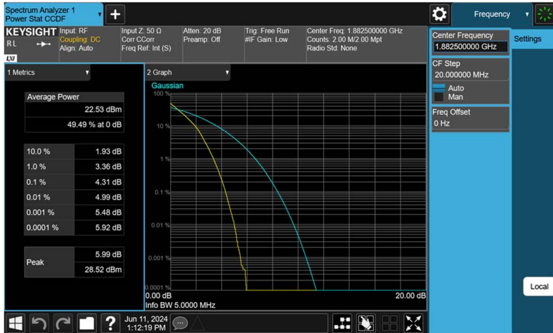
Sub6 n25(2)_5 M_PAR_Mid_BPSK_FullRB
