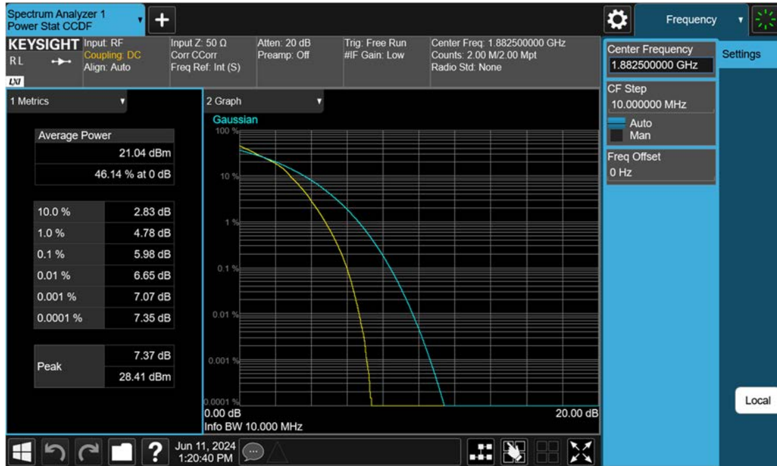
Sub6 n25(2)_10 M_PAR_Mid_16QAM_FullRB
