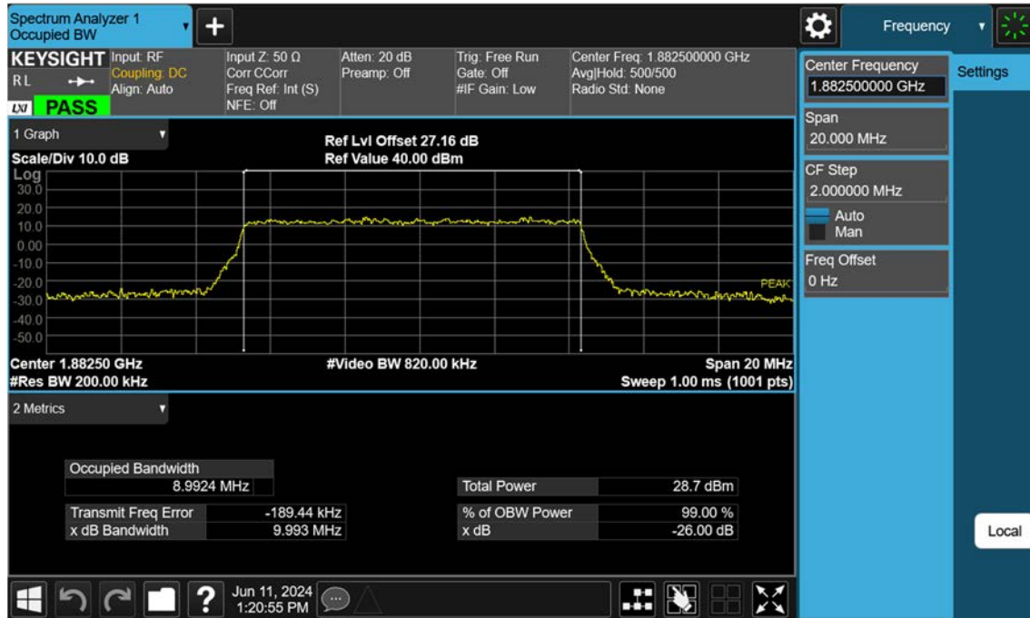
Sub6 n25(2)_10 M_OBW_Mid_64QAM_FullRB
