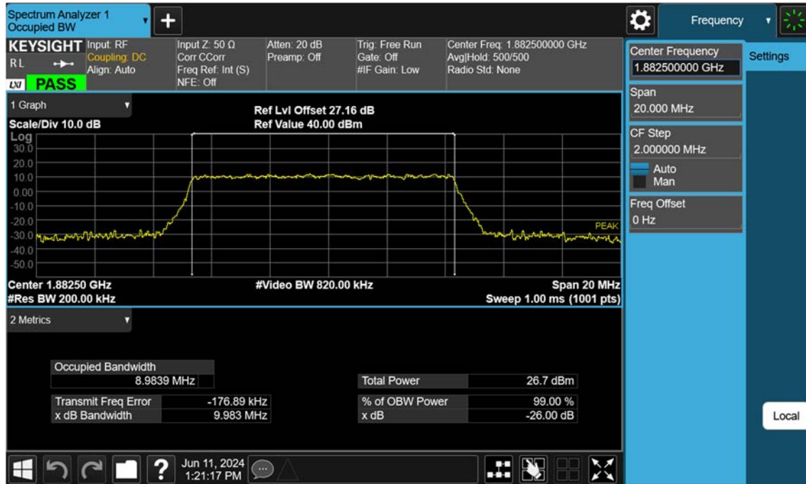
Sub6 n25(2)_10 M_OBW_Mid_256QAM_FullIRB
