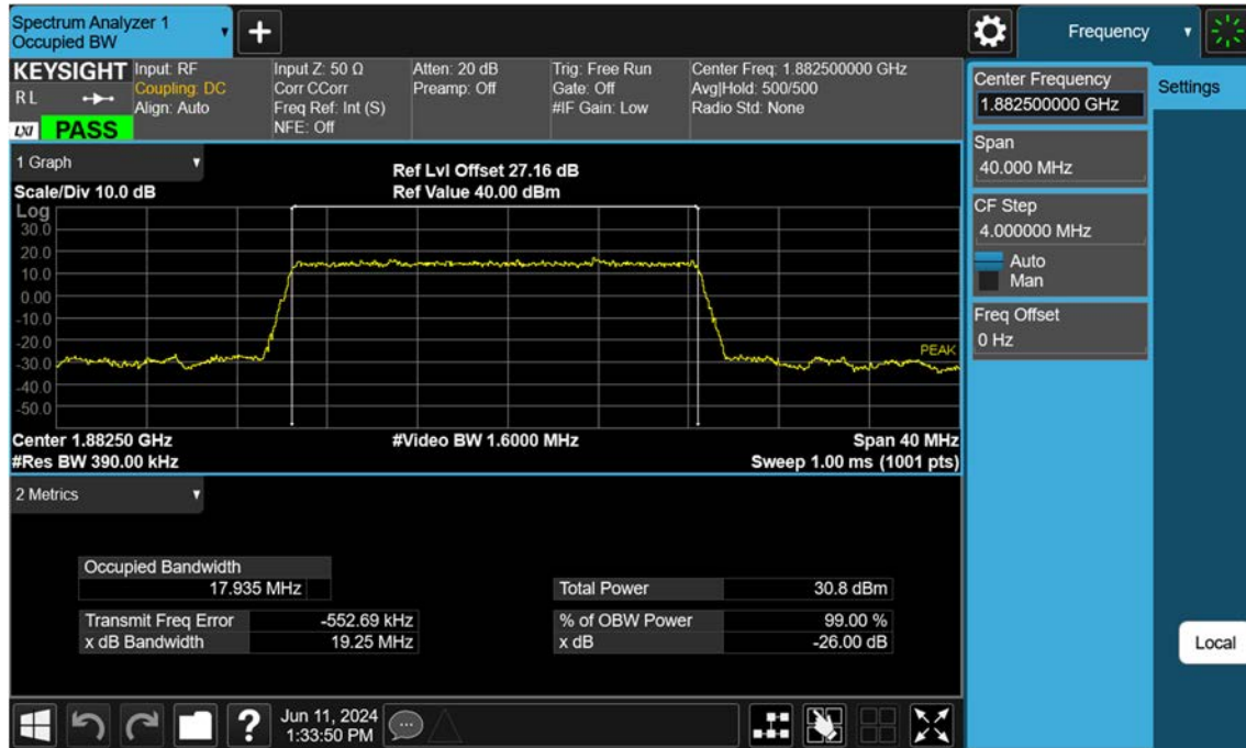
Sub6 n25(2)_20 M_OBW_Mid_BPSK_FullRB
