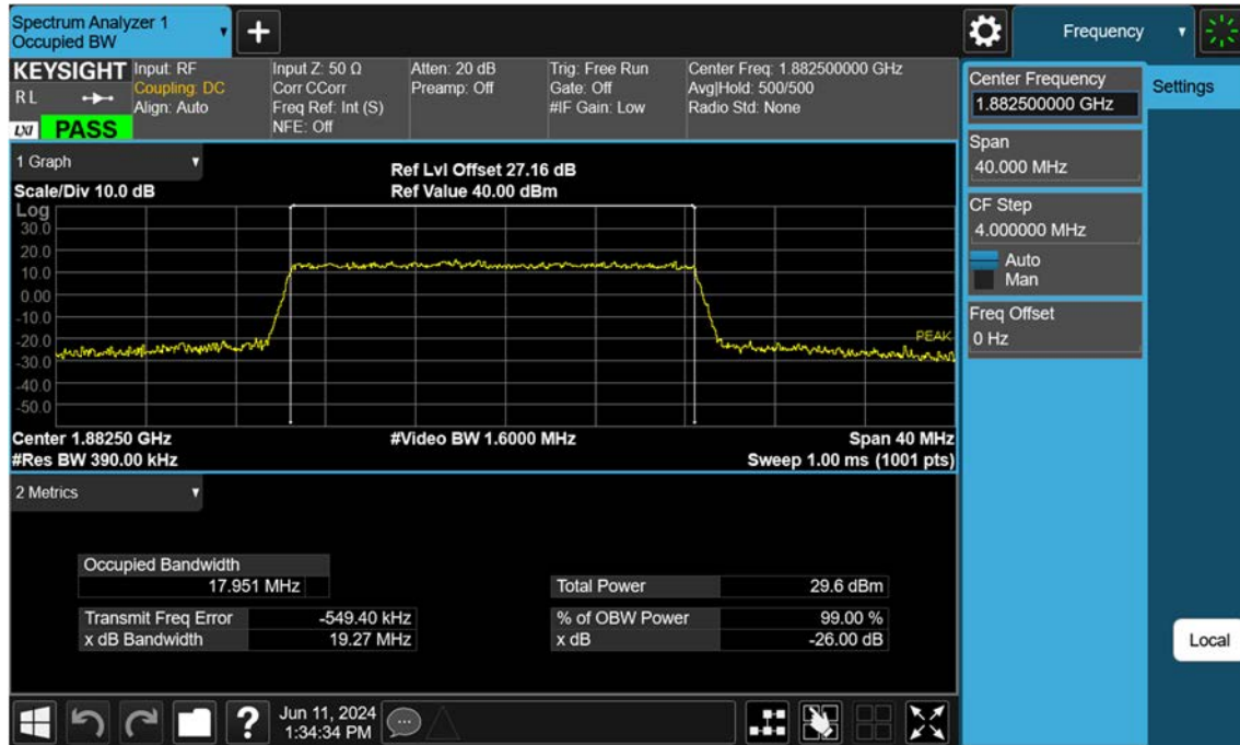
Sub6 n25(2)_20 M_OBW_Mid_16QAM_FullRB
