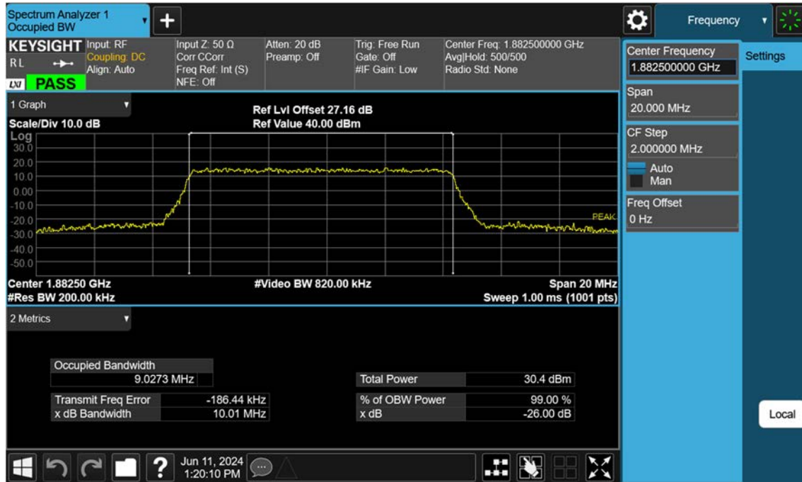
Sub6 n25(2)_10 M_OBW_Mid_QPSK_FullRB
