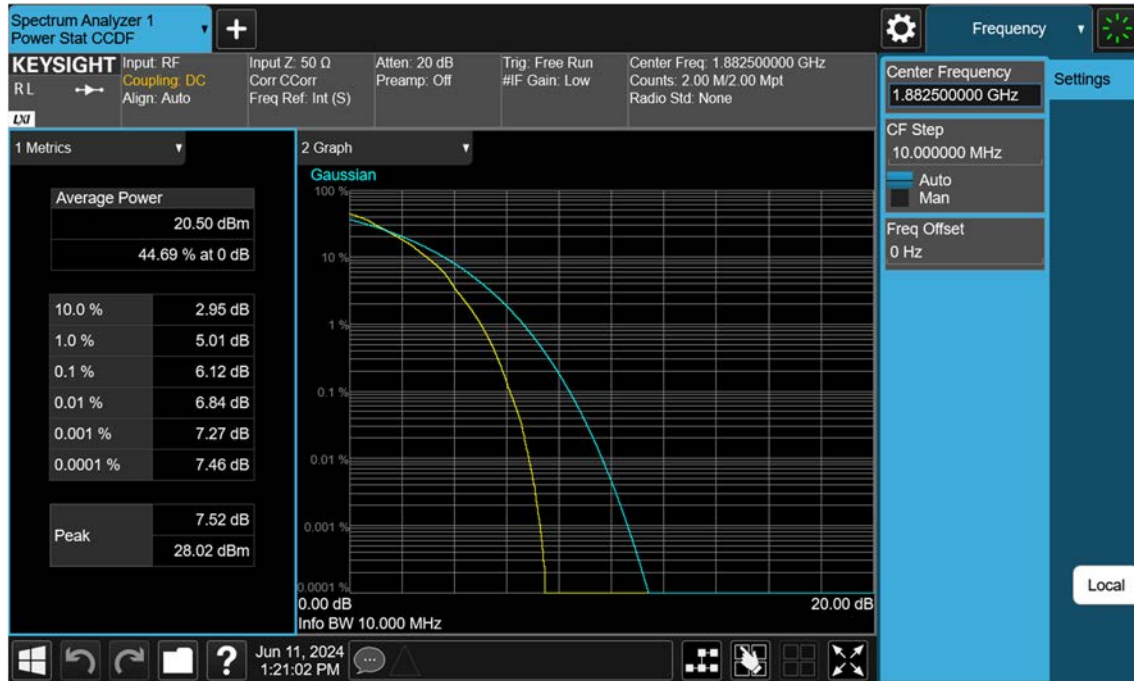
Sub6 n25(2)_10 M_PAR_Mid_64QAM_FullRB
