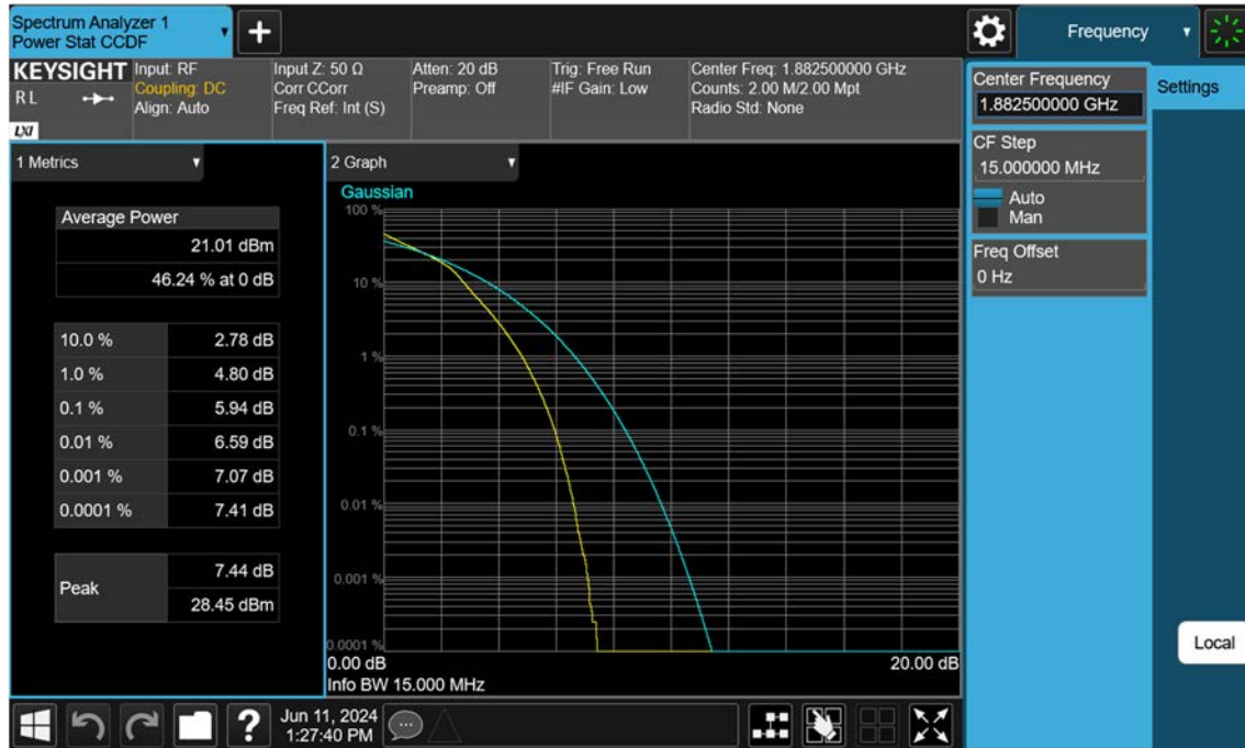
Sub6 n25(2)_15 M_PAR_Mid_16QAM_FullRB
