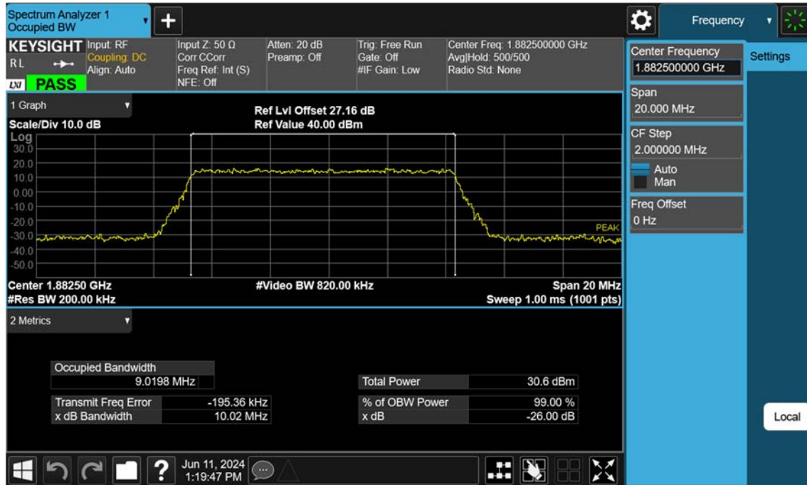
Sub6 n25(2)_10 M_OBW_Mid_BPSK_FullRB
