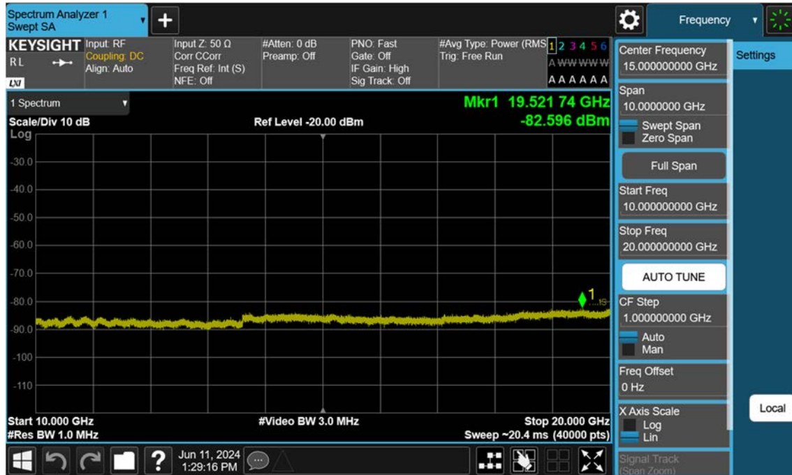
Sub6 n25(2)_15 M_Conducted Spurious(Above10 G)_Mid_BPSK_1RB
