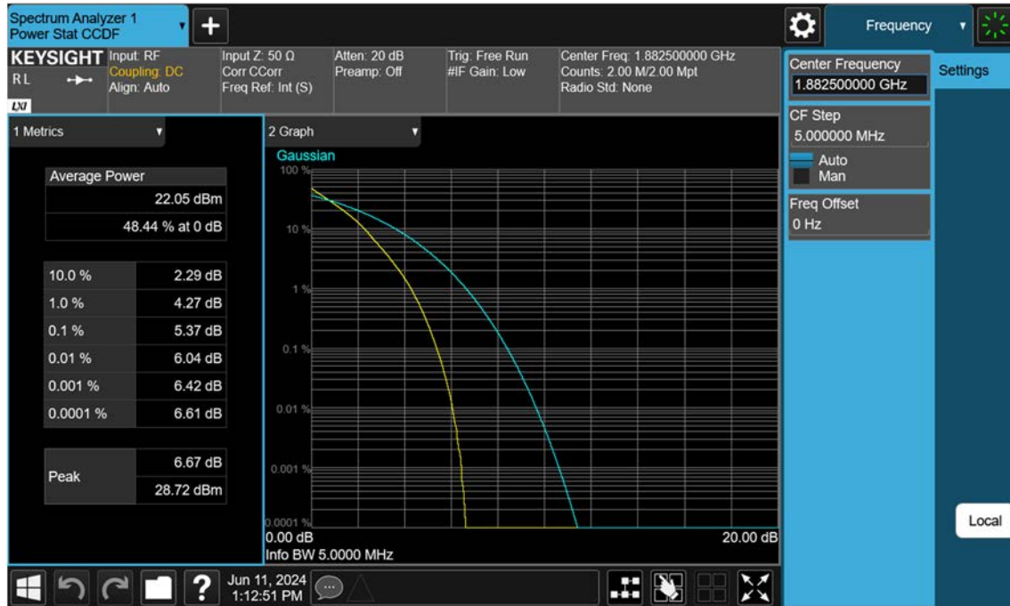
Sub6 n25(2)_5 M_PAR_Mid_QPSK_FullRB
