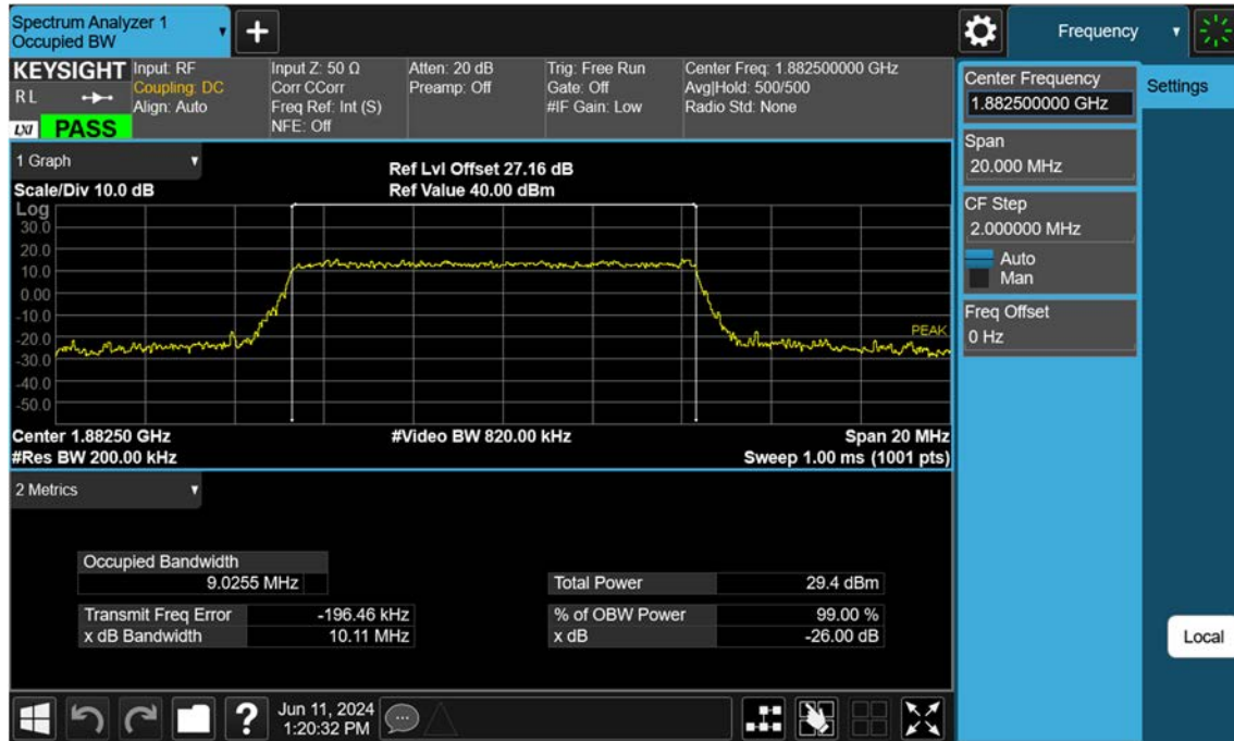
Sub6 n25(2)_10 M_OBW_Mid_16QAM_FullRB
