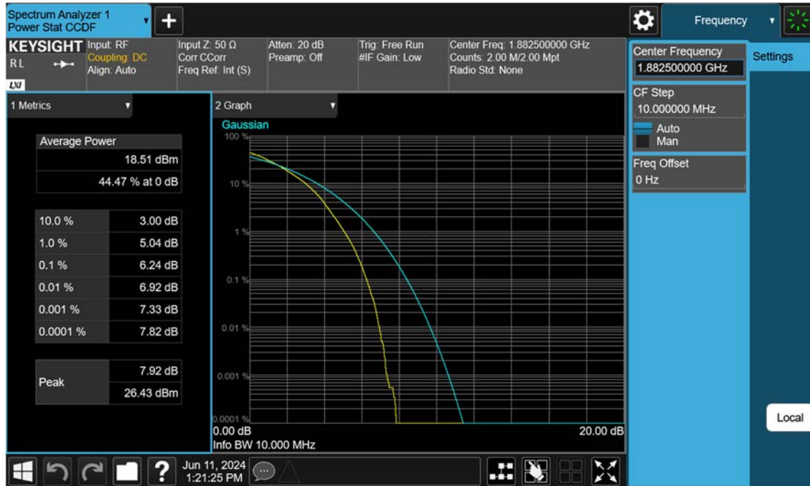
Sub6 n25(2)_10 M_PAR_Mid_256QAM_FullRB
