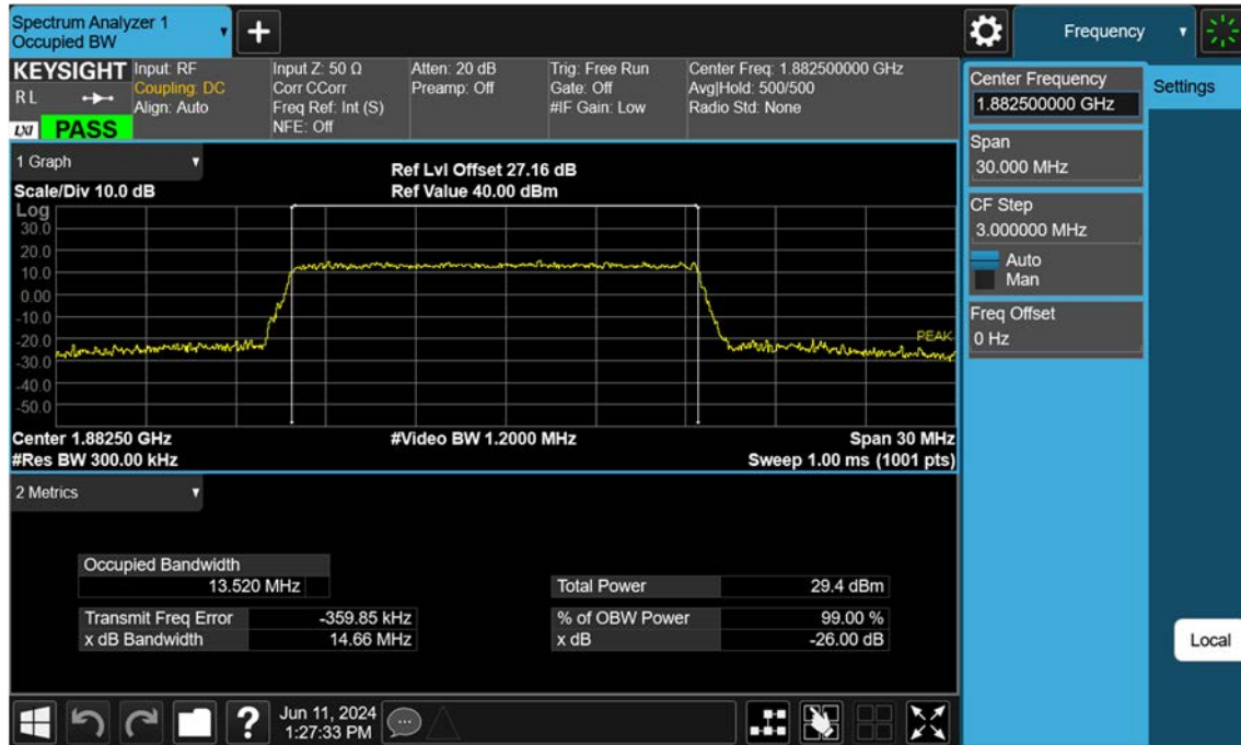
Sub6 n25(2)_15 M_OBW_Mid_16QAM_FullRB
