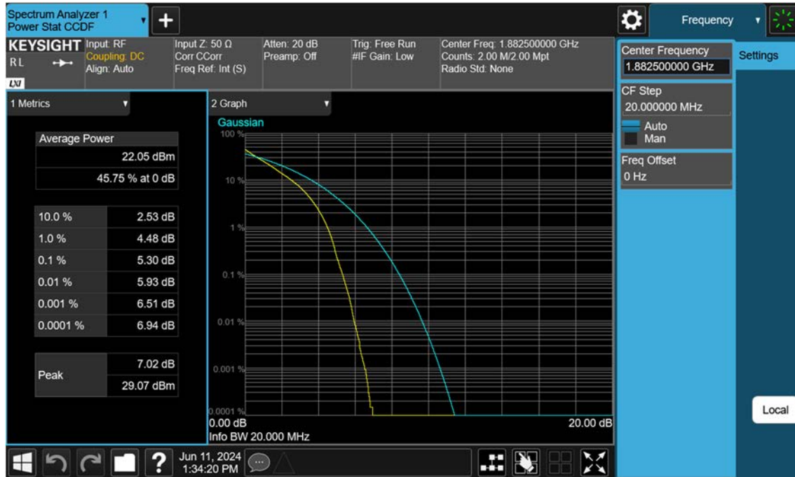
Sub6 n25(2)_20 M_PAR_Mid_QPSK_FullRB
