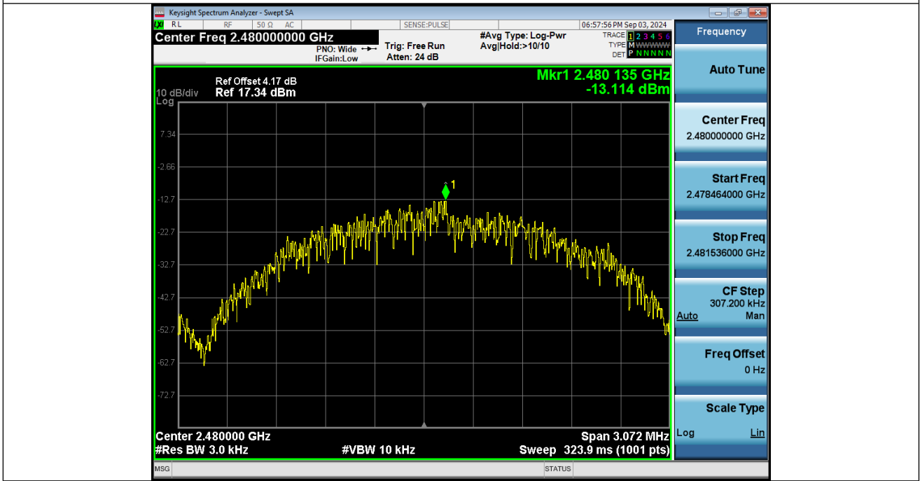
Power_Spectral_Density_NVNT_ANT1_2Mbps_2480
