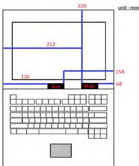
Fig.6 Antenna position of EUT
