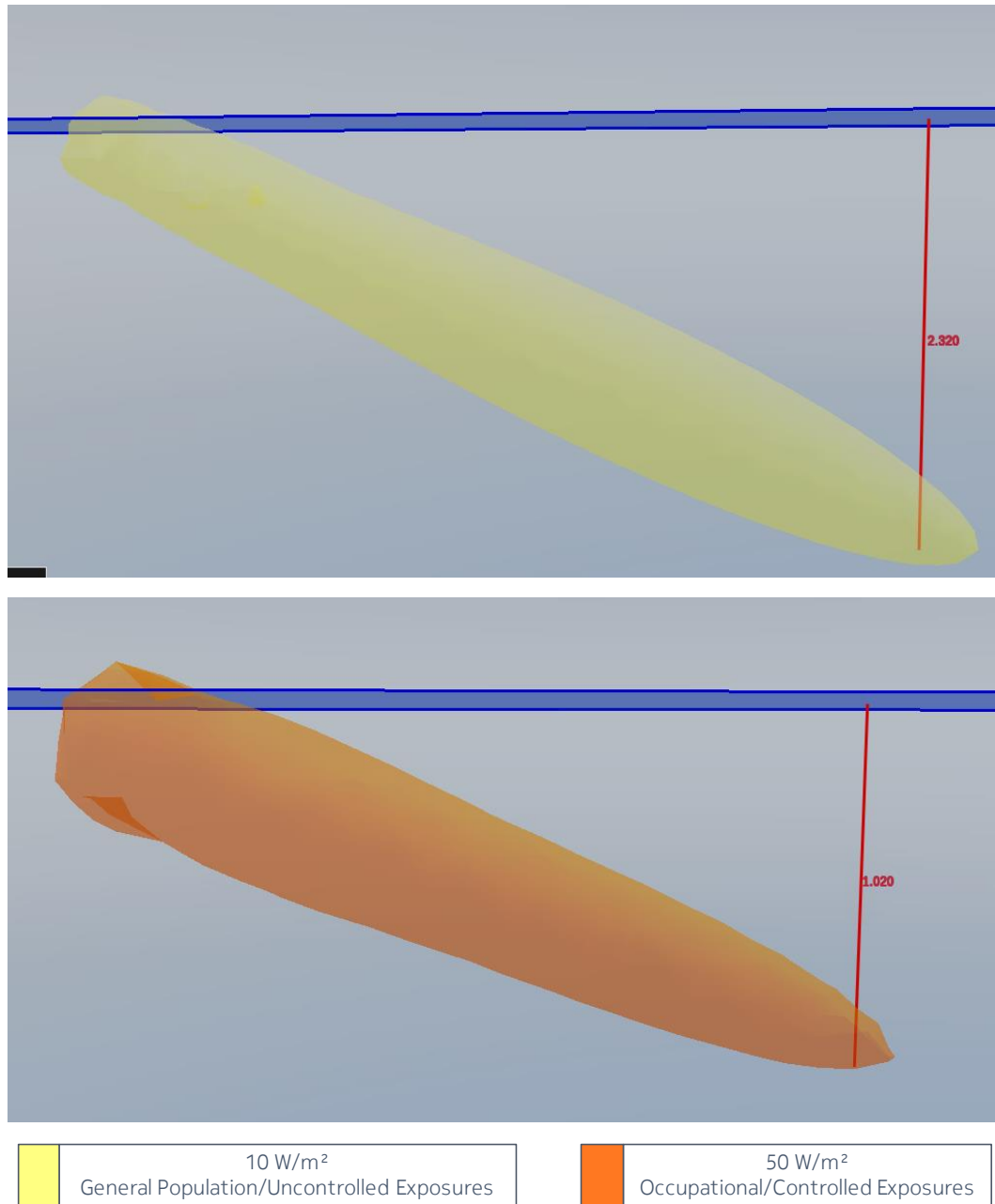
Figure 5 – Compliance distance down ( D_{d,c} ) for the time-averaged actual maximum transmitted power of 32 W and the beam oriented in azimuth = 0^\circ & elevation = -23^\circ
