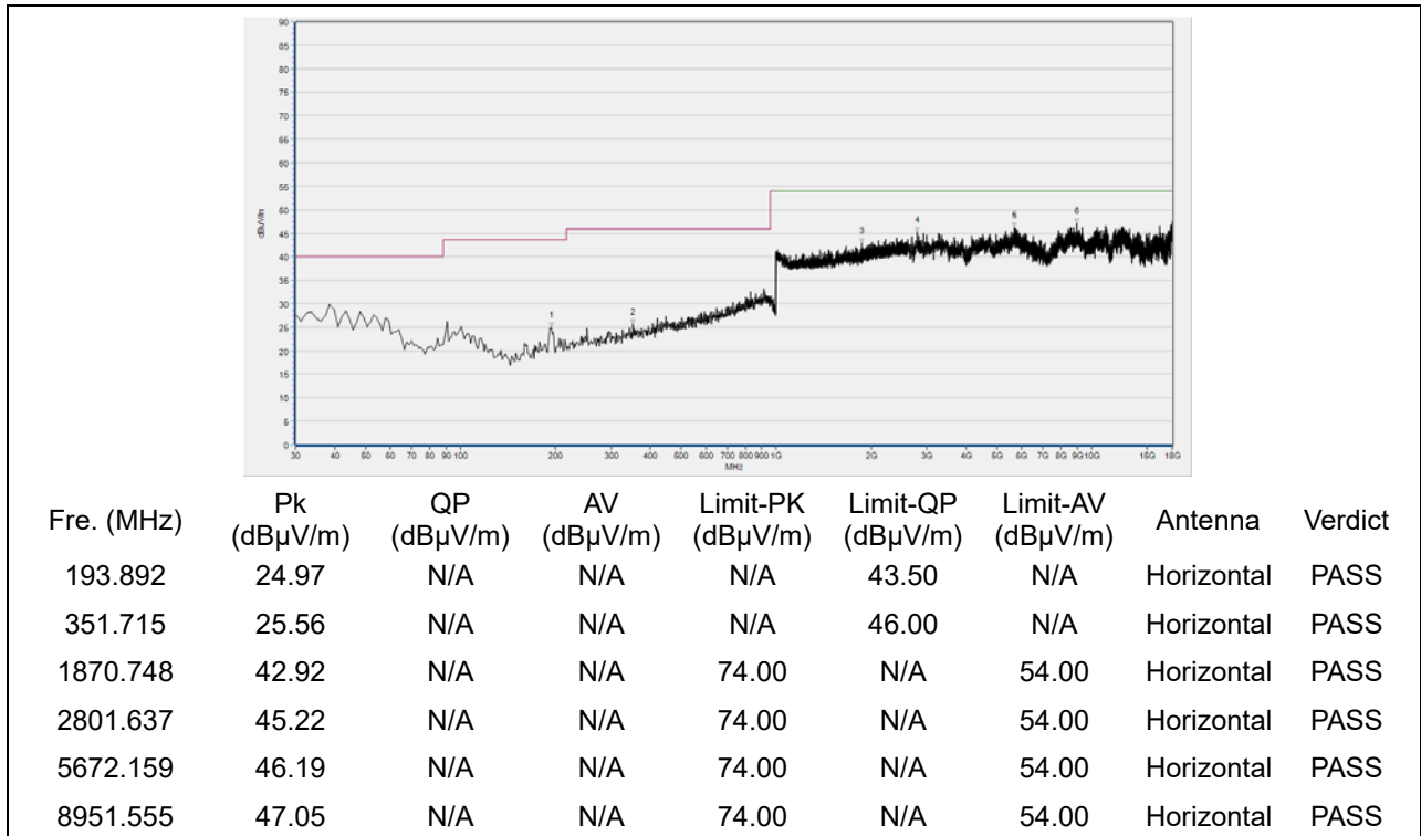
(30MHz to 18GHz, Antenna Horizontal, \pi/4 -DQPSK, channel 78)
