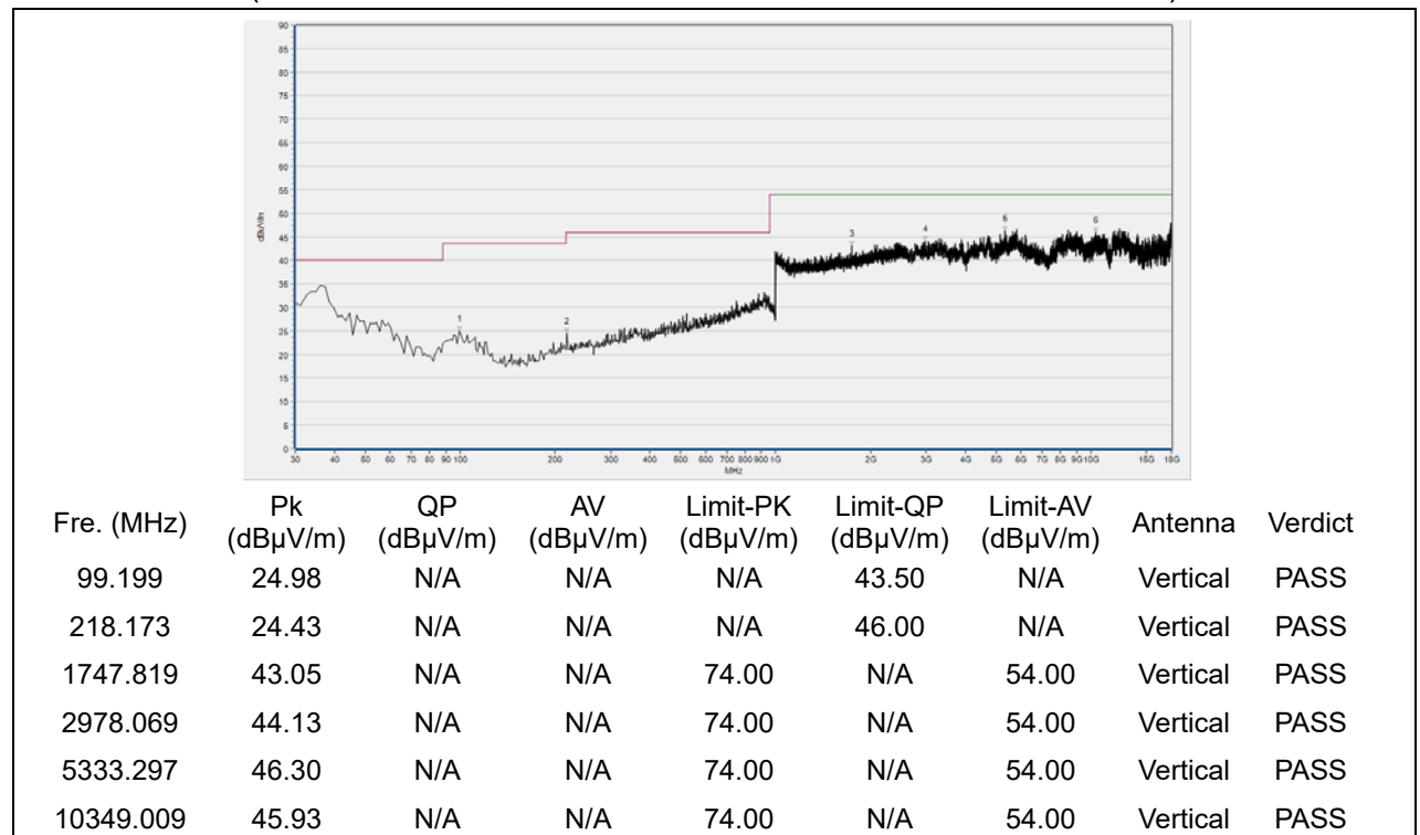
(30MHz to 18GHz, Antenna Vertical, \pi/4 -DQPSK, channel 78)
