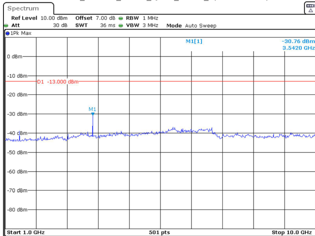
Band 12_1.4 MHz_Middle_QPSK_RB6#0_2(1GHz-10GHz)
