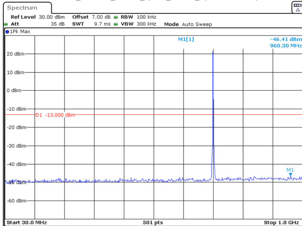
Band 12_1.4 MHz_Middle_QPSK_RB6#0_1(30MHz-1GHz)
