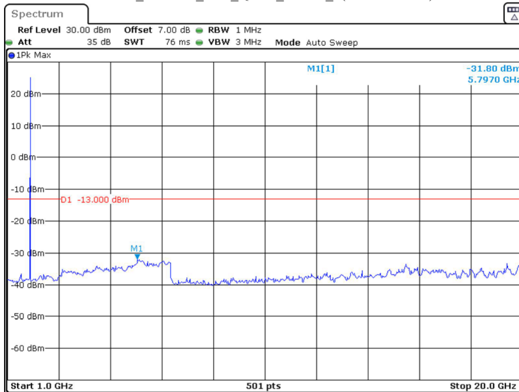
Band 2_1.4 MHz_Low_QPSK_RB6#0_2(1GHz-20GHz)
