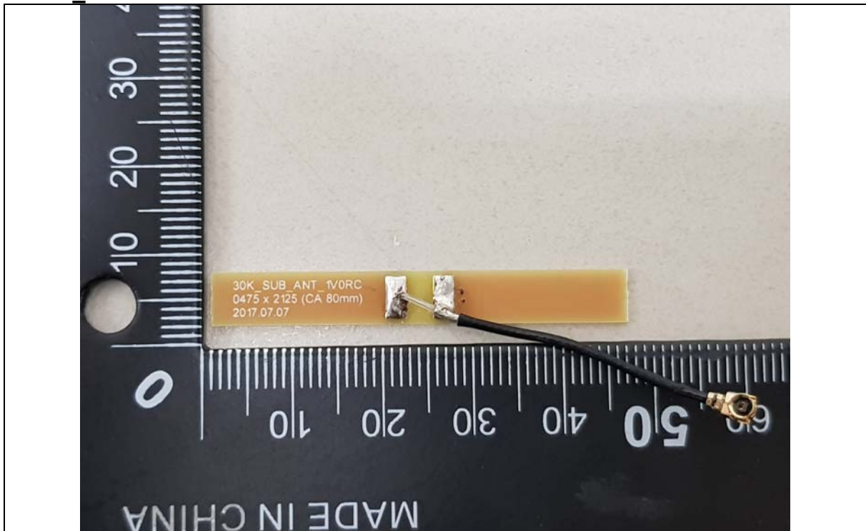
Mesh Antenna Board Rear
