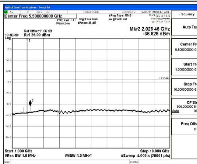
Band25-5MHz-QPSK-26065-1-0-Low-1000-10000--36.83-PASS
