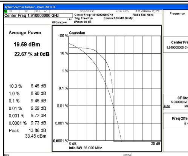
Band25-10MHz-QPSK-26640-1-0-High-9.46-9.46-13-PASS
