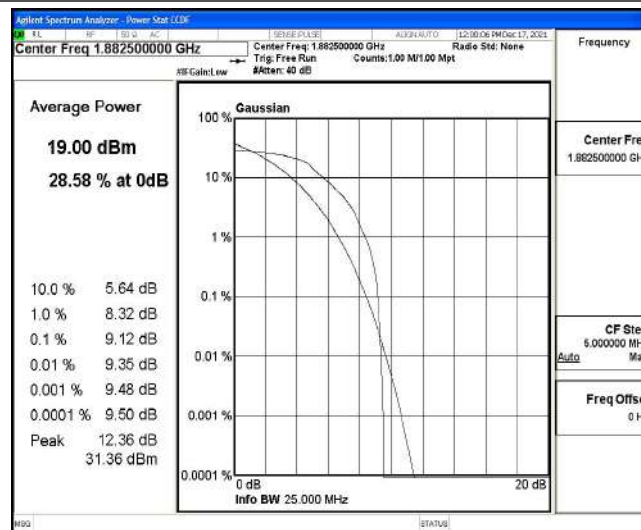
Band25-5MHz-QPSK-26365-6-0-Low-9.12-&lt;=13-PASS
