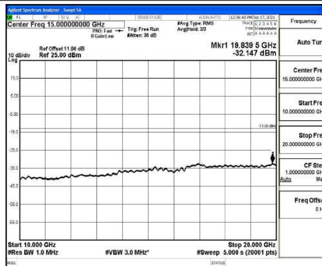
Band25-5MHz-QPSK-26665-1-0-High-10000-20000--32.15-PASS
