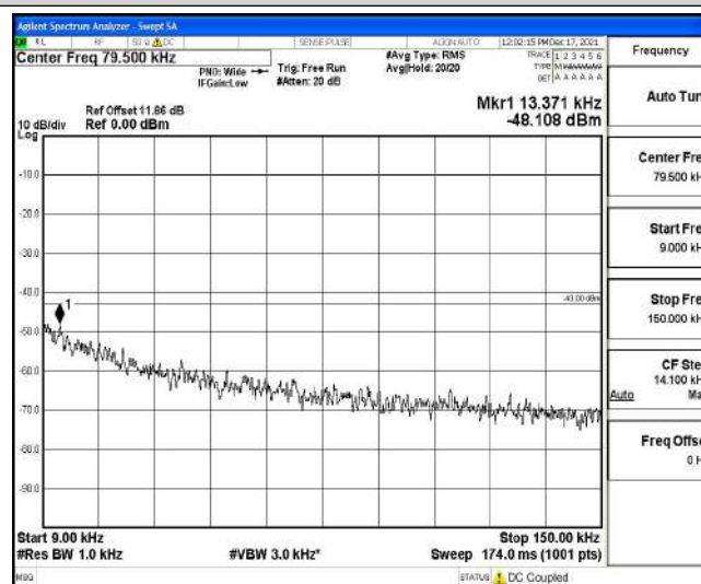
Band25-5MHz-16QAM-26065-1-0-Low-0.009-0.15--48.11-PASS
