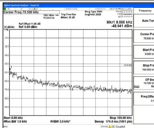
Band25-10MHz-QPSK-26090-1-0-Low-0.009-0.15--48.94-PASS
