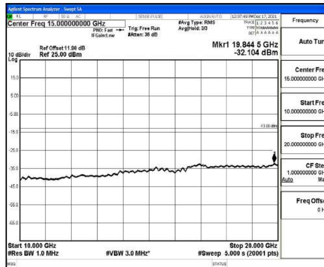
Band25-5MHz-16QAM-26665-1-0-High-10000-20000--32.1-PASS
