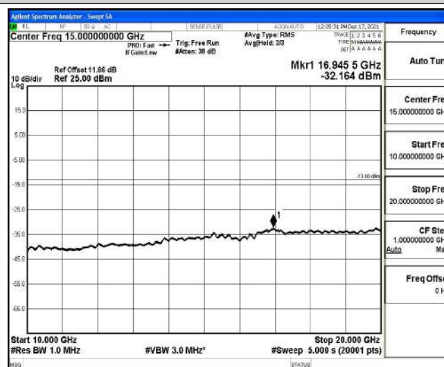
Band25-5MHz-16QAM-26365-1-0-Low-10000-20000--32.16-PASS
