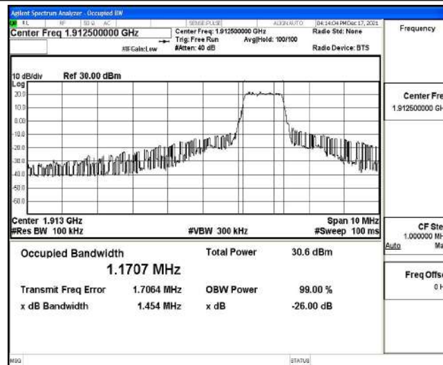
Band25-5MHz-QPSK-26665-6-0-High-1.1707-1.454-PASS
