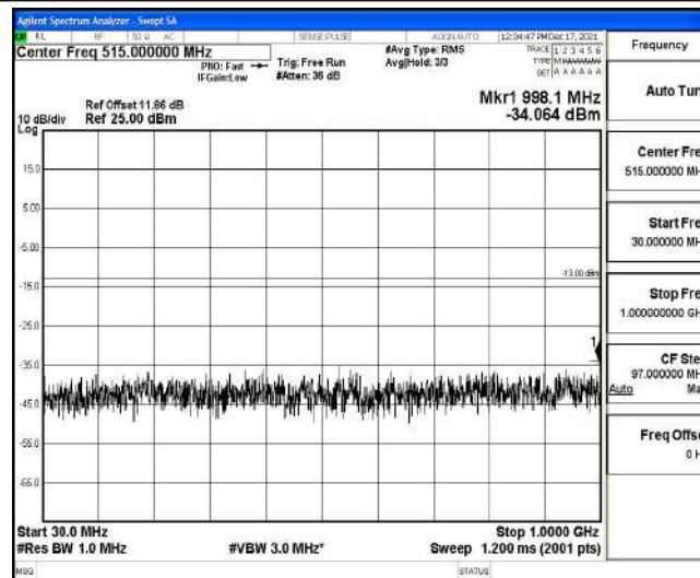
Band25-5MHz-16QAM-26365-1-0-Low-30-1000--34.06-PASS
