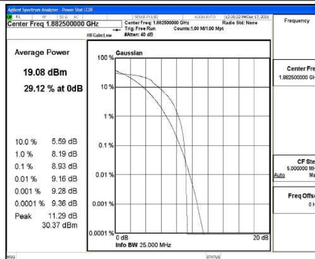
Band25-10MHz-QPSK-26365-6-0-Low-8.93-8.93-13-PASS
