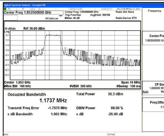
Band25-5MHz-16QAM-26065-6-0-Low-1.1737-1.665-PASS
