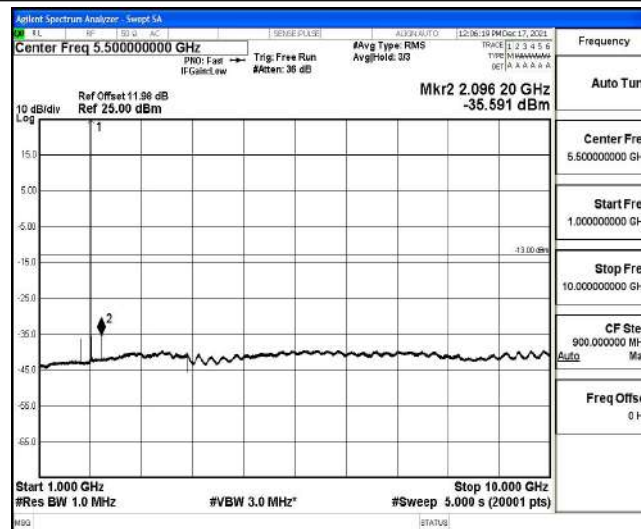
Band25-5MHz-QPSK-26665-1-0-High-1000-10000--35.59-PASS
