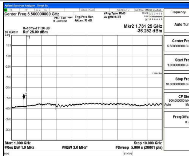
Band25-5MHz-16QAM-26665-1-0-High-1000-10000--36.25-PASS
