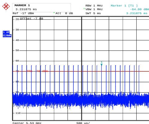
Radar #2 DFS detection threshold level
