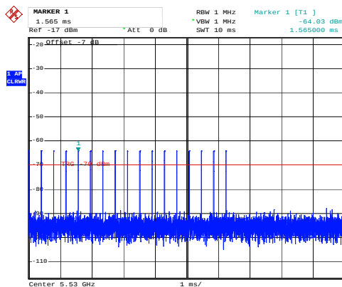
Radar #3 DFS detection threshold level
