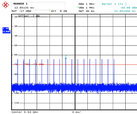
Radar #1 DFS detection threshold level
