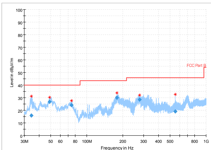
Fig.27 Radiated emission: Ch0, 30MHz~1GHz
