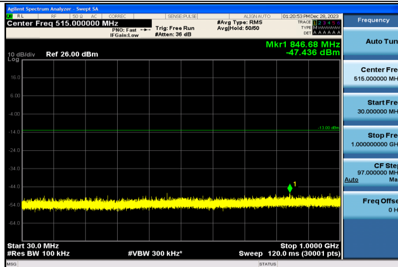
Band4-20MHz-16QAM-20175-1RB#0-30~1000MHz
