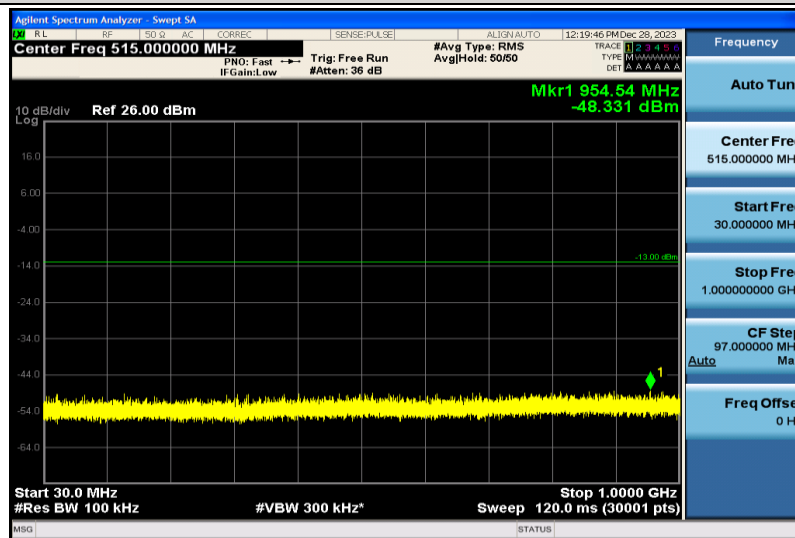
Band4-5MHz-16QAM-20375-1RB#0-30~1000MHz
