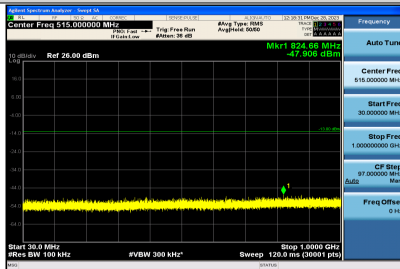
Band4-5MHz-16QAM-20175-1RB#0-30~1000MHz
