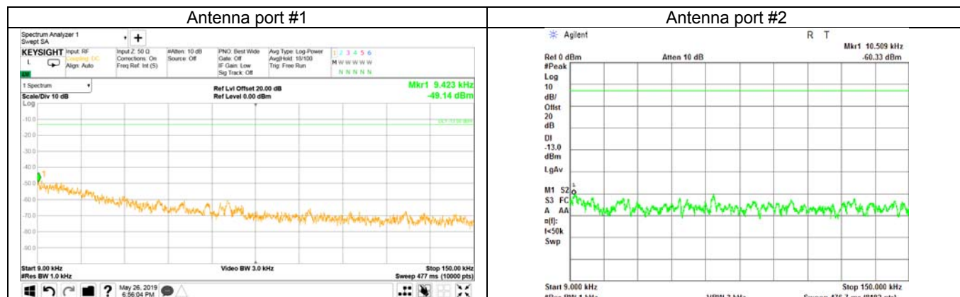
Plot 7.4.1 Spurious emission measurements in 9 - 150 kHz range at low carrier frequency
