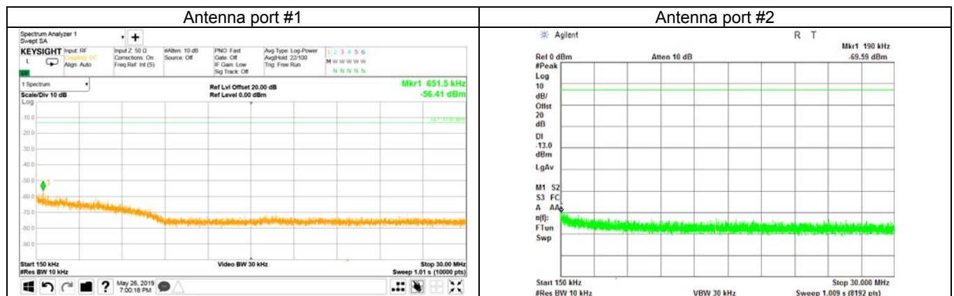
Plot 7.4.6 Spurious emission measurements in 0.15 - 30.0 MHz range at high carrier frequency
