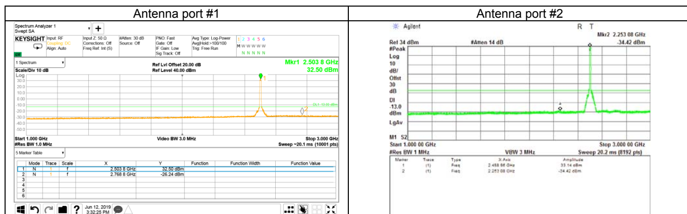
Plot 7.4.10 Spurious emission measurements in 1000 - 3000 MHz range at low carrier frequency
