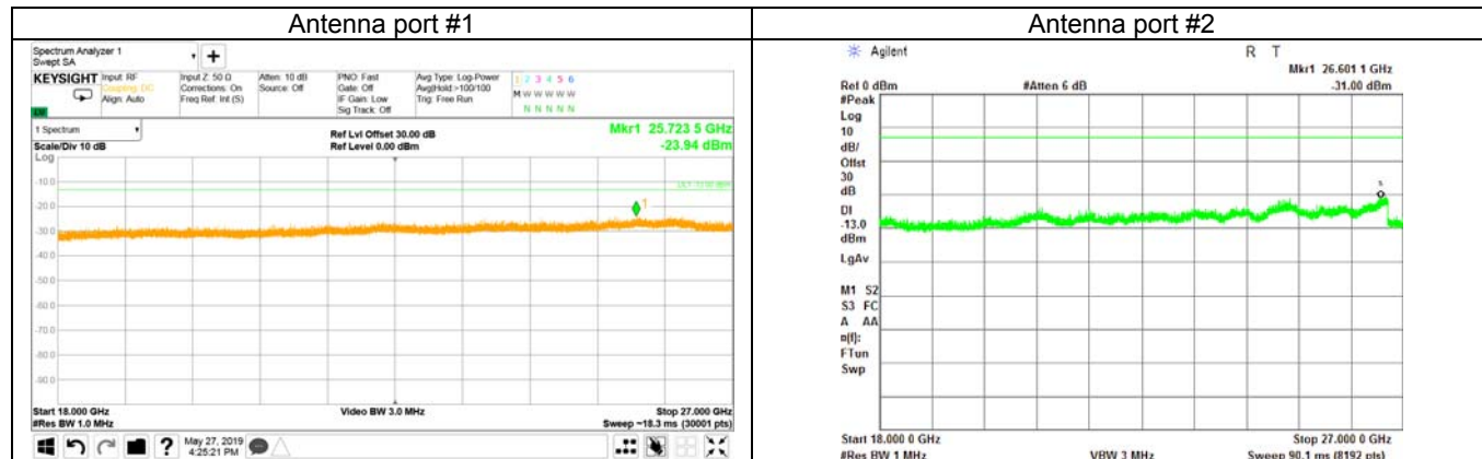
Plot 7.4.20 Spurious emission measurements in 18000 - 27000 MHz at mid carrier frequency
