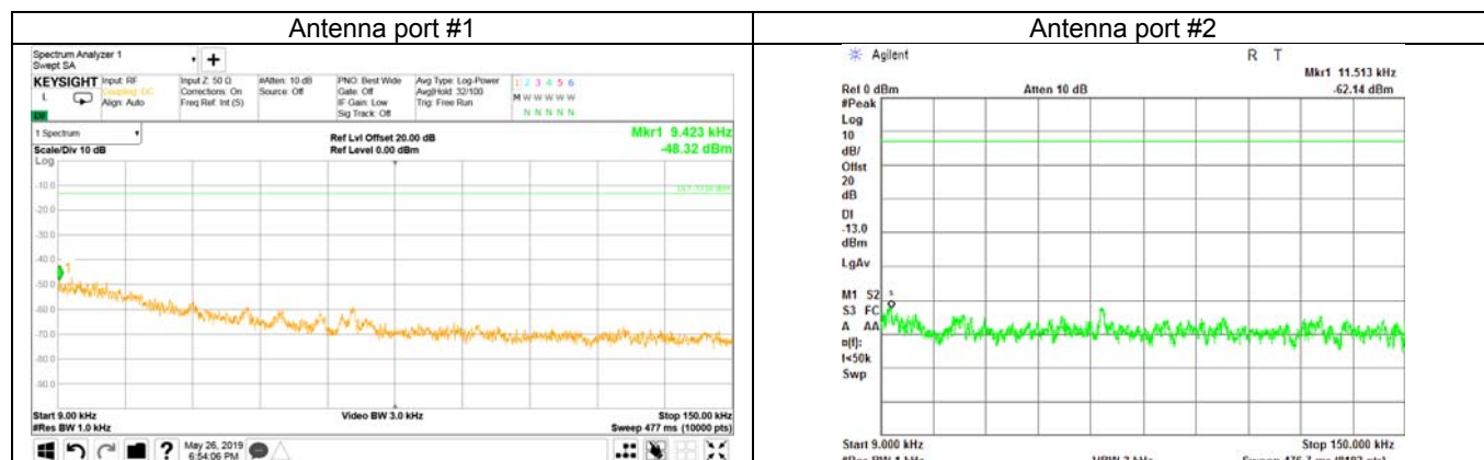
Plot 7.4.3 Spurious emission measurements in 9 - 150 kHz range at high carrier frequency
