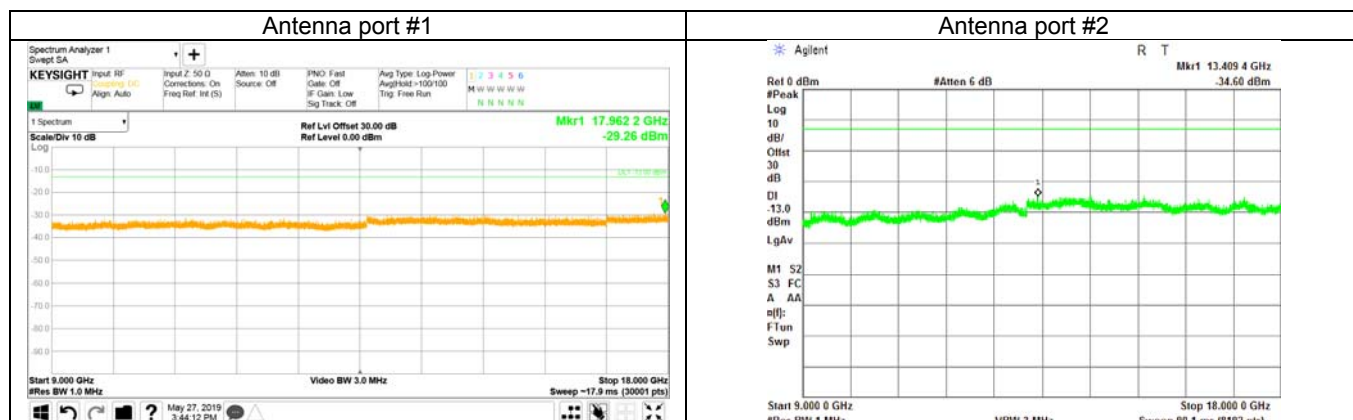
Plot 7.4.16 Spurious emission measurements in 9000 - 18000 MHz range at low carrier frequency
