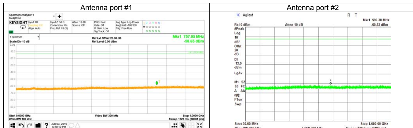
Plot 7.4.7 Spurious emission measurements in 30 - 1000 MHz range at low carrier frequency
