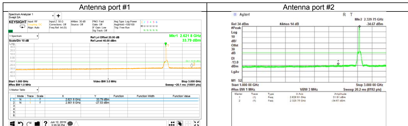
Plot 7.4.11 Spurious emission measurements in 1000 - 3000 MHz range at mid carrier frequency
