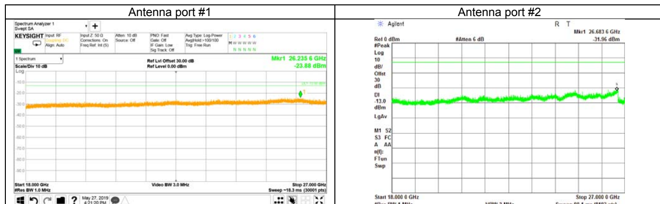
Plot 7.4.19 Spurious emission measurements in 18000 - 27000 MHz range at low carrier frequency
