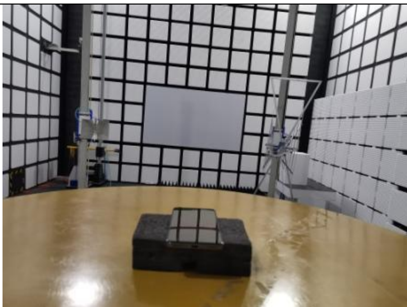
Spurious Radiated Emissions Test setup
