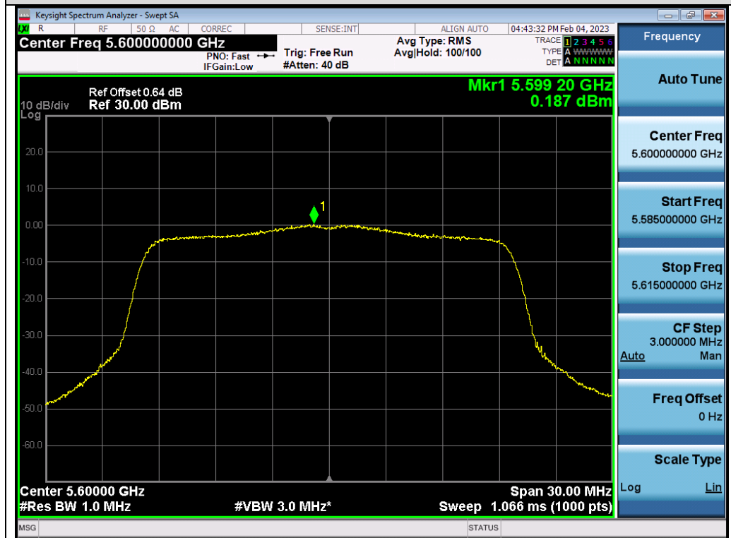
Test_Graph_802.11ax20_ANT2_5600_MCS0_PSD
