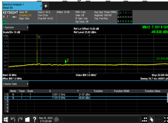
N48(10M)_DFT-s- OFDM BPSK Edge 1RB Left Low CH
