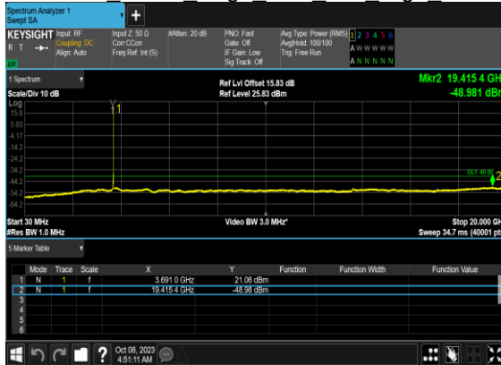
N48(10M)_DFT-s-OFDM BPSK Edge 1RB Left High CH
