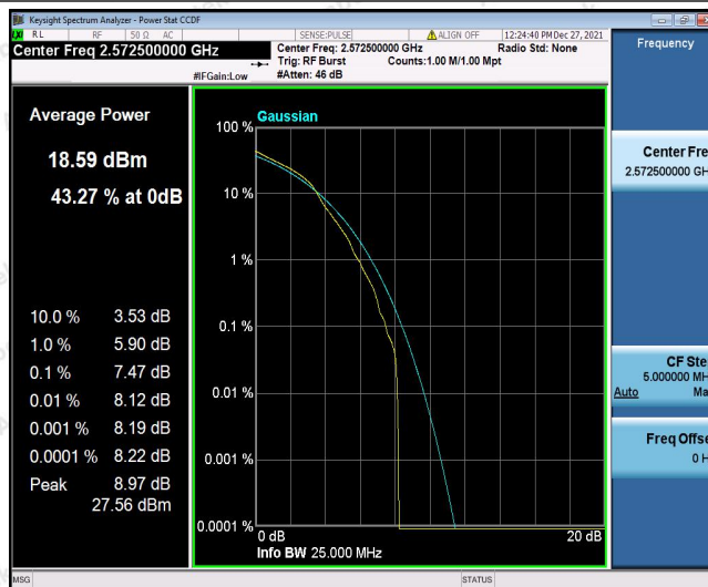
Band41-15MHz-16QAM-40415-75RB#0
