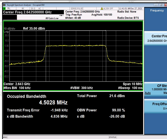
Band41-5MHz-16QAM-40365-25RB#0
