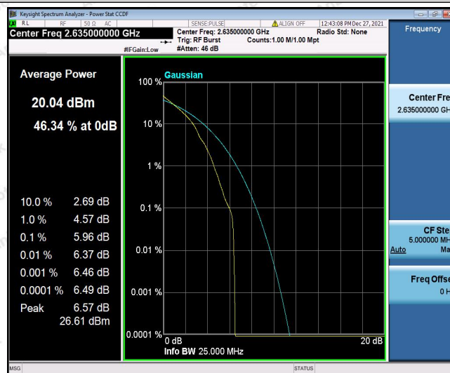
Band41-20MHz-QPSK-41040-100RB#0
