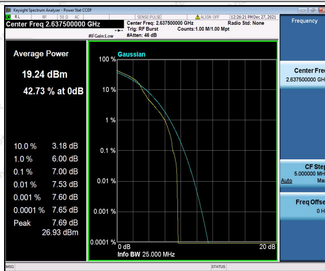
Band41-15MHz-16QAM-41065-75RB#0
