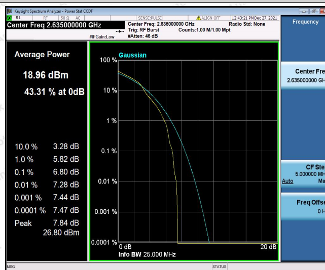
Band41-20MHz-16QAM-41040-100RB#0
