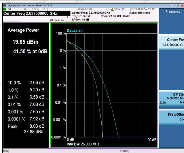
Band41-15MHz-16QAM-40415-1RB#0
