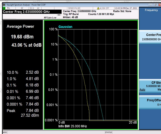
Band41-20MHz-16QAM-40440-1RB#0
