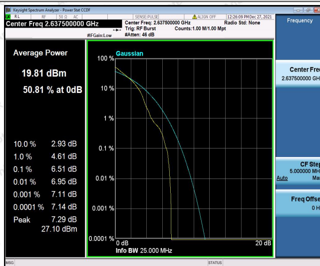
Band41-15MHz-QPSK-41065-75RB#0
