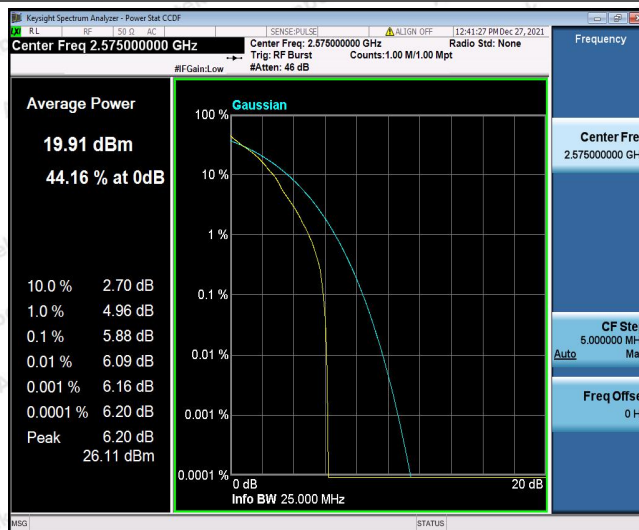
Band41-20MHz-QPSK-40440-100RB#0
