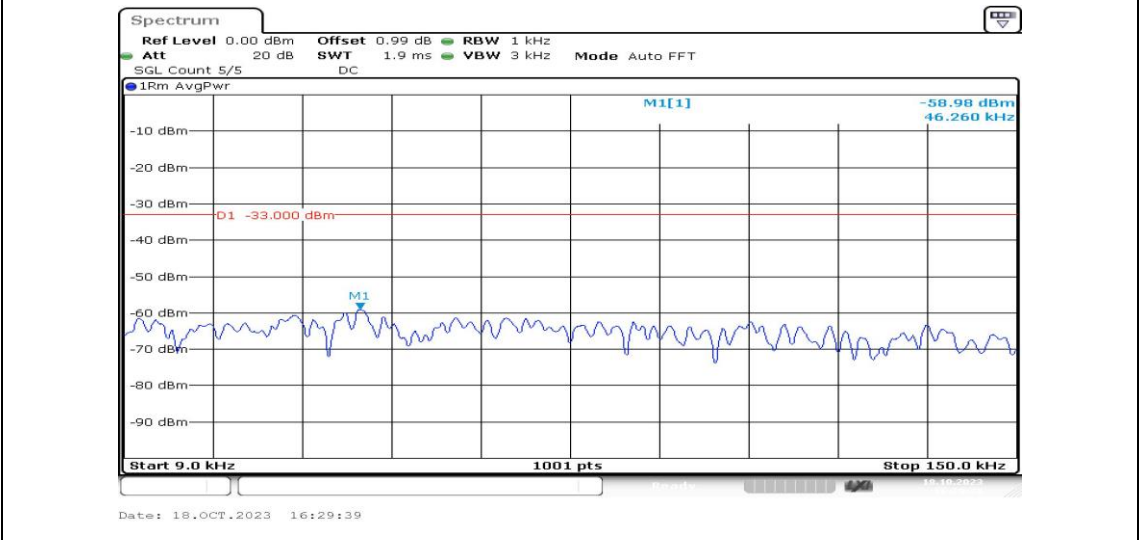
Band25-3MHz-QPSK-26055-1RB#0-Range1:0.009-0.15MHz-PASS
