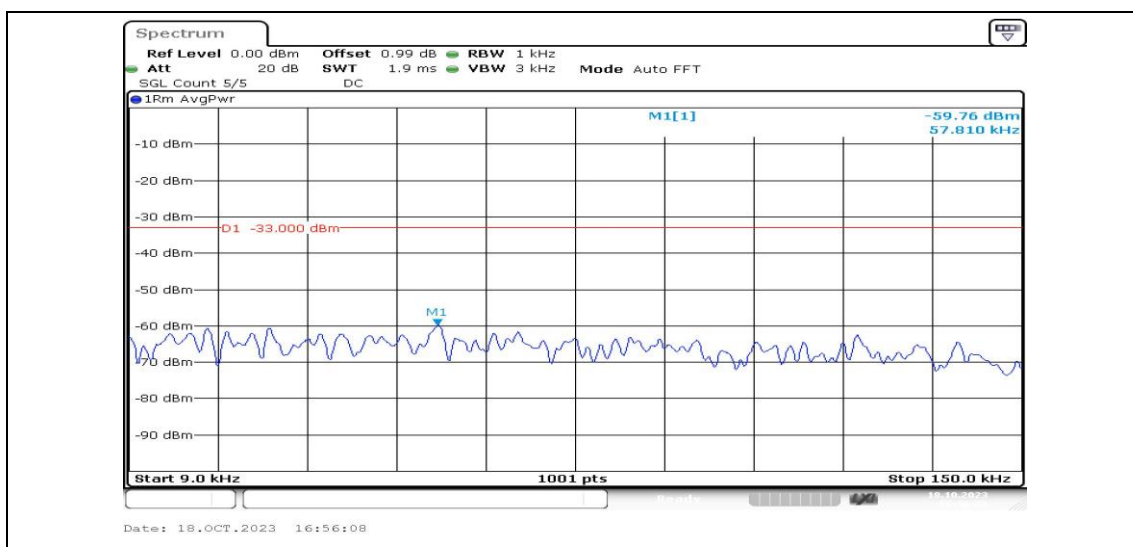
Band25-5MHz-QPSK-26365-1RB#0-Range1:0.009~0.15MHz-PASS
