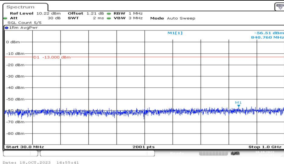
Band25-5MHz-16QAM-26065-1RB#0-Range3:30~1000MHz-PASS
