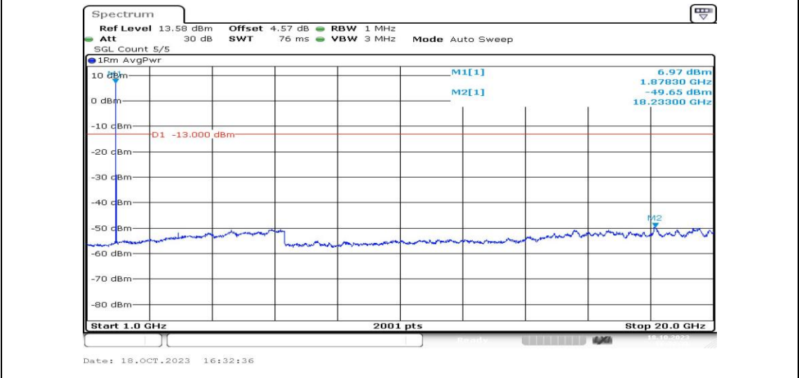
Band25-3MHz-16QAM-26365-1RB#0-Range4:1000~20000MHz-PASS
