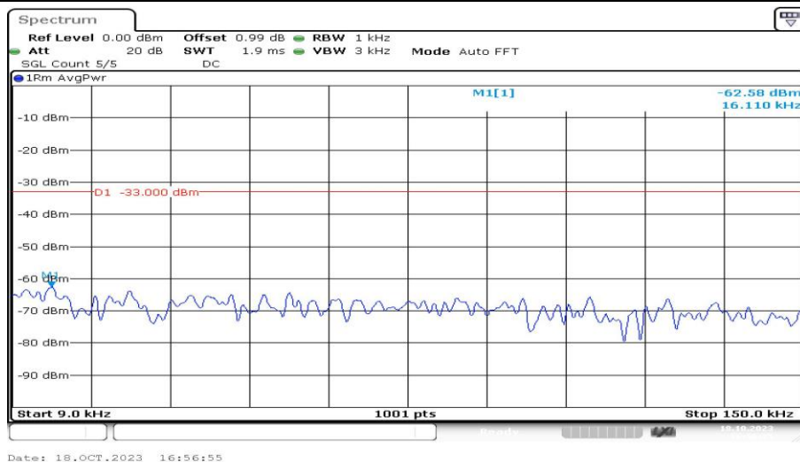
Band25-5MHz-16QAM-26365-1RB#0-Range1:0.009~0.15MHz-PASS
