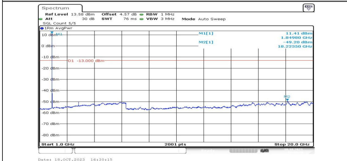
Band25-3MHz-QPSK-26055-1RB#0-Range4:1000~20000MHz-PASS
