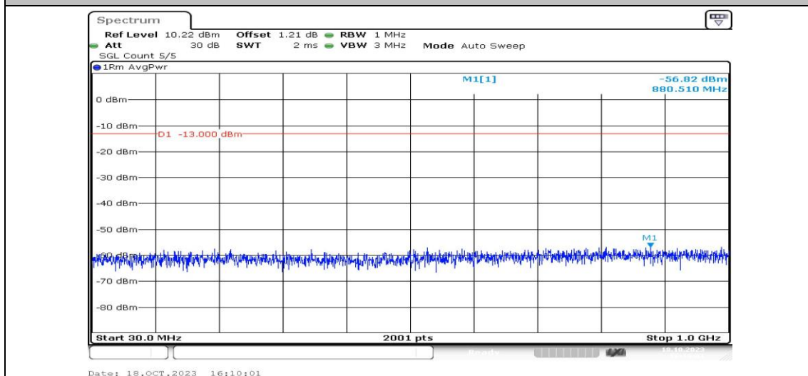
Band25-1.4MHz-16QAM-26683-1RB#0-Range3:30~1000MHz-PASS
