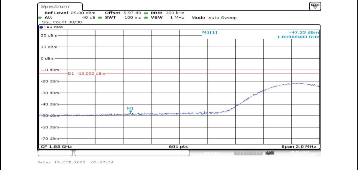
Band25-15MHz-16QAM-26115-1RB#74-PASS
