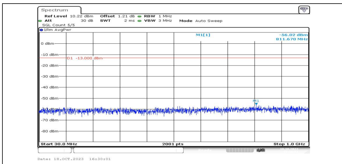
Band25-3MHz-QPSK-26055-1RB#0-Range3:30~1000MHz-PASS
