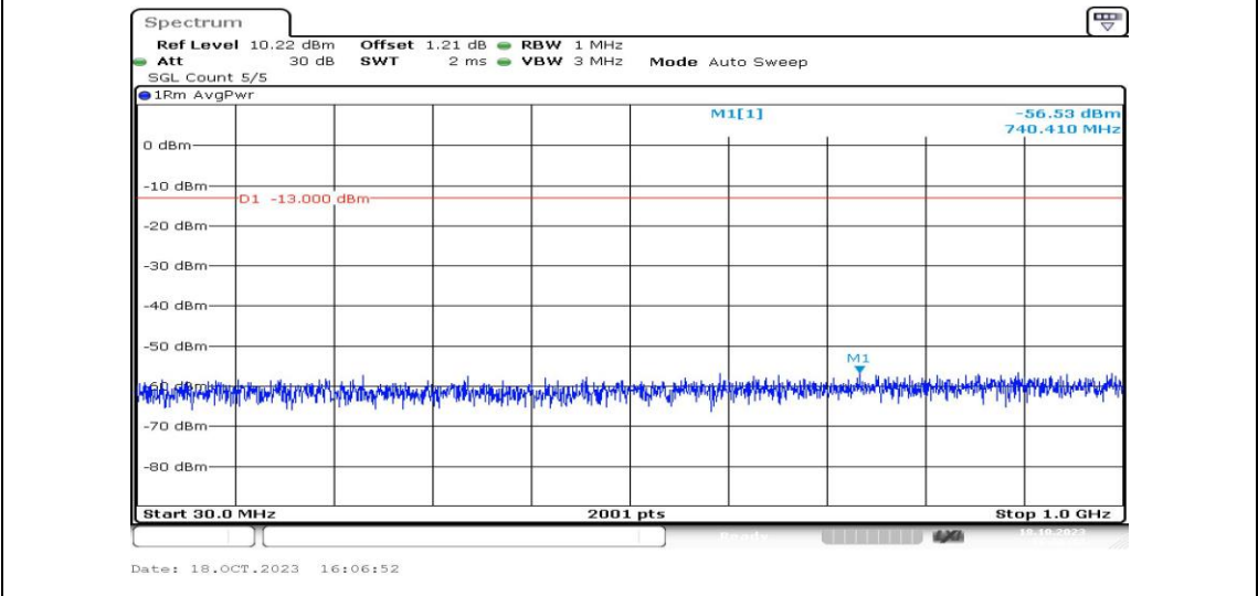
Band25-1.4MHz-16QAM-26047-1RB#0-Range3:30~1000MHz-PASS
