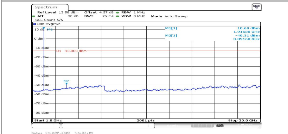
Band25-3MHz-QPSK-26675-1RB#0-Range4:1000~20000MHz-PASS
