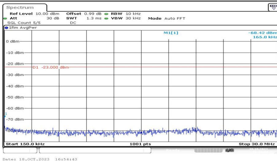
Band25-5MHz-QPSK-26065-1RB#0-Range2:0.15~30MHz-PASS
