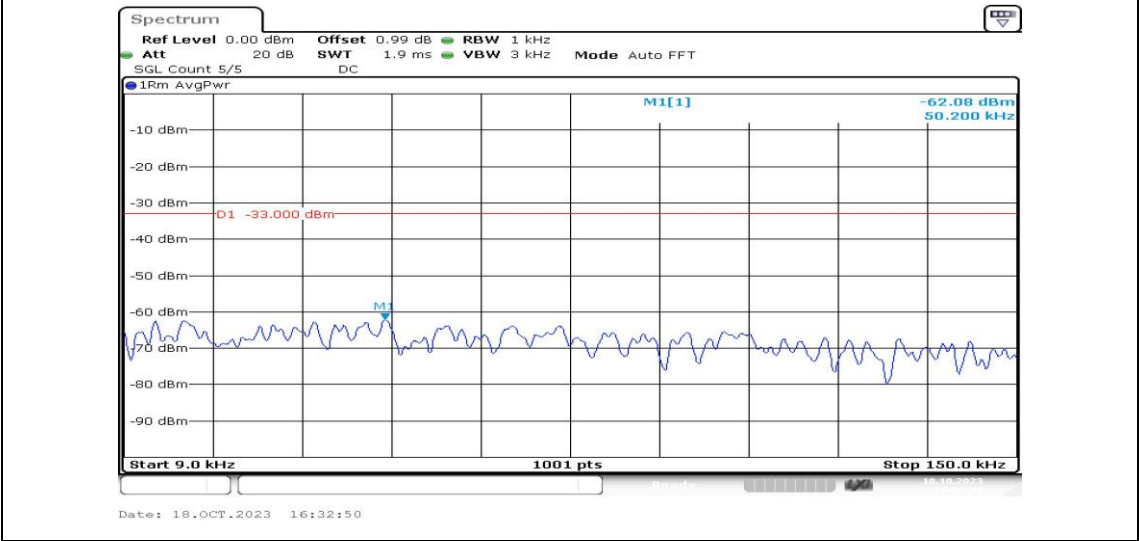
Band25-3MHz-QPSK-26675-1RB#0-Range1:0.009~0.15MHz-PASS
