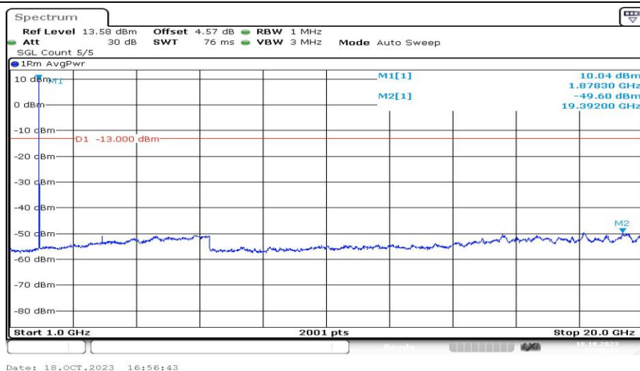
Band25-5MHz-QPSK-26365-1RB#0-Range4:1000~20000MHz-PASS
