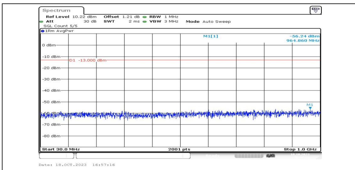
Band25-5MHz-16QAM-26365-1RB#0-Range3:30~1000MHz-PASS
