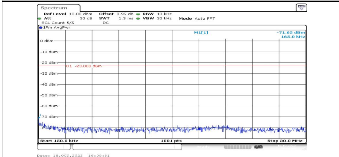
Band25-1.4MHz-16QAM-26683-1RB#0-Range2:0.15~30MHz-PASS
