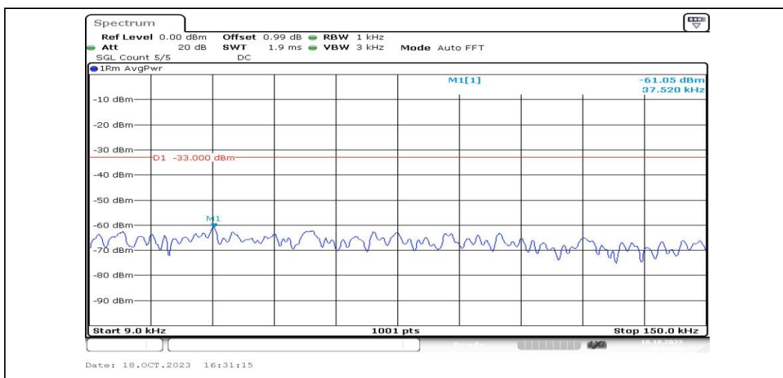
Band25-3MHz-QPSK-26365-1RB#0-Range1:0.009~0.15MHz-PASS
