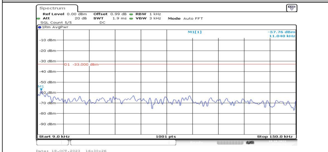
Band25-3MHz-16QAM-26055-1RB#0-Range1:0.009~0.15MHz-PASS
