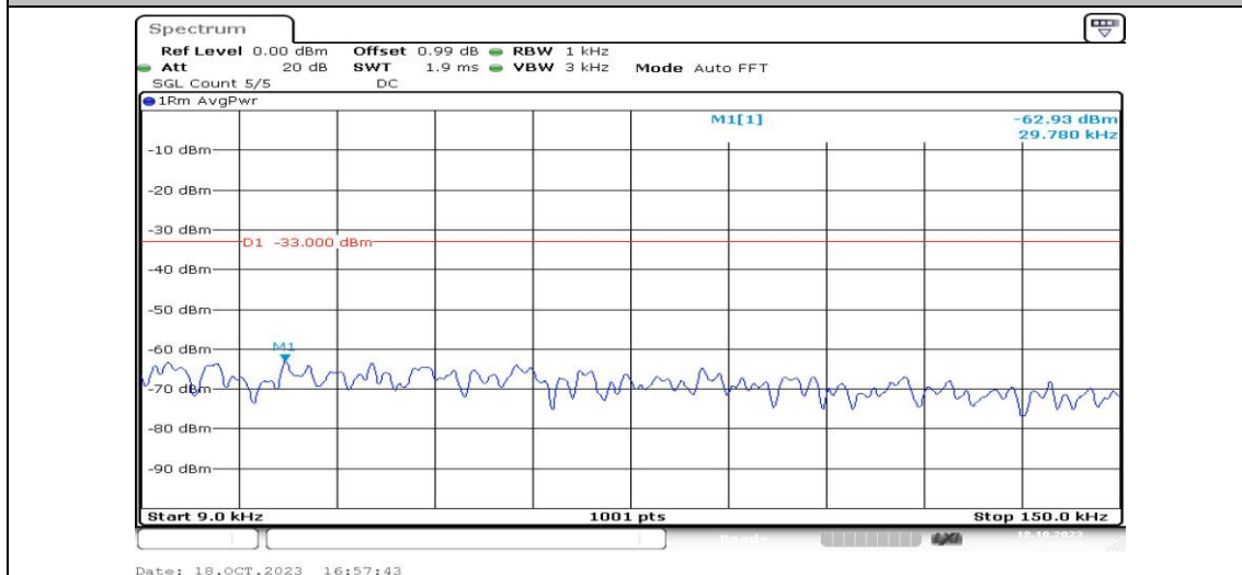
Band25-5MHz-QPSK-26665-1RB#0-Range1:0.009~0.15MHz-PASS
