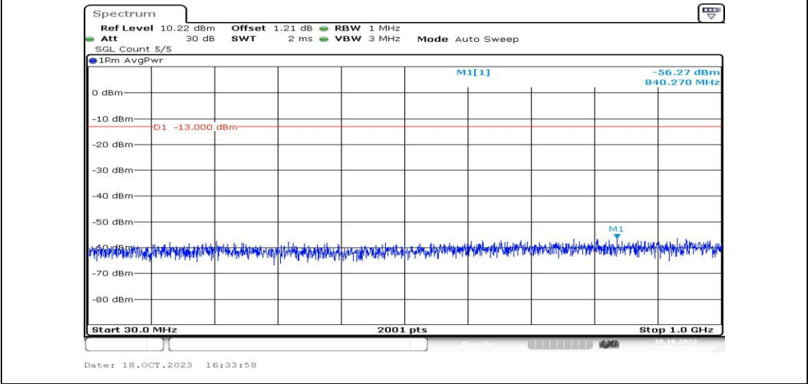
Band25-3MHz-16QAM-26675-1RB#0-Range3:30~1000MHz-PASS
