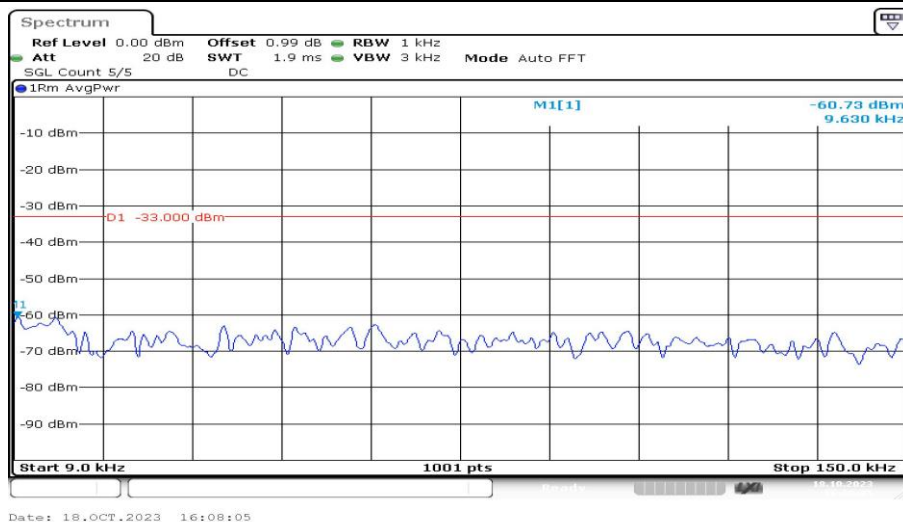
Band25-1.4MHz-16QAM-26365-1RB#0-Range1:0.009~0.15MHz-PASS
