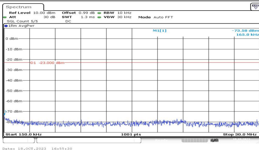
Band25-5MHz-16QAM-26065-1RB#0-Range2:0.15~30MHz-PASS
