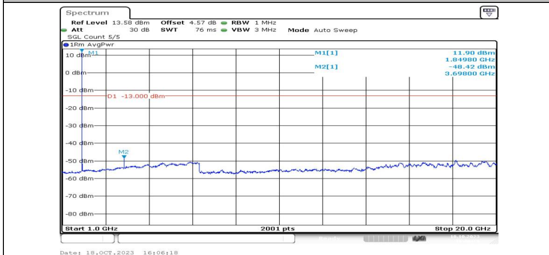
Band25-1.4MHz-QPSK-26047-1RB#0-Range4:1000~20000MHz-PASS
