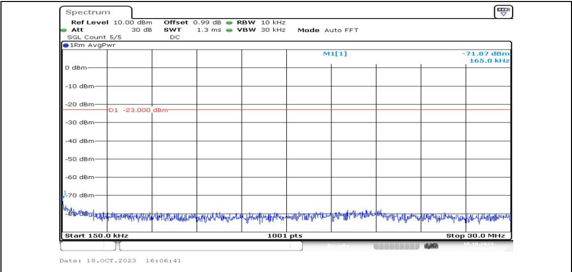
Band25-1.4MHz-16QAM-26047-1RB#0-Range2:0.15~30MHz-PASS
