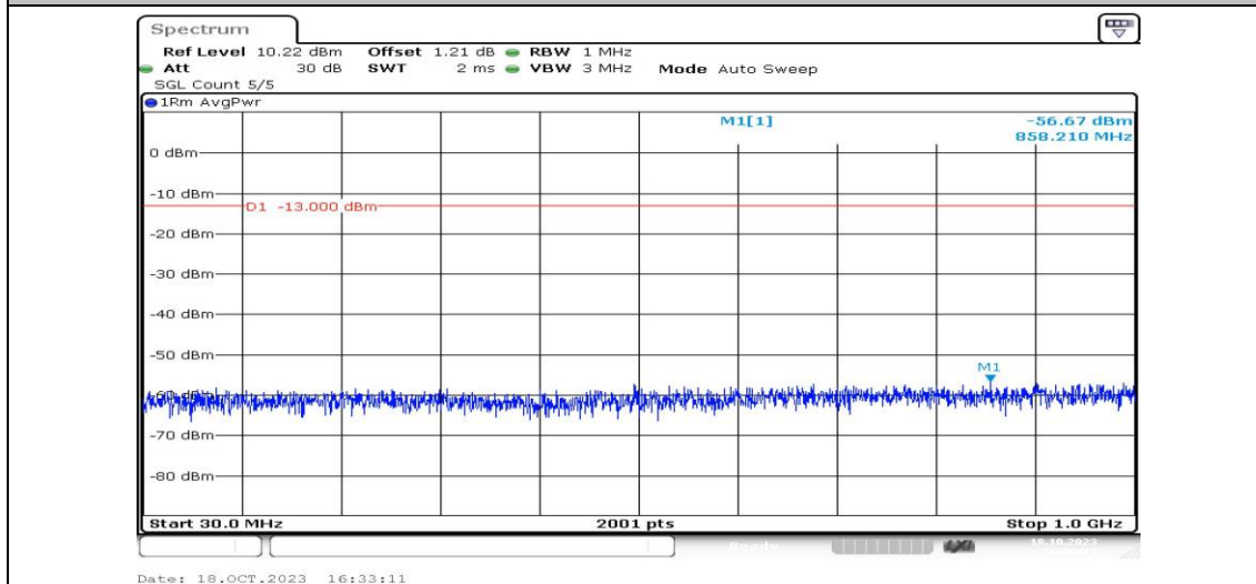
Band25-3MHz-QPSK-26675-1RB#0-Range3:30~1000MHz-PASS
