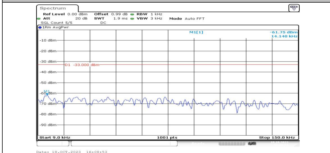
Band25-1.4MHz-QPSK-26683-1RB#0-Range1:0.009~0.15MHz-PASS
