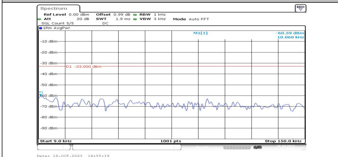
Band25-5MHz-16QAM-26065-1RB#0-Range1:0.009~0.15MHz-PASS
