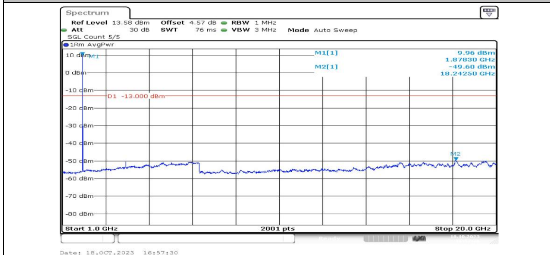
Band25-5MHz-16QAM-26365-1RB#0-Range4:1000~20000MHz-PASS
