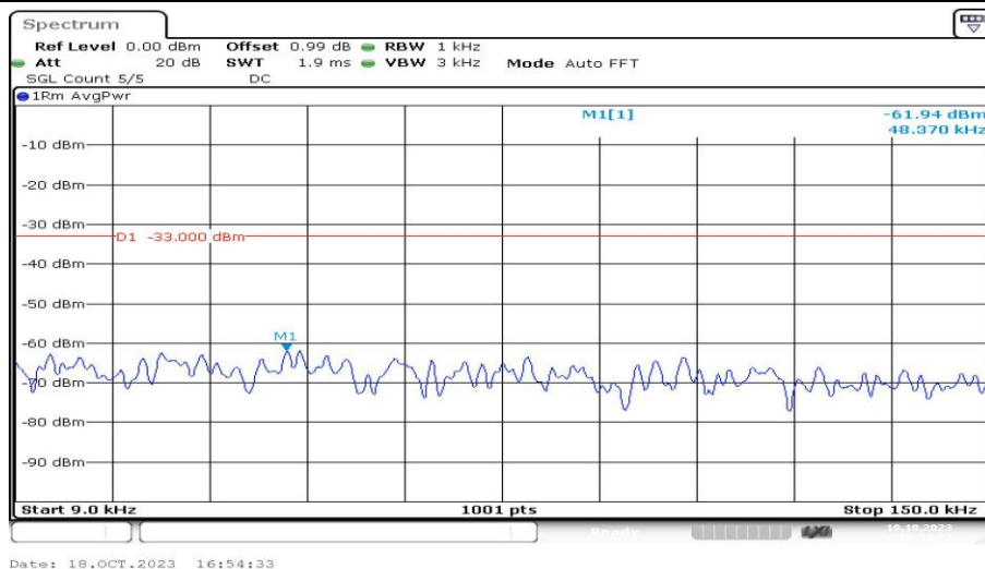
Band25-5MHz-QPSK-26065-1RB#0-Range1:0.009~0.15MHz-PASS
