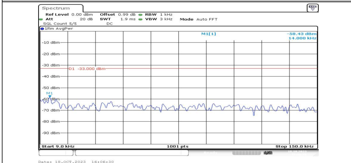
Band25-1.4MHz-16QAM-26047-1RB#0-Range1:0.009~0.15MHz-PASS
