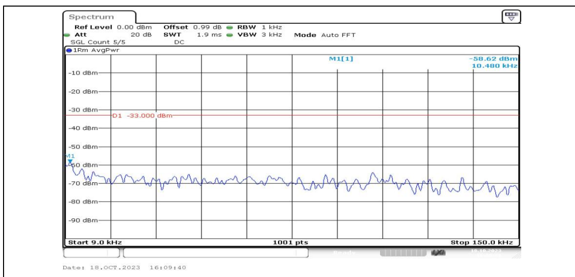
Band25-1.4MHz-16QAM-26683-1RB#0-Range1:0.009~0.15MHz-PASS
