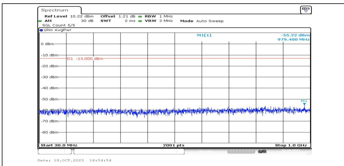
Band25-5MHz-QPSK-26065-1RB#0-Range3:30~1000MHz-PASS
