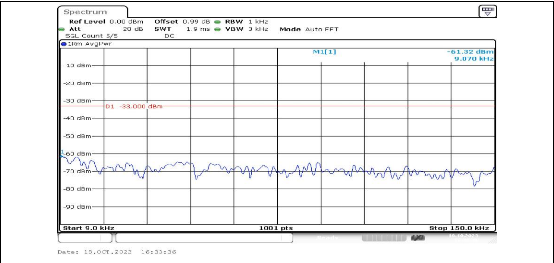
Band25-3MHz-16QAM-26675-1RB#0-Range1:0.009~0.15MHz-PASS
