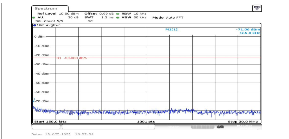
Band25-5MHz-QPSK-26665-1RB#0-Range2:0.15~30MHz-PASS
