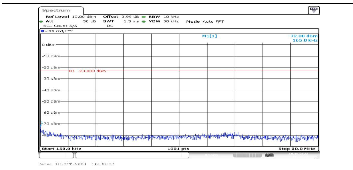
Band25-3MHz-16QAM-26055-1RB#0-Range2:0.15~30MHz-PASS
