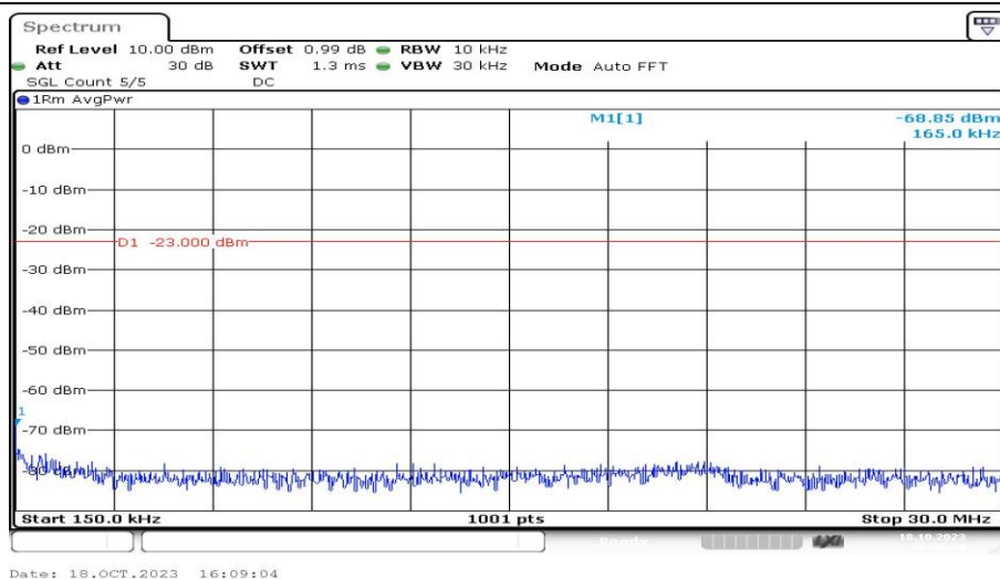
Band25-1.4MHz-QPSK-26683-1RB#0-Range2:0.15~30MHz-PASS
