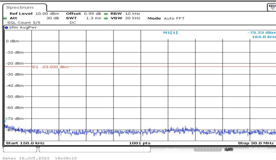
Band25-1.4MHz-16QAM-26365-1RB#0-Range2:0.15~30MHz-PASS
