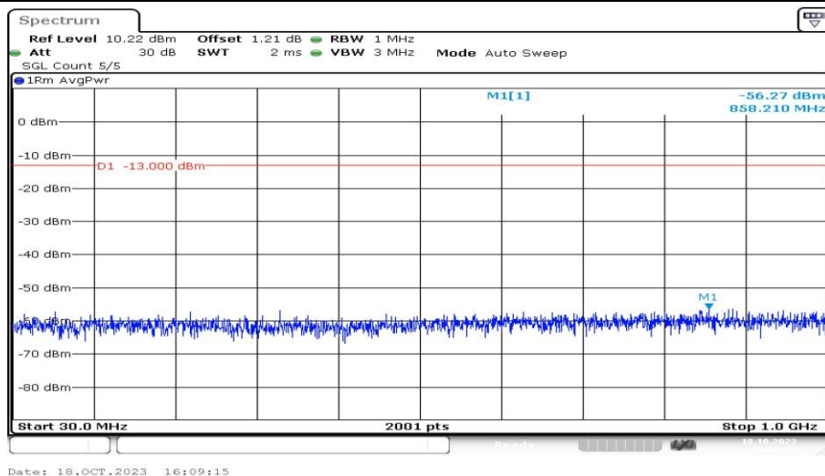
Band25-1.4MHz-QPSK-26683-1RB#0-Range3:30~1000MHz-PASS
