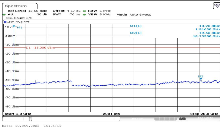
Band25-3MHz-16QAM-26675-1RB#0-Range4:1000~20000MHz-PASS
