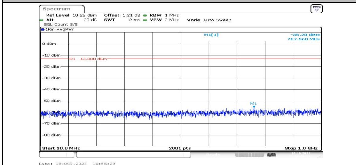
Band25-5MHz-QPSK-26365-1RB#0-Range3:30~1000MHz-PASS
