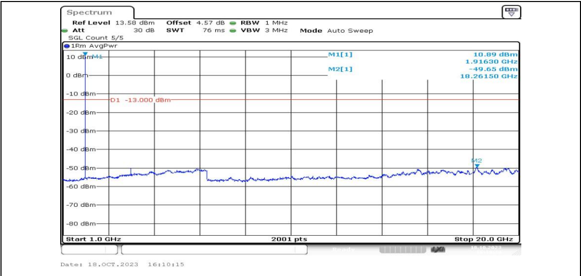
Band25-1.4MHz-16QAM-26683-1RB#0-Range4:1000-20000MHz-PASS
