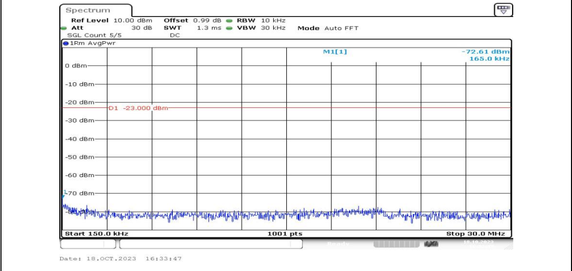
Band25-3MHz-16QAM-26675-1RB#0-Range2:0.15~30MHz-PASS
