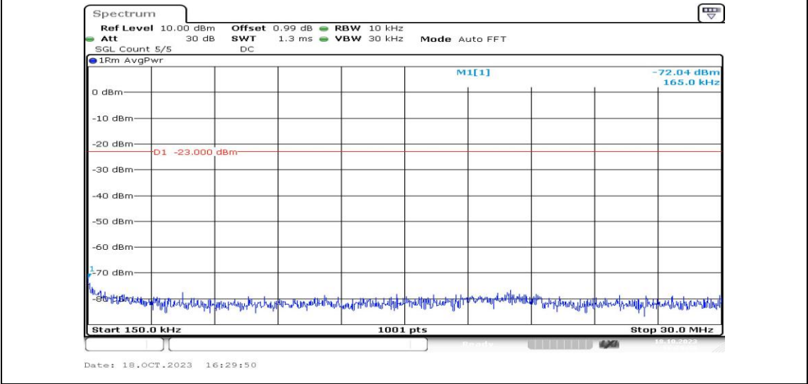
Band25-3MHz-QPSK-26055-1RB#0-Range2:0.15-30MHz-PASS
