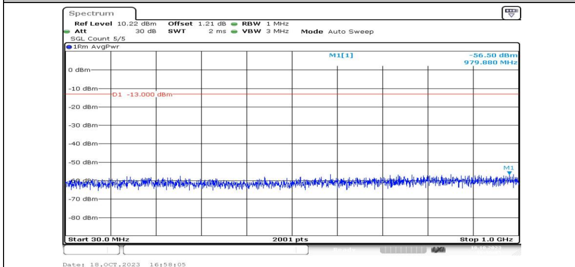
Band25-5MHz-QPSK-26665-1RB#0-Range3:30~1000MHz-PASS
