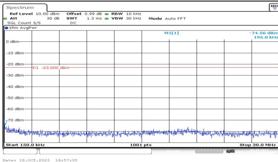
Band25-5MHz-16QAM-26365-1RB#0-Range2:0.15~30MHz-PASS
