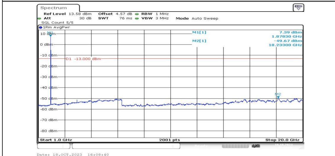
Band25-1.4MHz-16QAM-26365-1RB#0-Range4:1000~20000MHz-PASS
