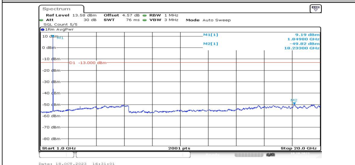
Band25-3MHz-16QAM-26055-1RB#0-Range4:1000~20000MHz-PASS
