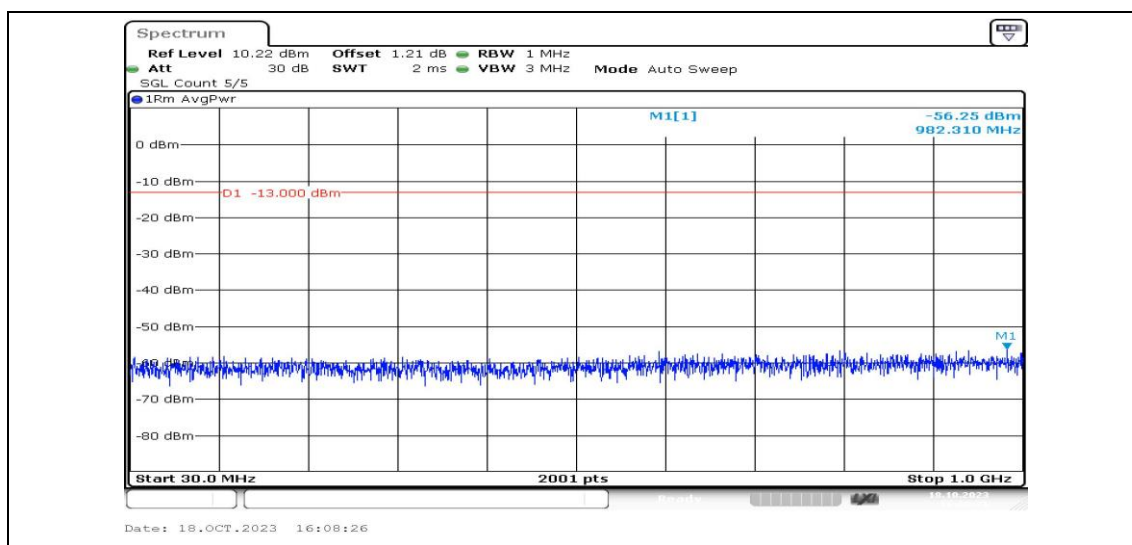
Band25-1.4MHz-16QAM-26365-1RB#0-Range3:30~1000MHz-PASS
