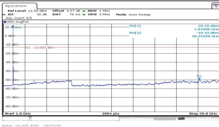
Band25-5MHz-16QAM-26065-1RB#0-Range4:1000~20000MHz-PASS
