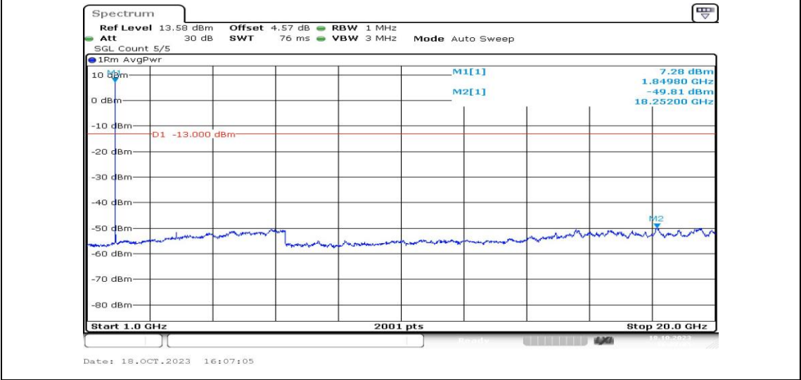
Band25-1.4MHz-16QAM-26047-1RB#0-Range4:1000~20000MHz-PASS
