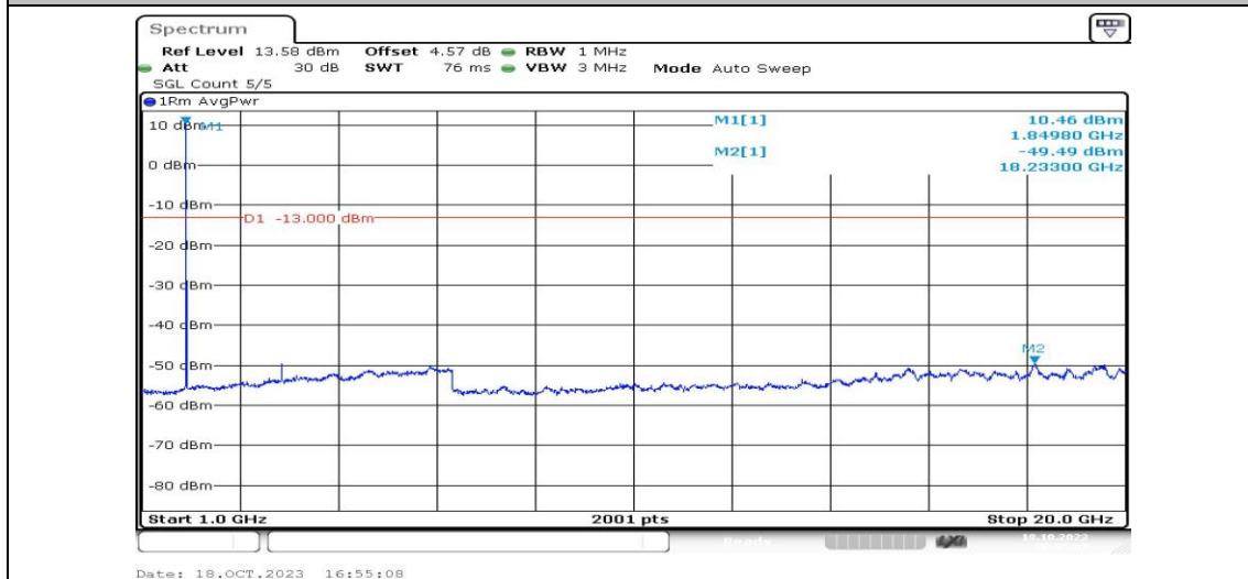
Band25-5MHz-QPSK-26065-1RB#0-Range4:1000~20000MHz-PASS
