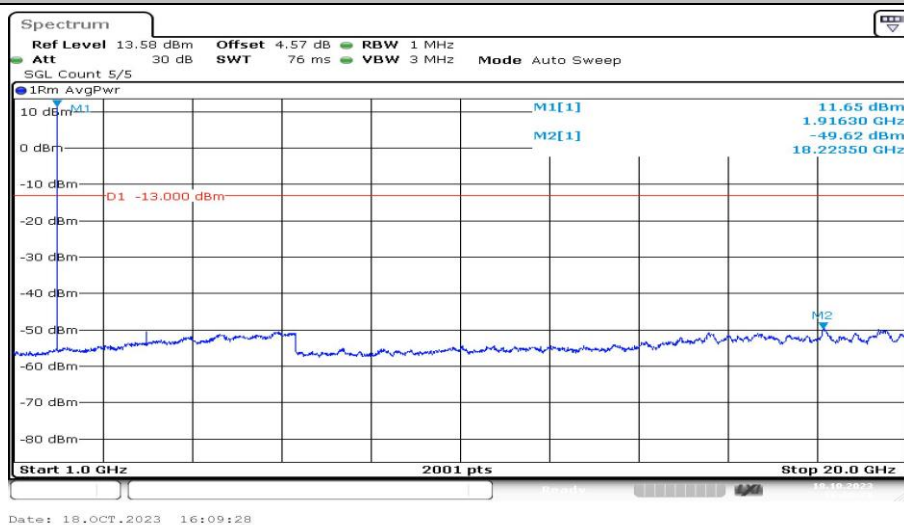
Band25-1.4MHz-QPSK-26683-1RB#0-Range4:1000~20000MHz-PASS
