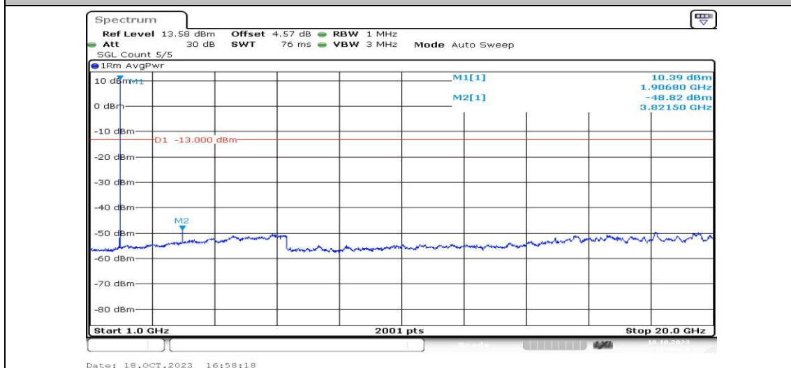
Band25-5MHz-QPSK-26665-1RB#0-Range4:1000~20000MHz-PASS
