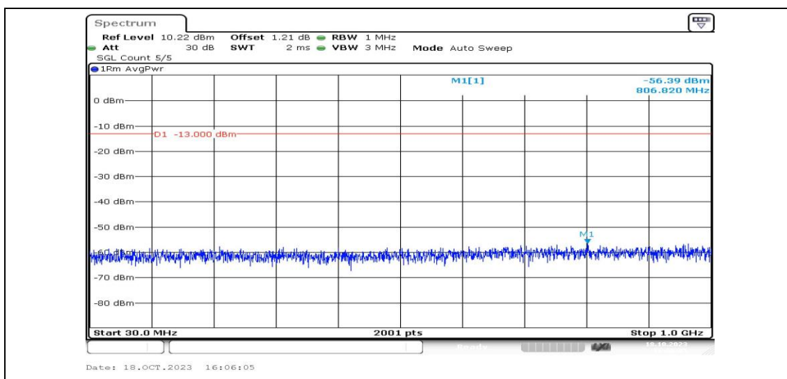
Band25-1.4MHz-QPSK-26047-1RB#0-Range3:30~1000MHz-PASS
