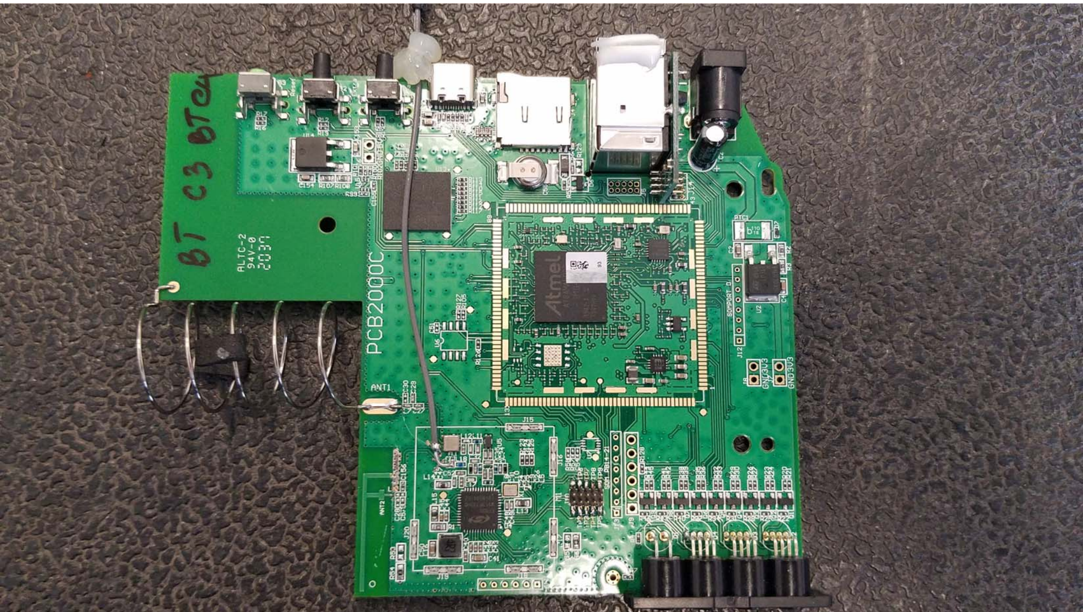
Top View of the PCB with Shield Removed - View #1
