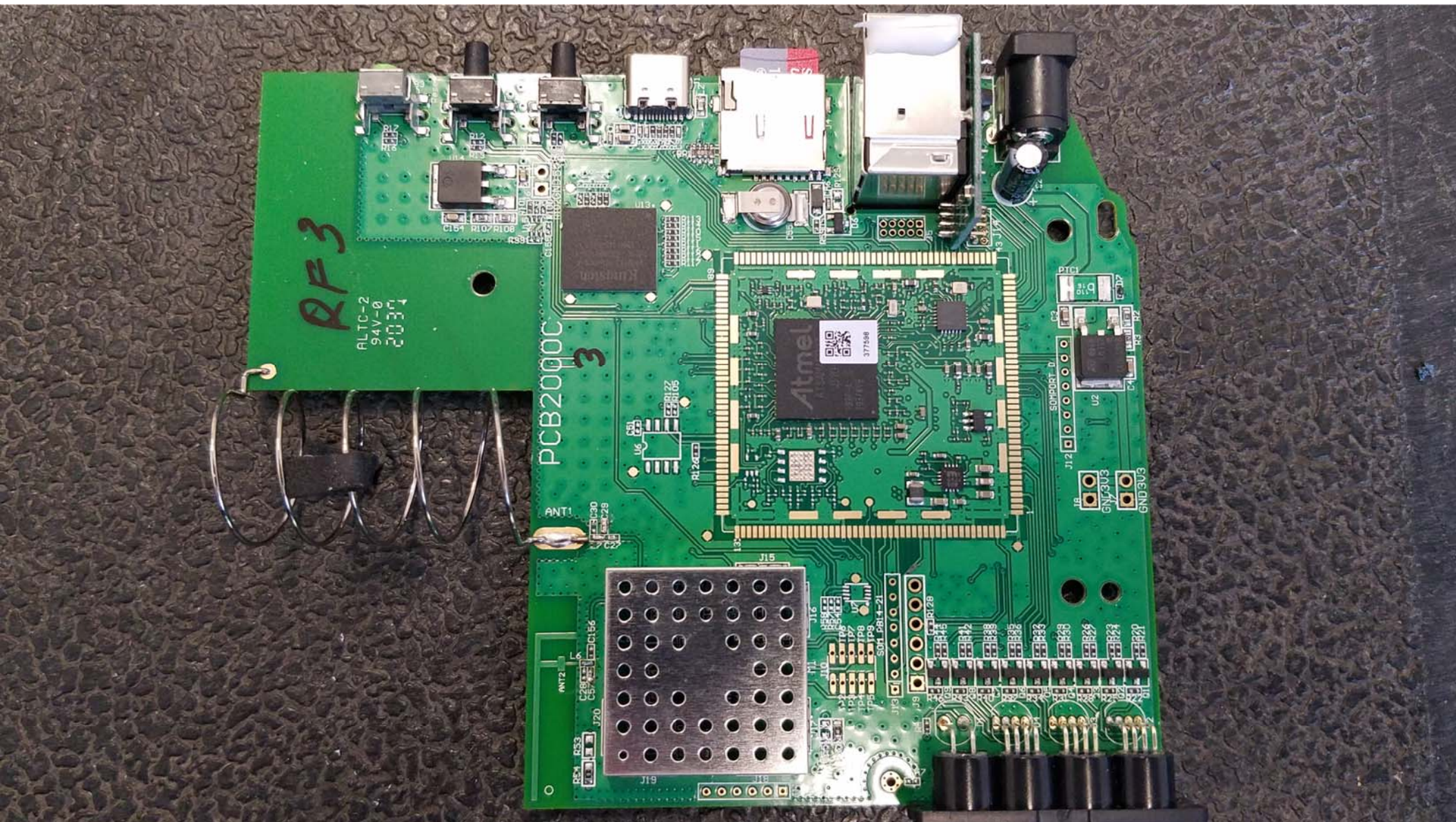
Top View of the PCB with Shield - View #1
