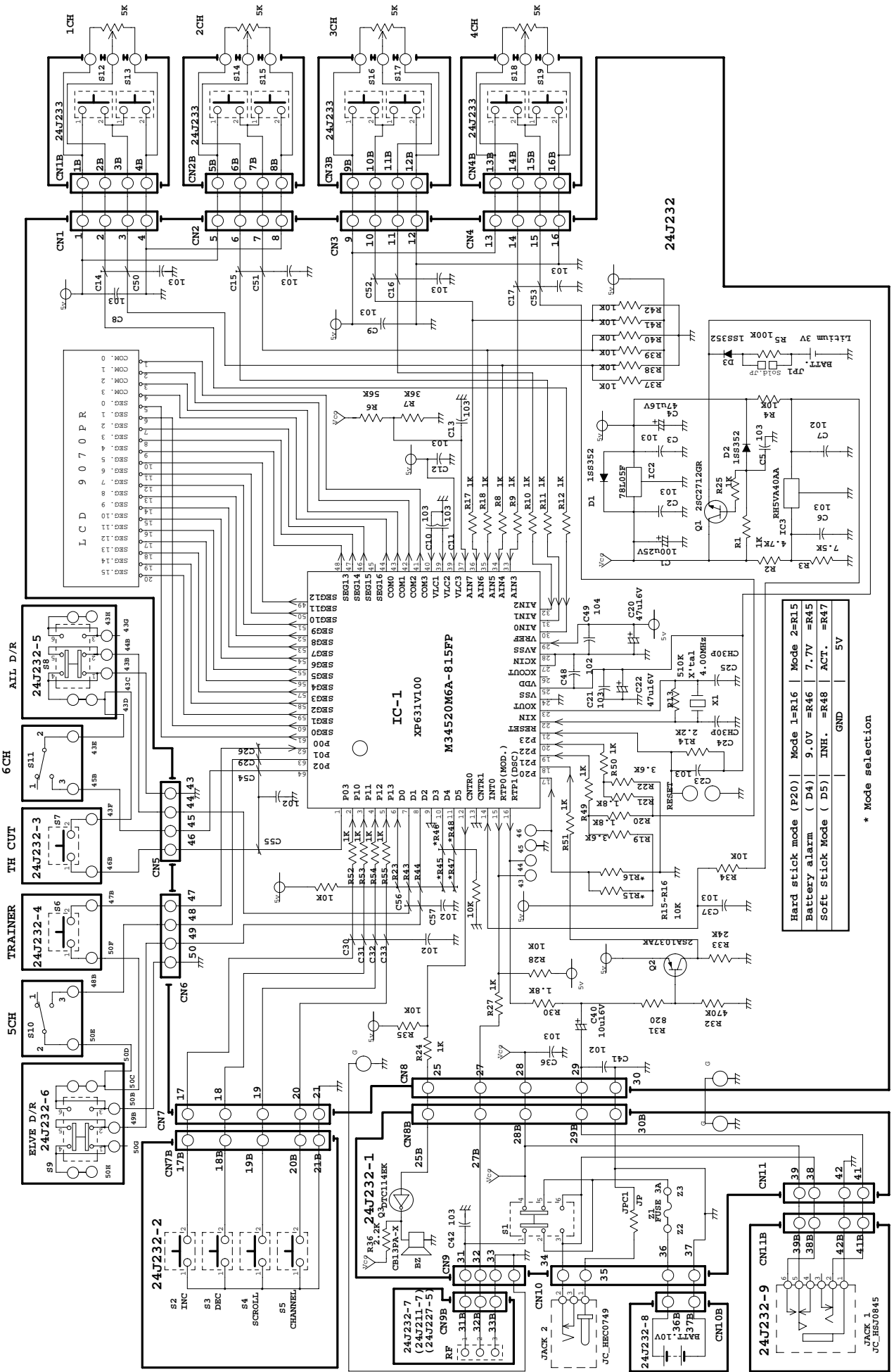
Figure 5.2.1.1. Transmitter Schematic Diagram
