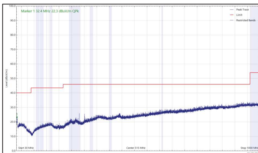
Figure 112 - U-NII-8 - 6995 MHz (CH209), HE20, SU, CDD, Core 0 + Core 1, 30 MHz to 1 GHz, Horizontal (Peak)
