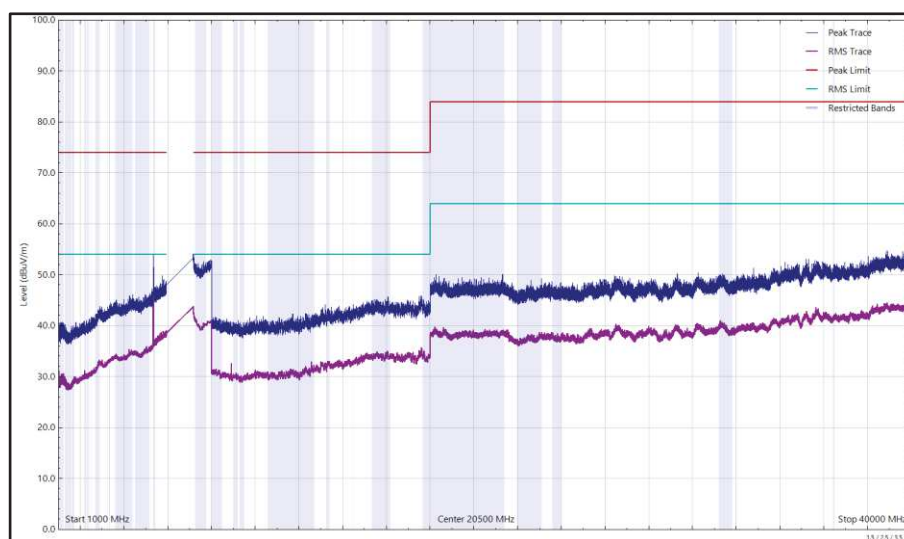
Figure 131 - U-NII-8 - 7115 MHz (CH233), HE20, SU, CDD, Core 0 + Core 1, 1 GHz to 40 GHz, Vertical
