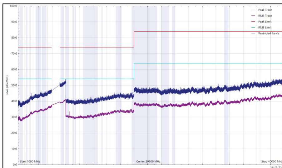
Figure 120 - U-NII-6 - 6435 MHz (CH97), HE20, SU, CDD, Core 0 + Core 1, 1 GHz to 40 GHz, Horizontal
