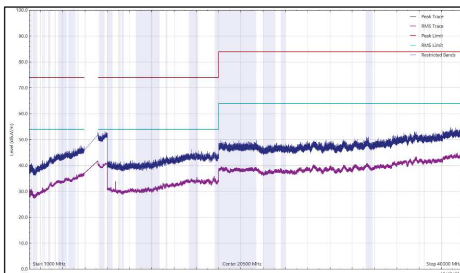
Figure 113 - U-NII-8 - 6995 MHz (CH209), HE20, SU, CDD, Core 0 + Core 1, 1 GHz to 40 GHz, Horizontal
