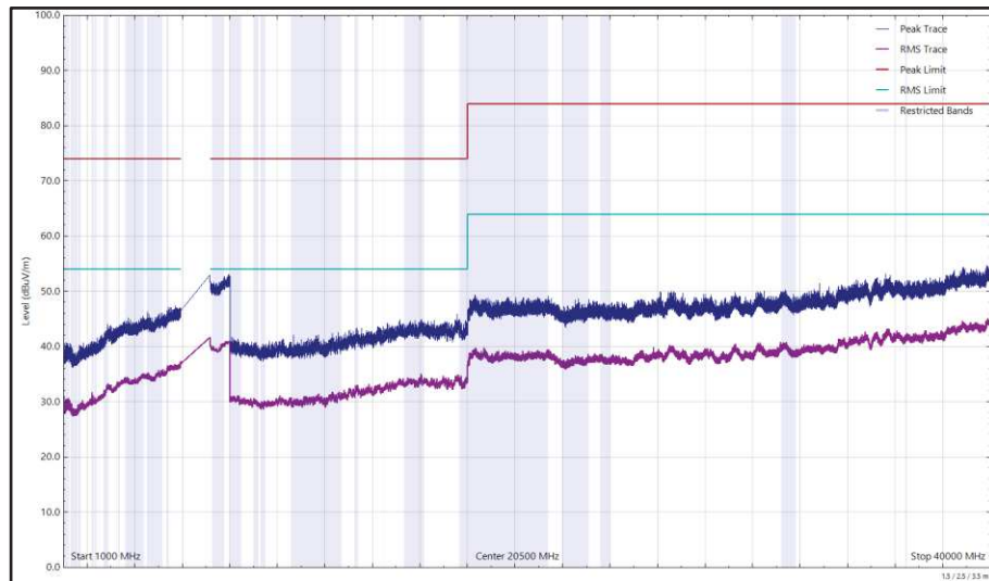
Figure 126 - U-NII-7 - 6855 MHz (CH181), HE20, SU, CDD, Core 0 + Core 1, 1 GHz to 40 GHz, Horizontal
