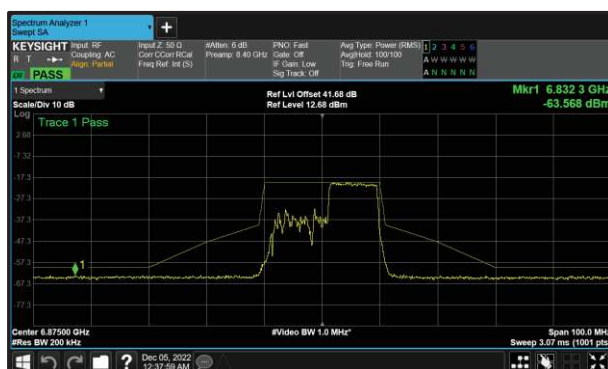
Figure 94 - B (Core 1) 802.11ax HE20 RU106 6875 MHz (CH185)
