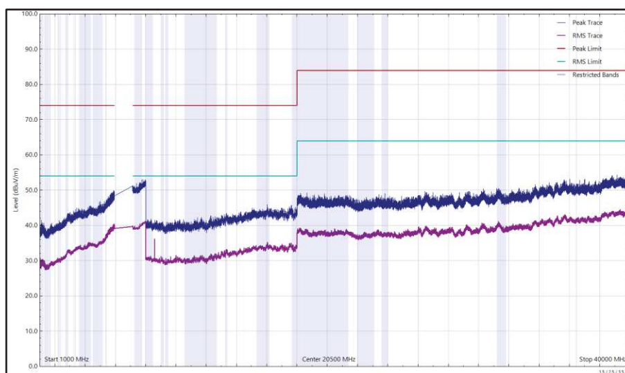
Figure 121 - U-NII-6 - 6435 MHz (CH97), HE20, SU, CDD, Core 0 + Core 1, 1 GHz to 40 GHz, Vertical
