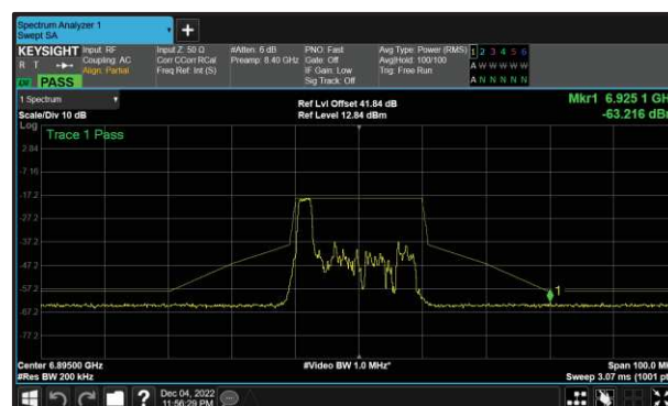
Figure 95 - B (Core 1) 802.11ax HE20 RU26 6895 MHz (CH189)
