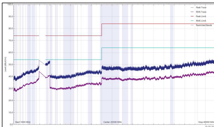
Figure 116 - U-NII-5 - 5955 MHz (CH1), HE20, SU, CDD, Core 0 + Core 1, 1 GHz to 40 GHz, Horizontal
