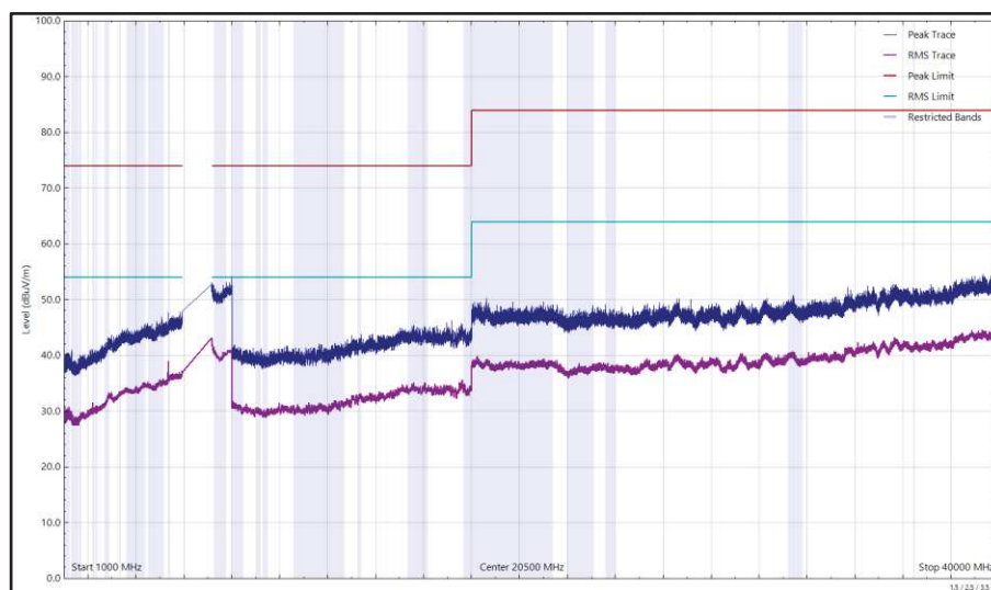
Figure 130 - U-NII-8 - 7115 MHz (CH233), HE20, SU, CDD, Core 0 + Core 1, 1 GHz to 40 GHz, Horizontal
