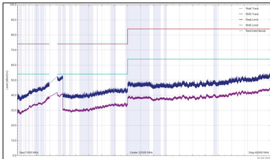
Figure 127 - U-NII-7 - 6855 MHz (CH181), HE20, SU, CDD, Core 0 + Core 1, 1 GHz to 40 GHz, Vertical
