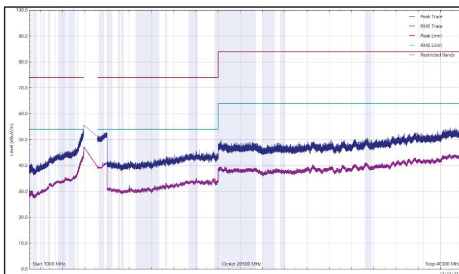
Figure 117 - U-NII-5 - 5955 MHz (CH1), HE20, SU, CDD, Core 0 + Core 1, 1 GHz to 40 GHz, Vertical
