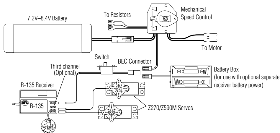
Figure A – Connections to BEC receiver with mechanical speed controller. Ni-Cd battery and speed controller are not included in the radio set.
