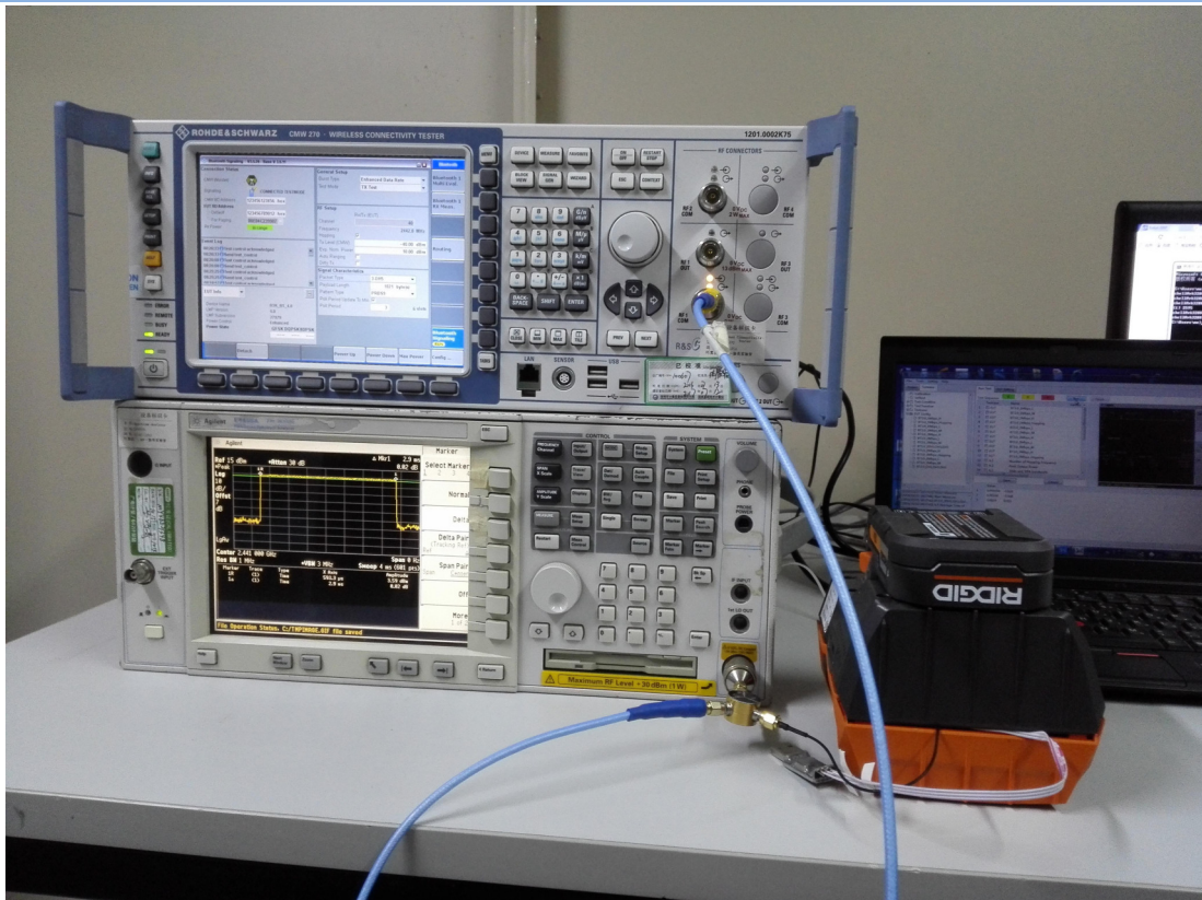
Conducted Test
