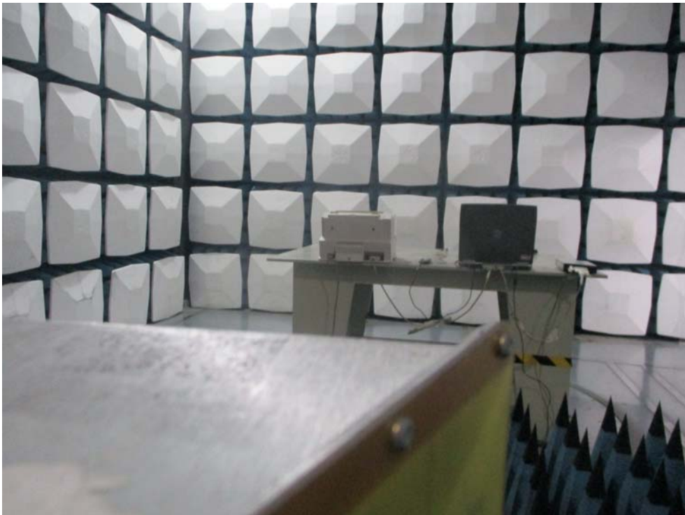
Radiated Emission Above 1GHz Side View
