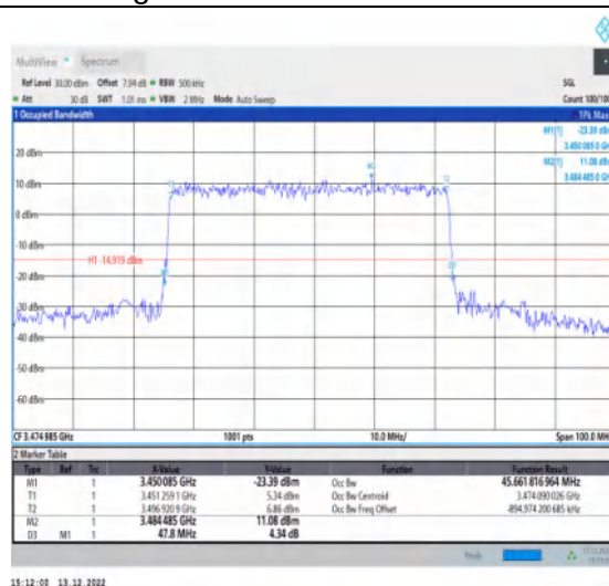
1-N77-3450-3550-30-50-L-3-DFT-16QAM-Outer_Full-128@0-Ant1-45.662-47.800-≤50-PASS
