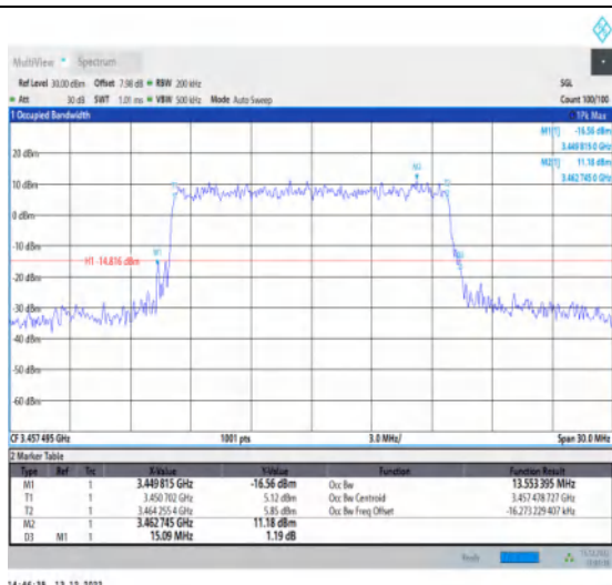
1-N77-3450-3550-30-15-L-6-CP-QPSK-Outer_Full-38@0-Ant1-13.553-15.090-≤15-PASS
