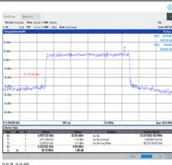
1-N77-3450-3550-30-60-M-8-CP-64QAM-Out_1 162@0-Ant1-57.676-59.760≤60-PASS
