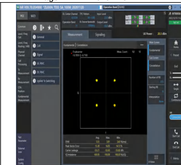
1-N77-3450-3550-30-100-M-6-CP-QPSK-Outer_Full-273@0-Ant1-see graph-PASS
