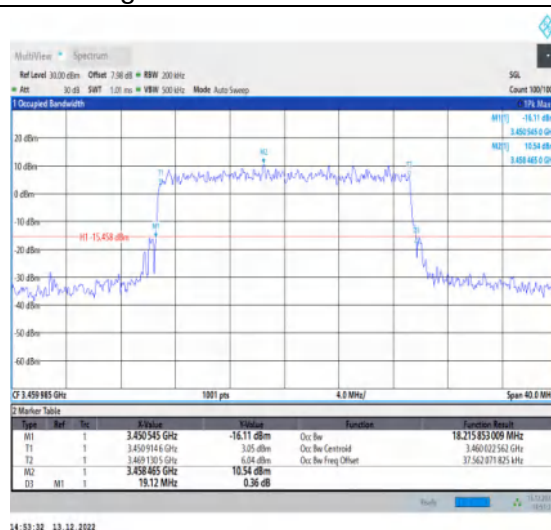
1-N77-3450-3550-30-20-L-8-CP-64QAM-Outer_Full-51@0-Ant1-18.216-19.120-≤20-PASS
