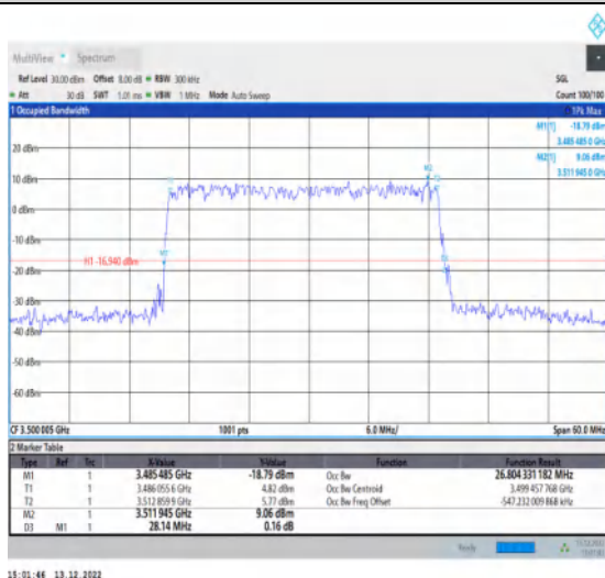
1-N77-3450-3550-30-30-M-5-DFT-256QAM-Outer_F ull-75@0-Ant1-26.804-28.140-≤30-PASS
