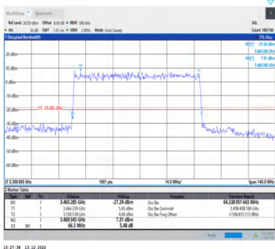
1-N77-3450-3550-30-70-M-5-DFT-256QAM-Outer_F ull-180@0-Ant1-64.339-66.500-≤70-PASS
