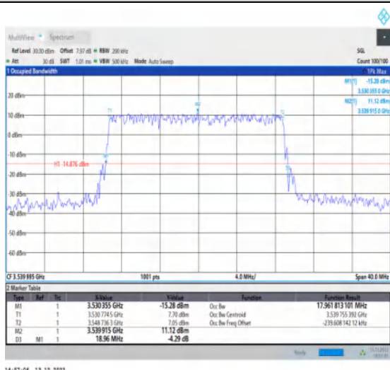
1-N77-3450-3550-30-20-H-3-DFT-16QAM-Outer_Full-50@0-Ant1-17.962-18.960-≤20-PASS
