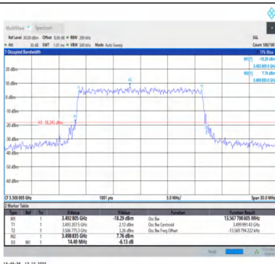
1-N77-3450-3550-30-15-M-9-CP-256QAM-Outer_Full-I-38@0-Ant1-13.568-14.490-≤15-PASS
