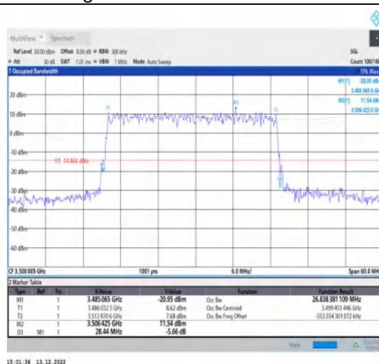
1-N77-3450-3550-30-30-M-4-DFT-64QAM-Outer_Ful I-75@0-Ant1-26.838-28.440-≤30-PASS
