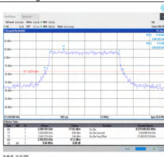
1-N77-3450-3550-30-10-H-8-CP-64QAM-Outer_Full-24@0-Ant1-8.58-9.640-≤10-PASS
