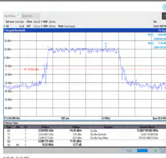
1-N77-3450-3550-30-15-H-3-DFT-16QAM-Outer_Full-36@0-Ant1-12.893-14.550-≤15-PASS
