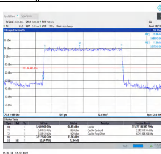
1-N77-3450-3550-30-60-H-2-DFT-PI2BPSK-Outer_Full-162@0-Ant1-57.874-60.240-≤60-PASS
