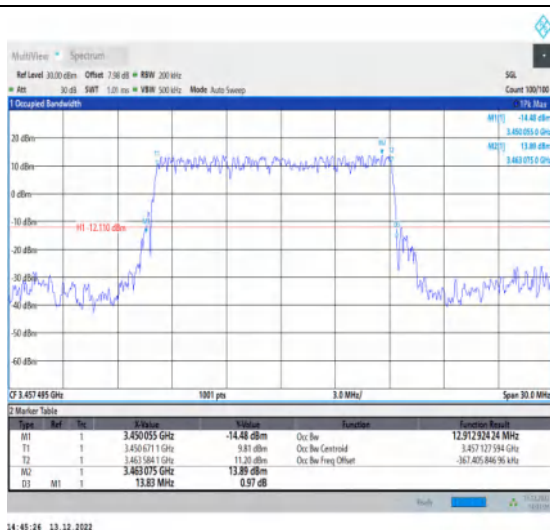
1-N77-3450-3550-30-15-L-2-DFT-PI2BPSK-Outer_Full-36@0-Ant1-12.913-13.830-≤15-PASS
