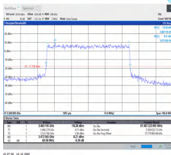
1-N77-3450-3550-30-70-M-6-CP-QPSK-Outer_Full-1 89@0-Ant1-67.487-69.580-≤70-PASS
