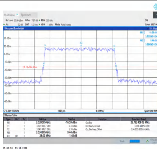
1-N77-3450-3550-30-30-H-5-DFT-256QAM-Outer_Full-75@0-Ant1-26.732-28.020-≤30-PASS
