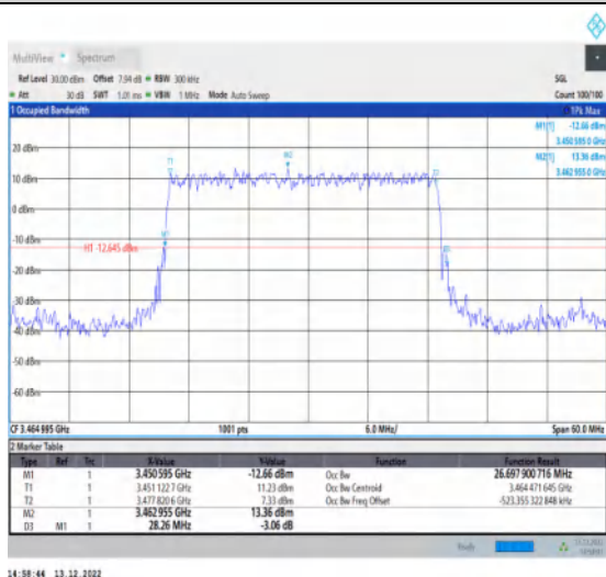
1-N77-3450-3550-30-30-L-2-DFT-PI2BPSK-Outer_Full-75@0-Ant1-26.698-28.260-≤30-PASS
