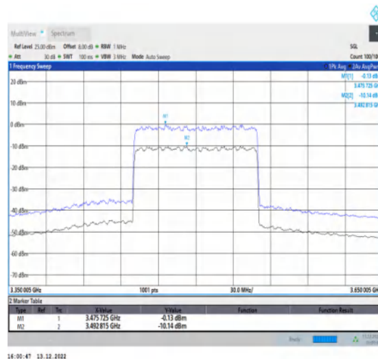
1-N77-3450-3550-30-100-M-2-CP-256QAM-Outer_Full-273@0-Ant1-10.01-100%-0.00-10.01-PASS-≤13
