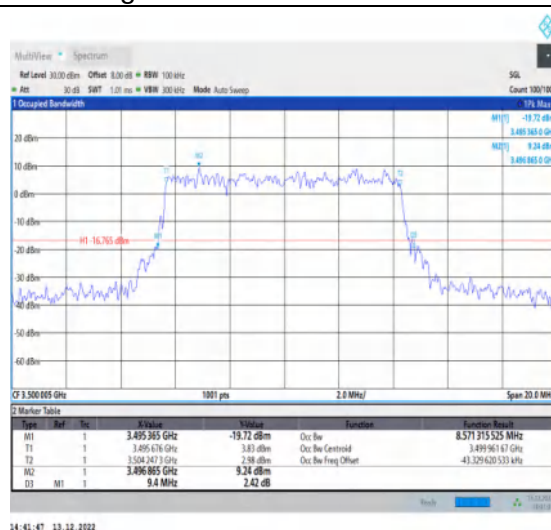
1-N77-3450-3550-30-10-M-5-DFT-256QAM-Out-Full-I-24@0-Ant1-8.571-9.400-≤10-PASS
