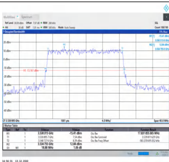
1-N77-3450-3550-30-20-H-1-DFT-QPSK-Outer_Full-50@0-Ant1-17.832-18.880-≤20-PASS
