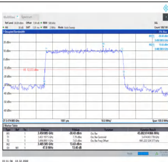
1-N77-3450-3550-30-50-L-2-DFT-PI2BPSK-Outer_Full-128@0-Ant1-45.693-47.800-≤50-PASS
