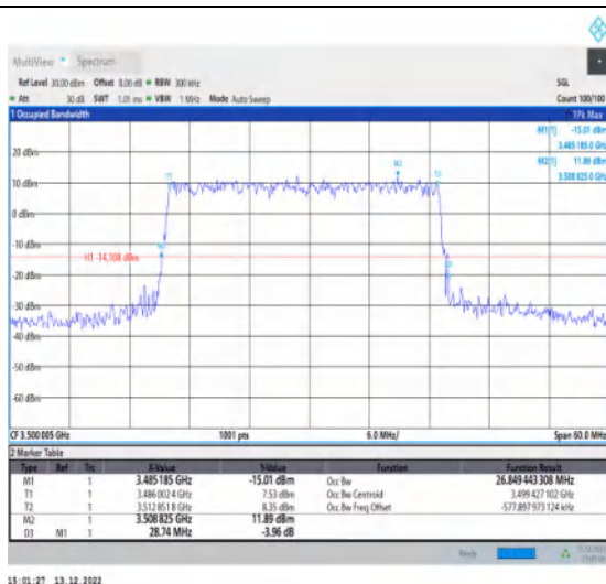
1-N77-3450-3550-30-30-M-3-DFT-16QAM-Outer_Ful I-75@0-Ant1-26.849-28.740-≤30-PASS
