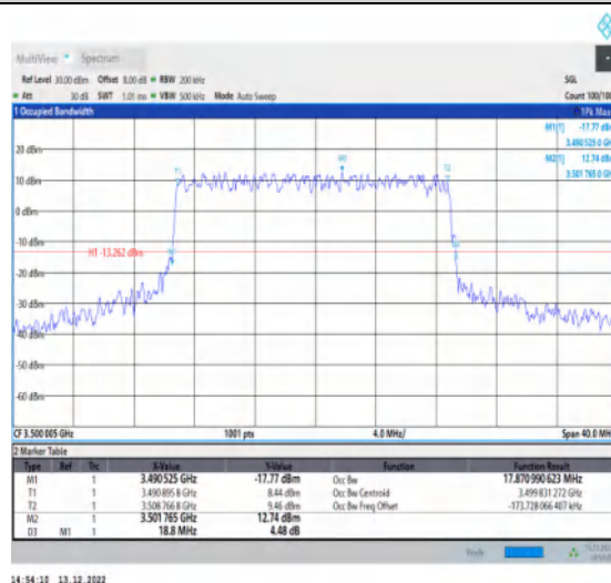
1-N77-3450-3550-30-20-M-1-DFT-QPSK-Outer_Full-50@0-Ant1-17.871-18.800-≤20-PASS
