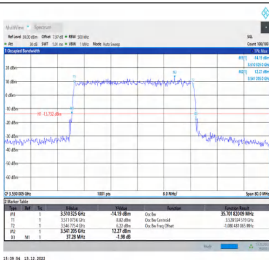
1-N77-3450-3550-30-40-H-3-DFT-16QAM-Outer_Ful I-100@0-Ant1-35.702-37.280-≤40-PASS
