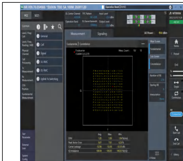
1-N77-3450-3550-30-100-M-5-DFT-256QAM-Outer_Full-270@0-Ant1-see graph-PASS
