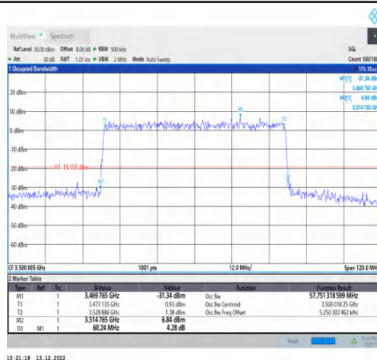
1-N77-3450-3550-30-60-M-9-CP-256QAM-Out_1 162@0-Ant1-57.751-60.240≤60-PASS
