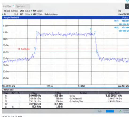
1-N77-3450-3550-30-20-M-8-CP-64QAM-Outter_Full-51@0-Ant1-18.221-19.280-≤20-PASS
