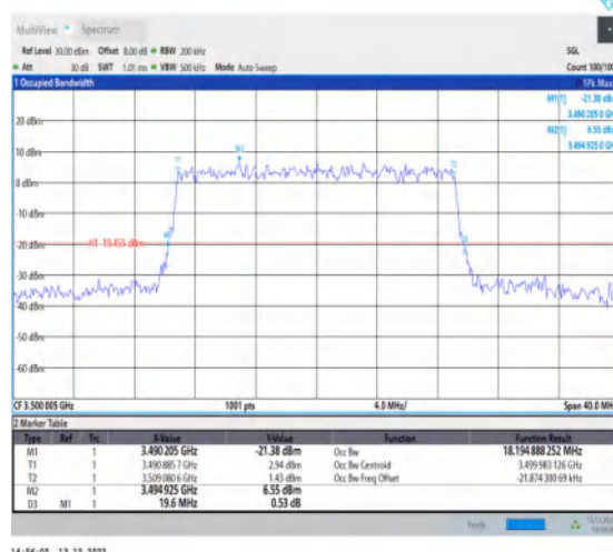
1-N77-3450-3550-30-20-M-9-CP-256QAM-Outter_Fu II-51@0-Ant1-18.195-19.600-≤20-PASS
