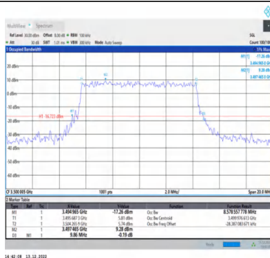
1-N77-3450-3550-30-10-M-7-CP-16QAM-Out-Full-I-24@0-Ant1-8.579-9.860-≤10-PASS
