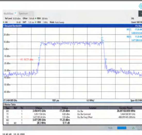
1-N77-3450-3550-30-30-L-3-DFT-16QAM-Outer_Full-75@0-Ant1-26.698-28.500-≤30-PASS
