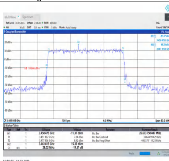
1-N77-3450-3550-30-30-L-1-DFT-QPSK-Outer_Full-75@0-Ant1-26.674-28.020-≤30-PASS
