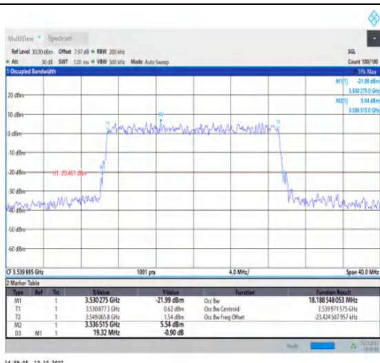
1-N77-3450-3550-30-20-H-9-CP-256QAM-Outer_Ful I-51@0-Ant1-18.189-19.320-≤20-PASS
