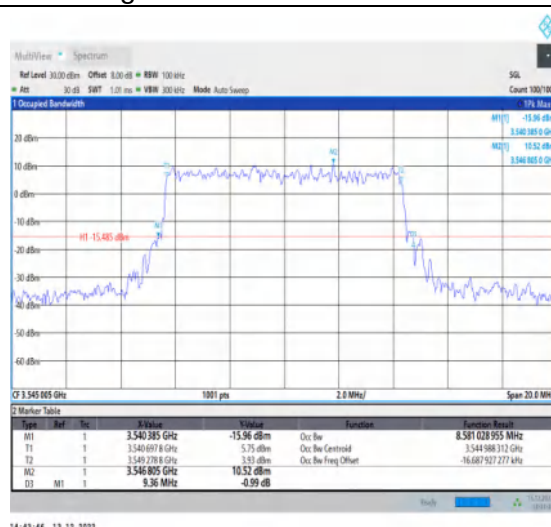
1-N77-3450-3550-30-10-H-4-DFT-64QAM-Outer_Ful I-24@0-Ant1-8.581-9.360-≤10-PASS
