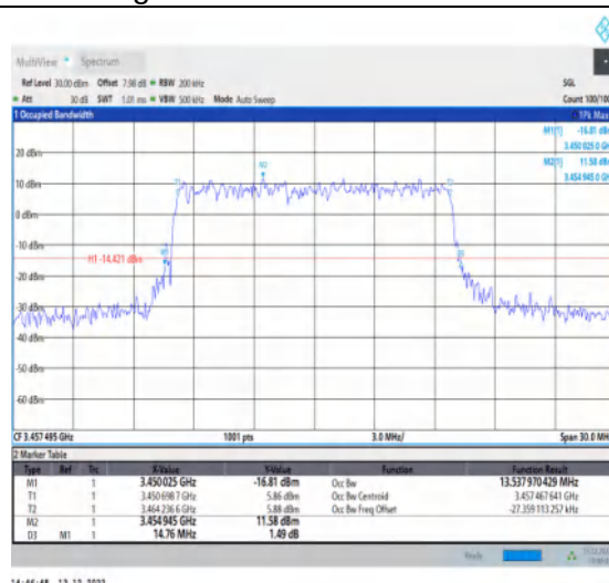
1-N77-3450-3550-30-15-L-7-CP-16QAM-Outer_Full-38@0-Ant1-13.538-14.760-≤15-PASS
