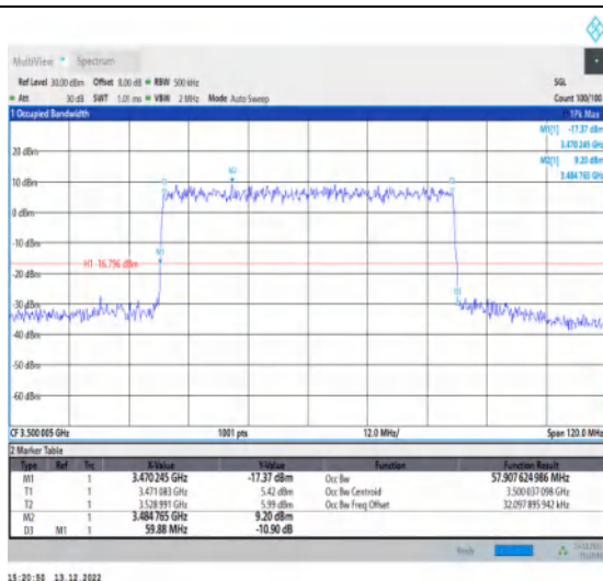
1-N77-3450-3550-30-60-M-6-CP-QPSK-Out_1 62@0-Ant1-57.908-59.880≤60-PASS
