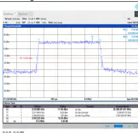
1-N77-3450-3550-30-40-H-4-DFT-64QAM-Outer_Ful I-100@0-Ant1-35.786-37.600-≤40-PASS
