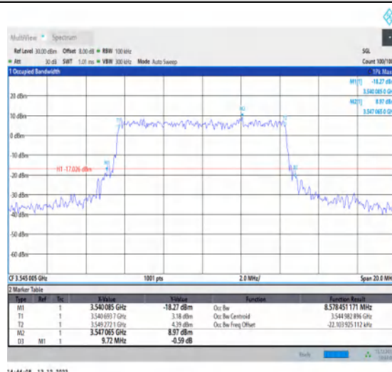
1-N77-3450-3550-30-10-H-6-CP-QPSK-Outer_Full-24@0-Ant1-8.578-9.720-≤10-PASS
