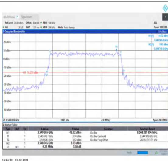
1-N77-3450-3550-30-10-H-7-CP-16QAM-Outer_Full-24@0-Ant1-8.568-9.240-≤10-PASS
