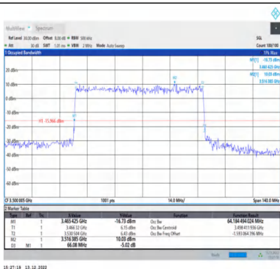
1-N77-3450-3550-30-70-M-3-DFT-16QAM-Outer_Ful I-180@0-Ant1-64.184-66.080-≤70-PASS
