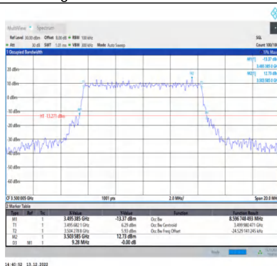
1-N77-3450-3550-30-10-M-1-DFT-QPSK-Outer_Full- 24@0-Ant1-8.597-9.280-≤10-PASS
