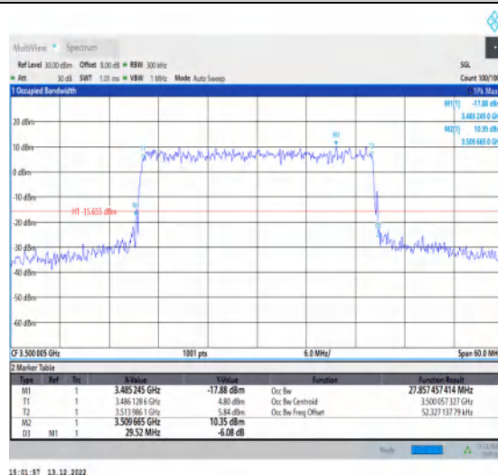
1-N77-3450-3550-30-30-M-6-CP-QPSK-Outer_Full-7 8@0-Ant1-27.857-29.520-≤30-PASS
