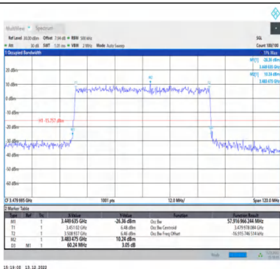
1-N77-3450-3550-30-60-L-7-CP-16QAM-Outer_Full-162@0-Ant1-57.917-60.240-≤60-PASS
