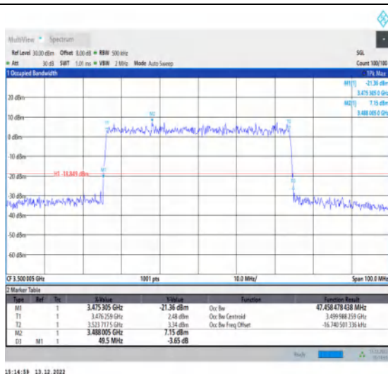
1-N77-3450-3550-30-50-M-9-CP-256QAM-Outer_Ful I-133@0-Ant1-47.458-49.500-≤50-PASS
