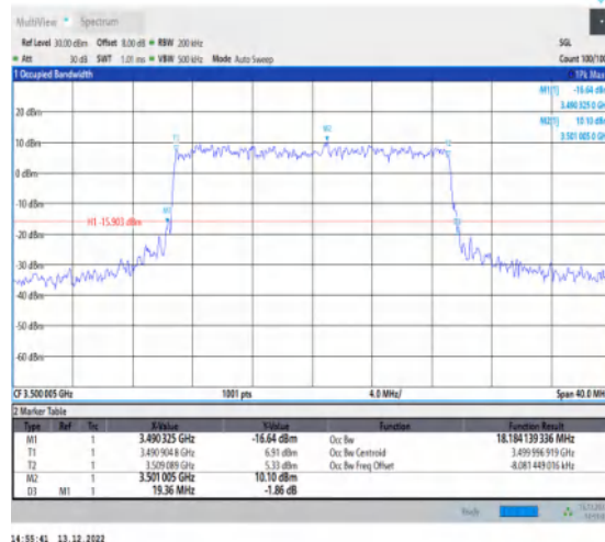
1-N77-3450-3550-30-20-M-7-CP-16QAM-Outter_Full -51@0-Ant1-18.184-19.360-≤20-PASS
