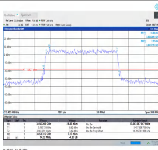
1-N77-3450-3550-30-15-L-9-CP-256QAM-Outer_Full-38@0-Ant1-13.563-14.520-≤15-PASS
