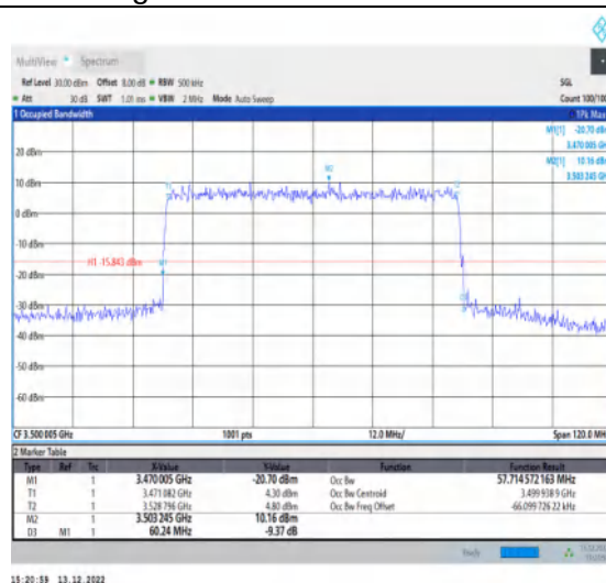
1-N77-3450-3550-30-60-M-7-CP-16QAM-Out_1 -162@0-Ant1-57.715-60.240≤60-PASS
