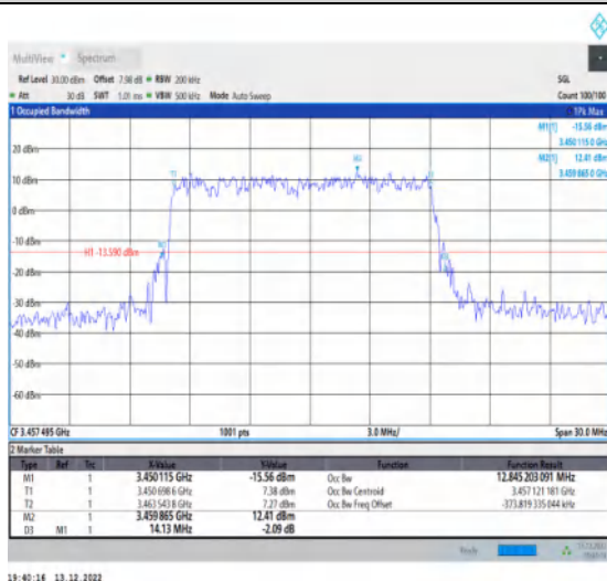
1-N77-3450-3550-30-15-L-4-DFT-64QAM-Outer_Full-36@0-Ant1-12.845-14.130-≤15-PASS
