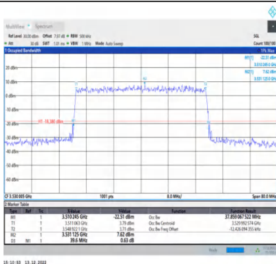
1-N77-3450-3550-30-40-H-9-CP-256QAM-Outer_Ful-I-106@0-Ant1-37.859-39.600-≤40-PASS
