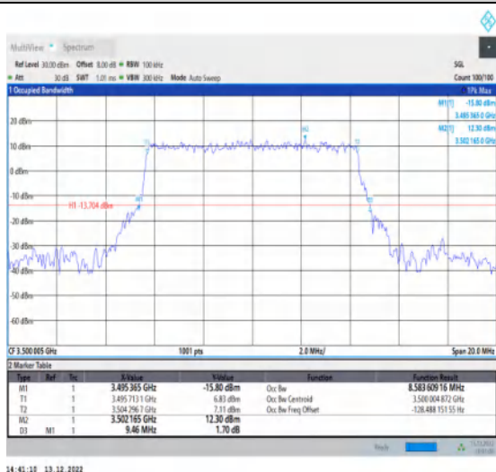
1-N77-3450-3550-30-10-M-2-DFT-PI2BPSK-Outer_F ull-24@0-Ant1-8.584-9.460-≤10-PASS
