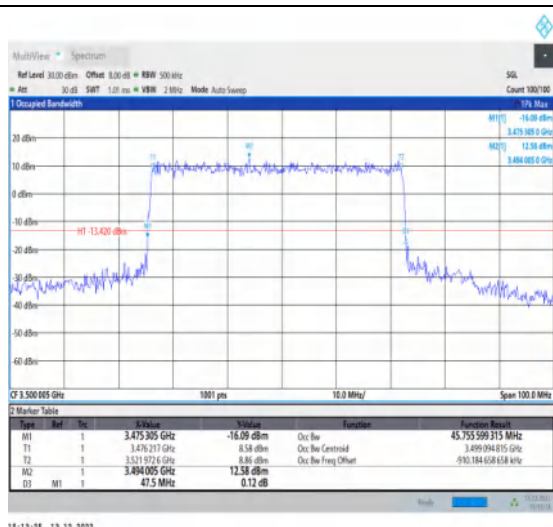
1-N77-3450-3550-30-50-M-1-DFT-QPSK-Outer_Full-128@0-Ant1-45.756-47.500-≤50-PASS
