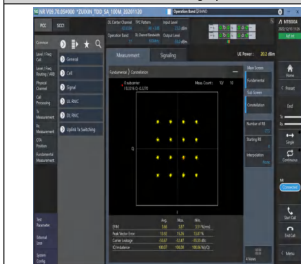
1-N77-3450-3550-30-100-M-7-CP-16QAM-Outer_Full-273@0-Ant1-see graph-PASS
