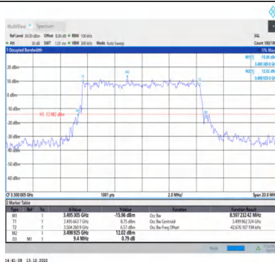
1-N77-3450-3550-30-10-M-3-DFT-16QAM-Outer_Ful l-24@0-Ant1-8.597-9.400-≤10-PASS
