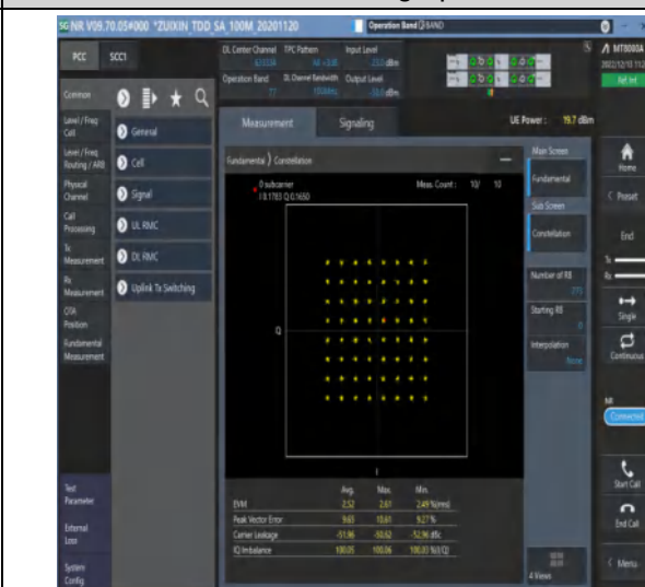
1-N77-3450-3550-30-100-M-8-CP-64QAM-Outer_Full-273@0-Ant1-see graph-PASS
