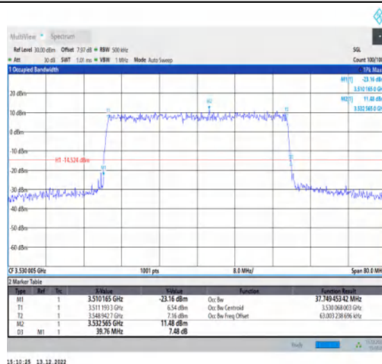
1-N77-3450-3550-30-40-H-6-CP-QPSK-Outer_Full-1 06@0-Ant1-37.749-39.760-≤40-PASS
