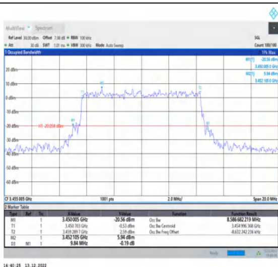
1-N77-3450-3550-30-10-L-9-CP-256QAM-Outer_Full -24@0-Ant1-8.587-9.840-≤10-PASS
