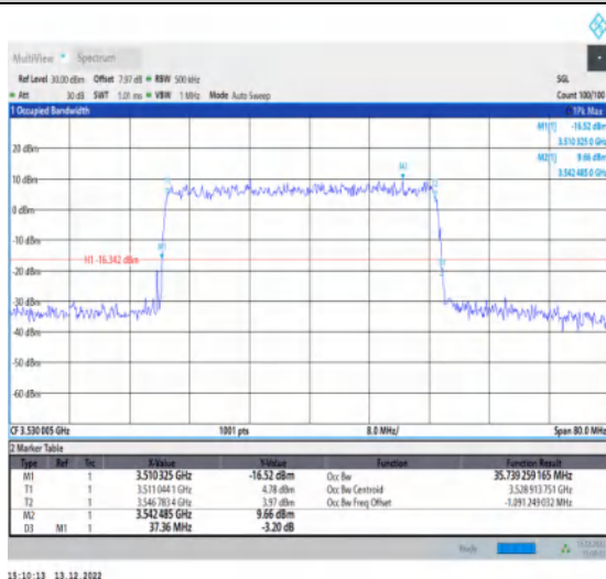
1-N77-3450-3550-30-40-H-5-DFT-256QAM-Outer_F ull-100@0-Ant1-35.739-37.360-≤40-PASS
