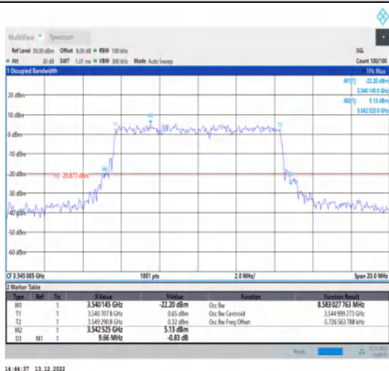
1-N77-3450-3550-30-10-H-9-CP-256QAM-Outer_Ful-I-24@0-Ant1-8.583-9.660-≤10-PASS
