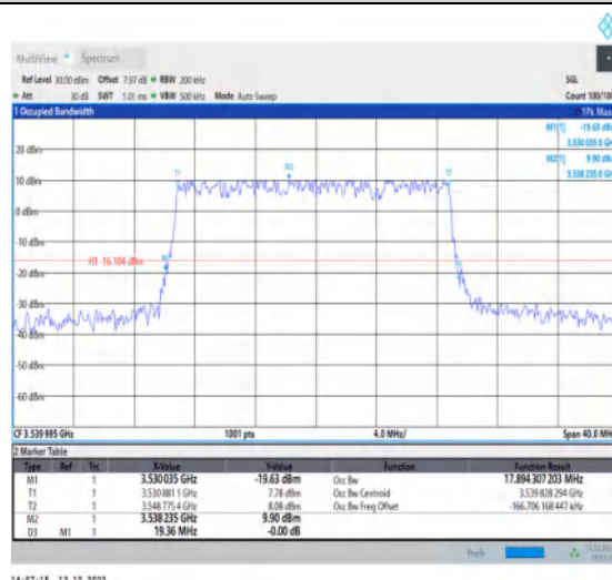
1-N77-3450-3550-30-20-H-4-DFT-64QAM-Outer_Full-50@0-Ant1-17.894-19.360-≤20-PASS
