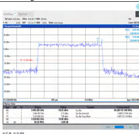
1-N77-3450-3550-30-70-M-4-DFT-64QAM-Outer_Ful I-180@0-Ant1-64.26-66.360-≤70-PASS
