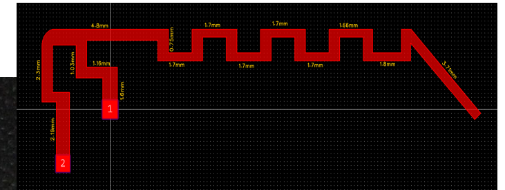
BT Antenna
