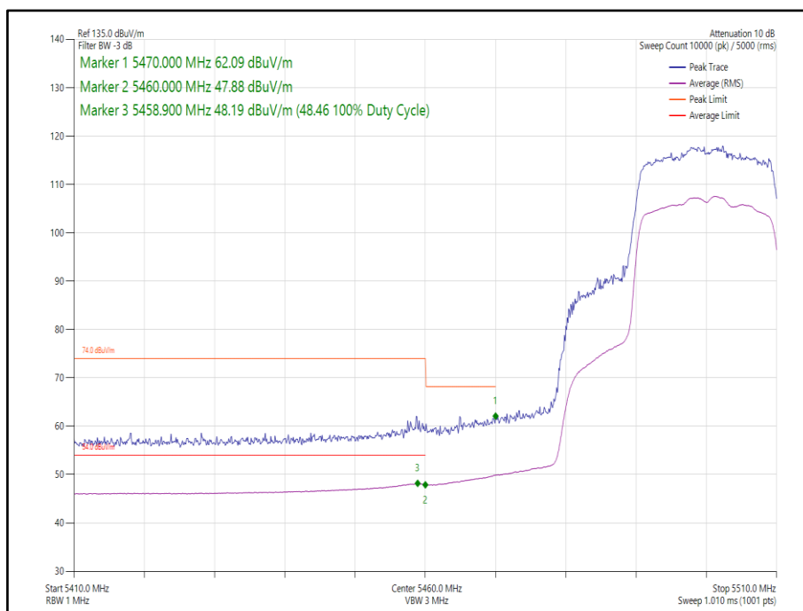
Figure 29 - 802.11ax HE20 SDM, Cores 0-1, SU - 5500 MHz, Band Edge Frequency 5460 MHz
