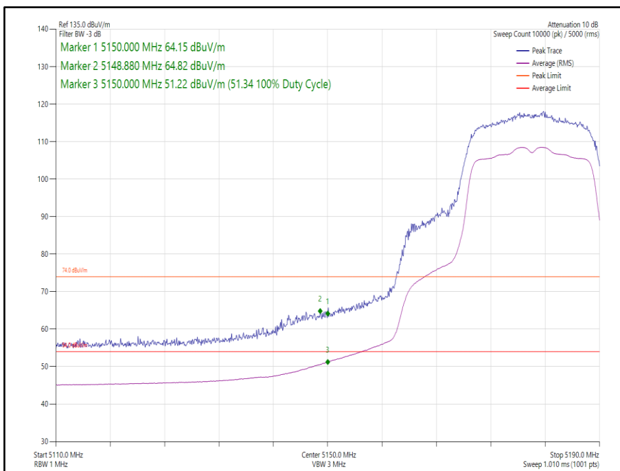
Figure 2 - 802.11n HT20, Core 1 - 5180 MHz, Band Edge Frequency 5150 MHz
