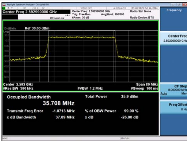
NTNV-n41-PC2-30-40-M-DFT-16QAM-Outer_Full-Ant1-PA SS
