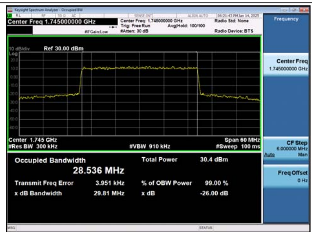
NTNV-n66-PC3-15-30-M-DFT-QPSK-Outet_Full-Ant1-PAS S
