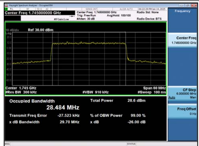
NTNV-n66-PC3-15-30-M-DFT-64QAM-Outet_Full-Ant1-PA SS
