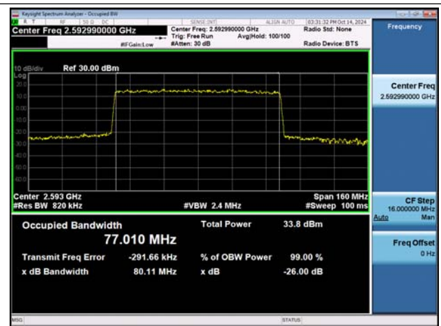
NTV-n41-PC2-30-80-M-DFT-QPSK-Outer_Full-Ant1-PAS S
