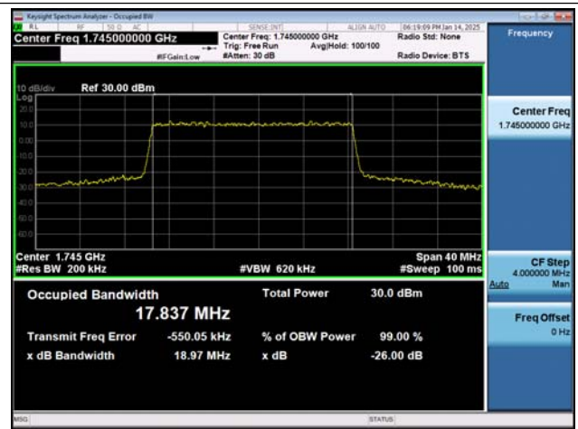
NTVN-n66-PC3-15-20-M-DFT-QPSK-Outer_Full-Ant1-PASS S
