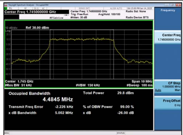
NTNV-n66-PC3-15-5-M-DFT-BPSK-Outter_Full-Ant1-PASS
