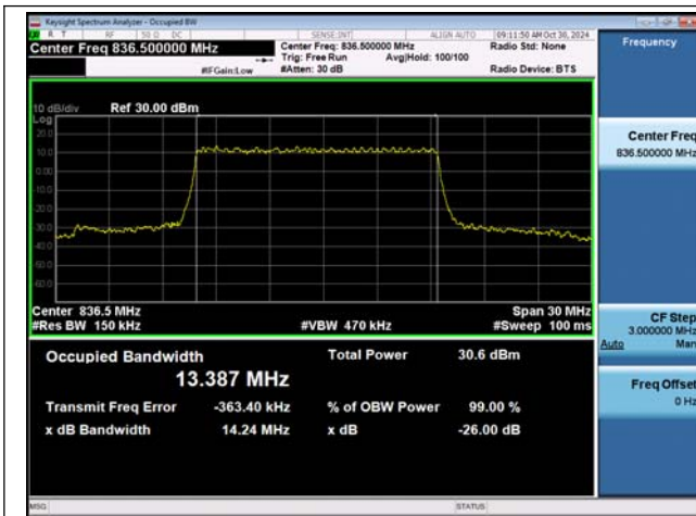
NTVN-n5-PC3-15-15-M-DFT-BPSK-Outer_Full-Ant1-PASS
