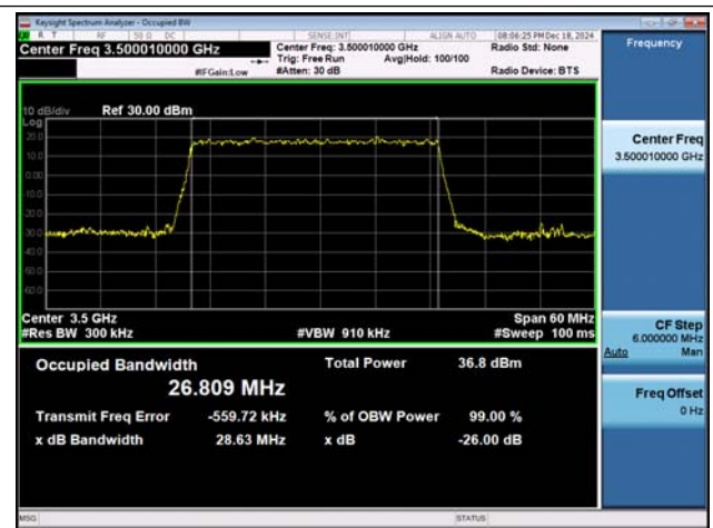
NTNV-n78(3450-3550)-PC2-30-30-M-DFT-BPSK-Outter_Full-Ant1-PASS
