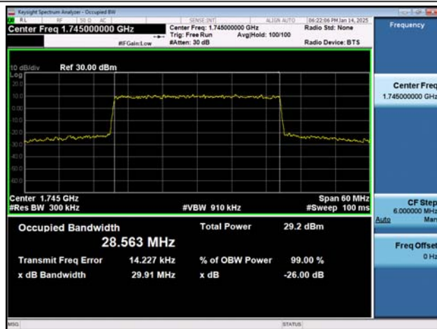
NTNV-n66-PC3-15-30-M-DFT-16QAM-Outet_Full-Ant1-PA SS
