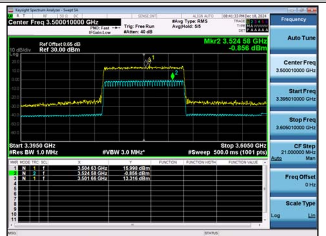
NTNT-n78(3450-3550)-PC2-30-70-M-CP-256QAM-Outer_Full-Ant1-PASS
