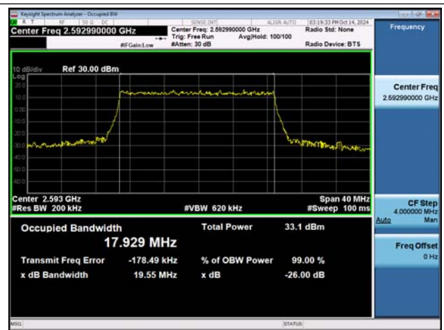
NTNV-n41-PC2-30-20-M-DFT-QPSK-Outer_Full-Ant1-PAS S
