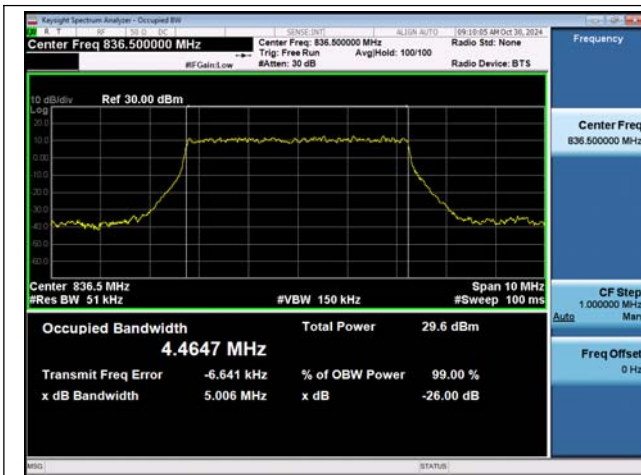
NTVN-n5-PC3-15-5-M-DFT-BPSK-Outet_Full-Ant1-PASS
