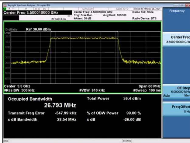
NTNV-n78(3450-3550)-PC2-30-30-M-DFT-QPSK-Outter_Full-Ant1-PASS
