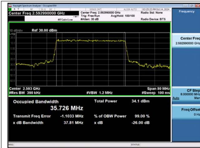
NTNV-n41-PC2-30-40-M-DFT-BPSK-Outer_Full-Ant1-PASS
