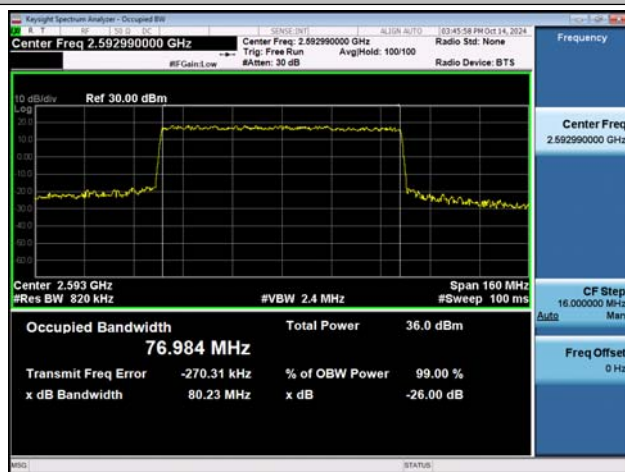
NTV-n41-PC2-30-80-M-DFT-16QAM-Outer_Full-Ant1-PA SS
