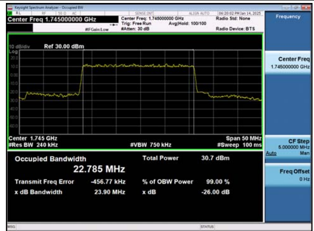
NTVN-n66-PC3-15-25-M-DFT-BPSK-Outer_Full-Ant1-PASS
