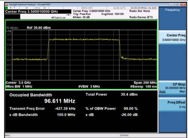
NTNV-n77(3450-3550)-PC3-30-100-M-DFT-QPSK-Outter_Full-Ant1-PASS
