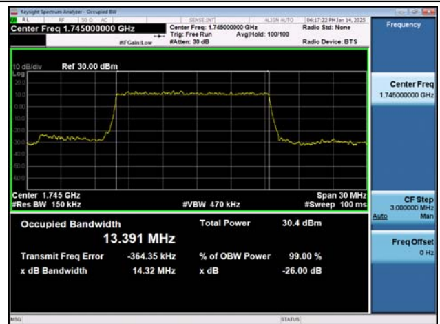
NTVN-n66-PC3-15-10-M-DFT-QPSK-Outer_Full-Ant1-PASS S
