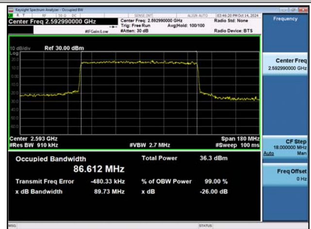
NTV-n41-PC2-30-90-M-DFT-16QAM-Outer_Full-Ant1-PA SS
