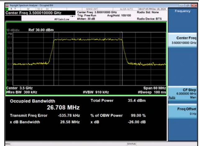
NTNV-n78(3450-3550)-PC2-30-30-M-DFT-16QAM-Outter_Full-Ant1-PASS
