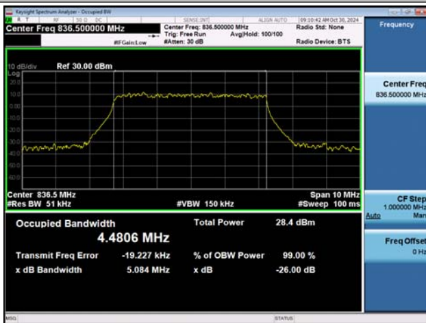
NTVN-n5-PC3-15-5-M-DFT-16QAM-Outet_Full-Ant1-PASS
