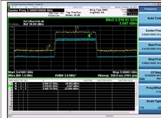
NTNT-n78(3450-3550)-PC2-30-60-M-DFT-256QAM-Outer_Full-Ant1-PASS
